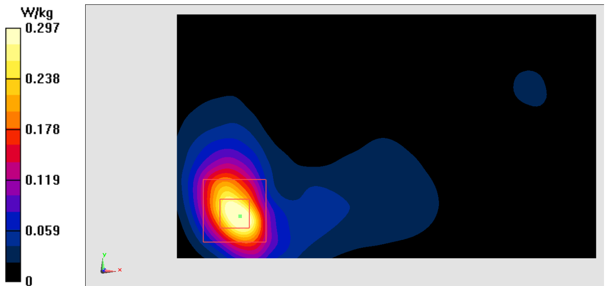
Fig.I.2 2450 MHz
