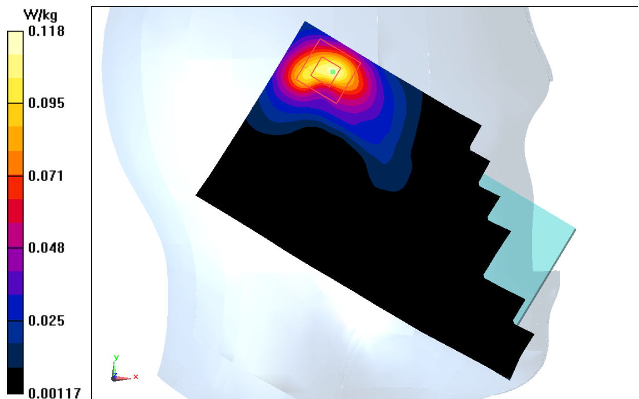
Fig.I.1 2450 MHz
