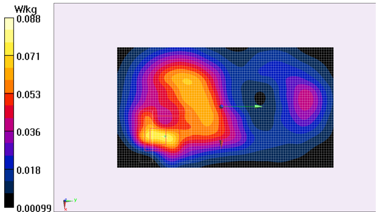
Fig.10 2450 MHz CH11
