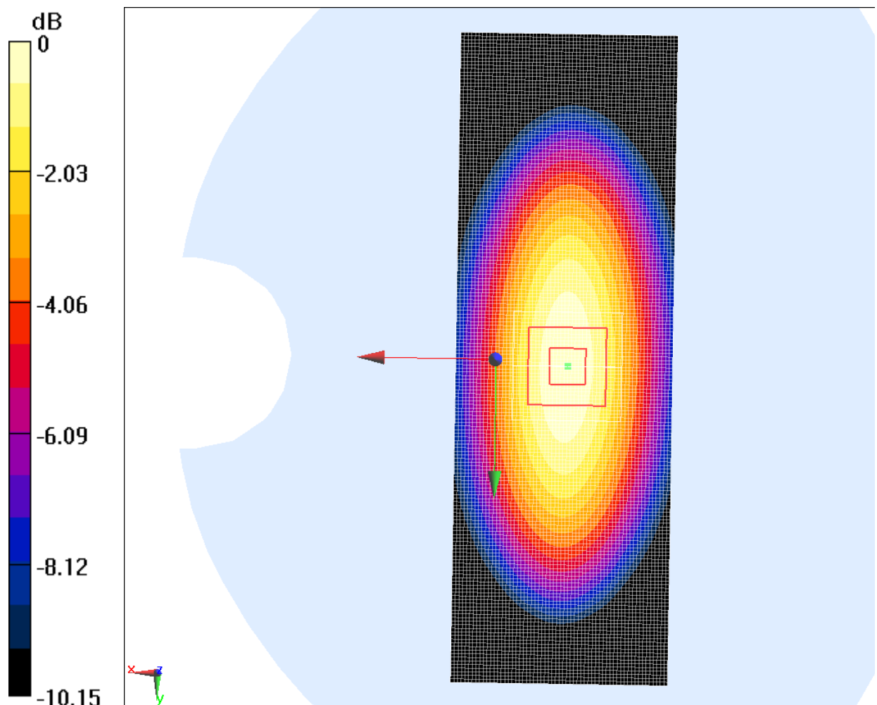
Fig.B.2 validation 835MHz 250mW
