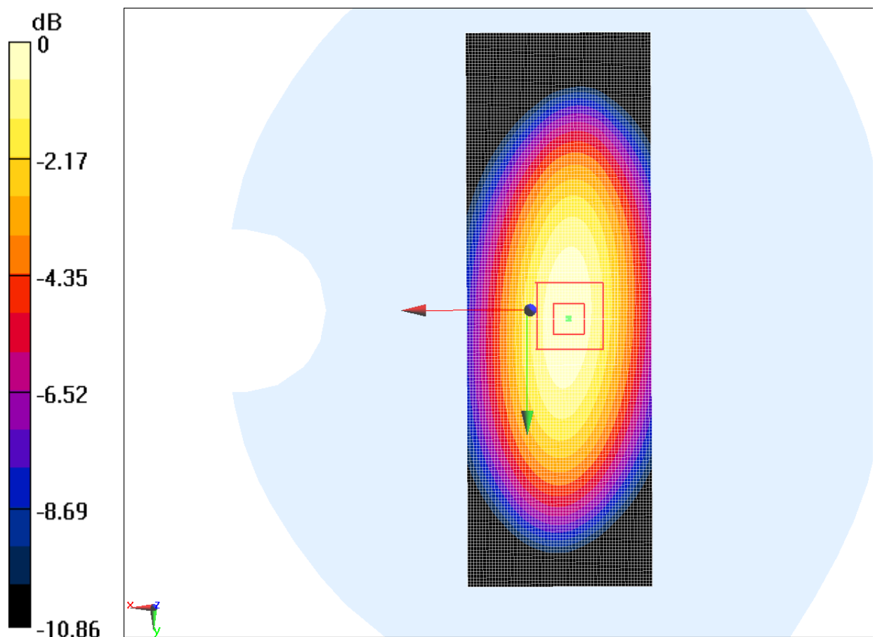
Fig.B.1 validation 835MHz 250mW
