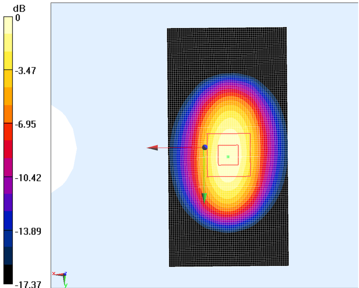
Fig.B.4 validation 1900MHz 250mW
