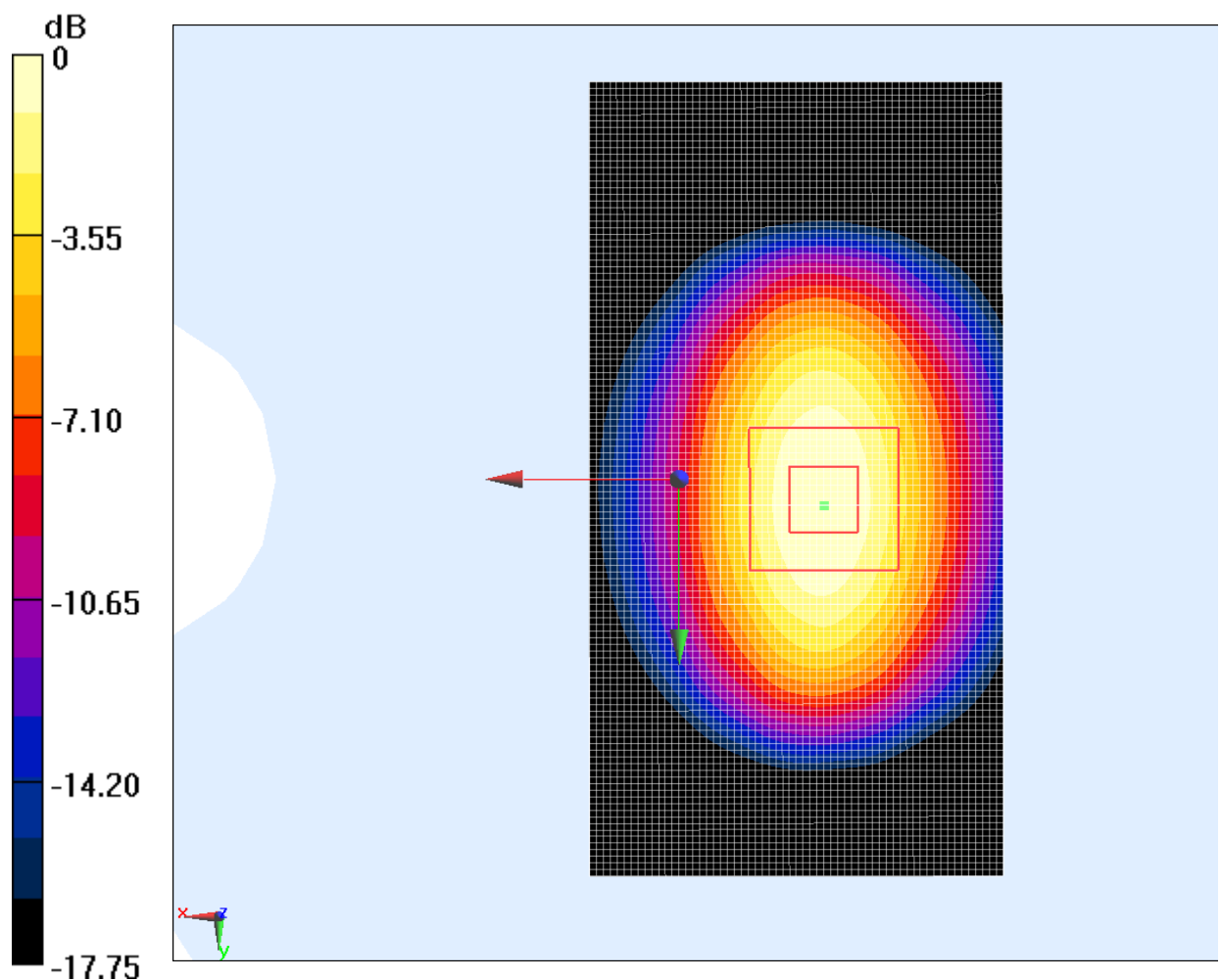
Fig.B.3 validation 1900MHz 250mW
