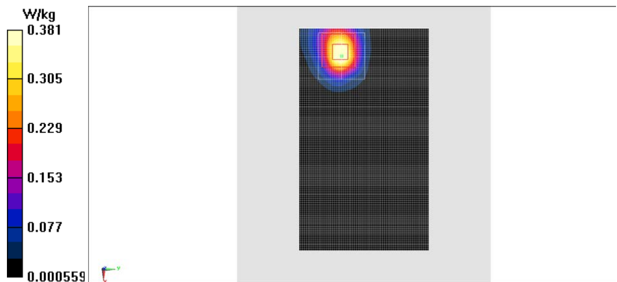
Fig.8 2450 MHz CH6
