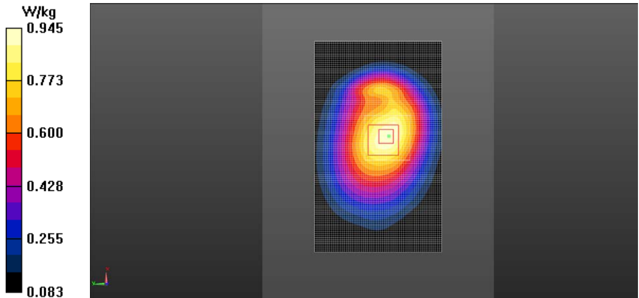
Fig.6 WCDMA 850 CH4233
