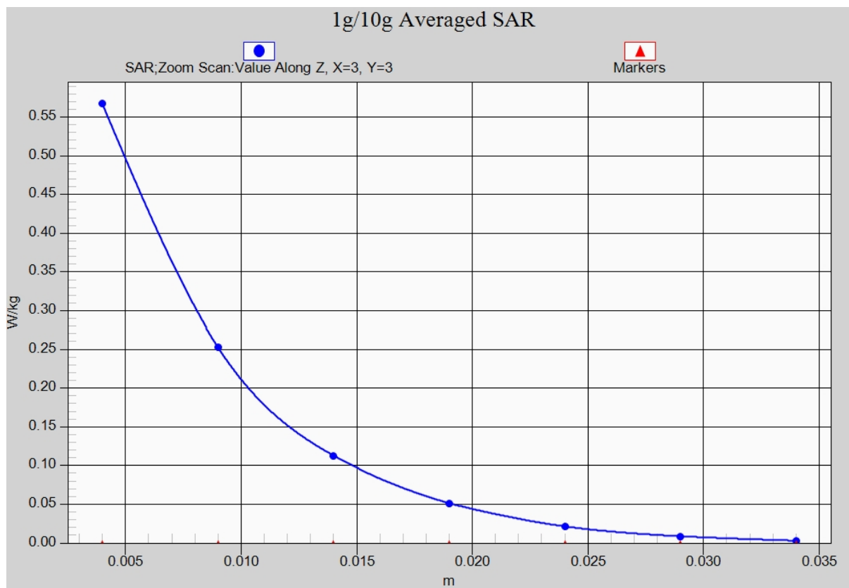
Fig. 7-1 Z-Scan at power reference point (2450 MHz CH6)
