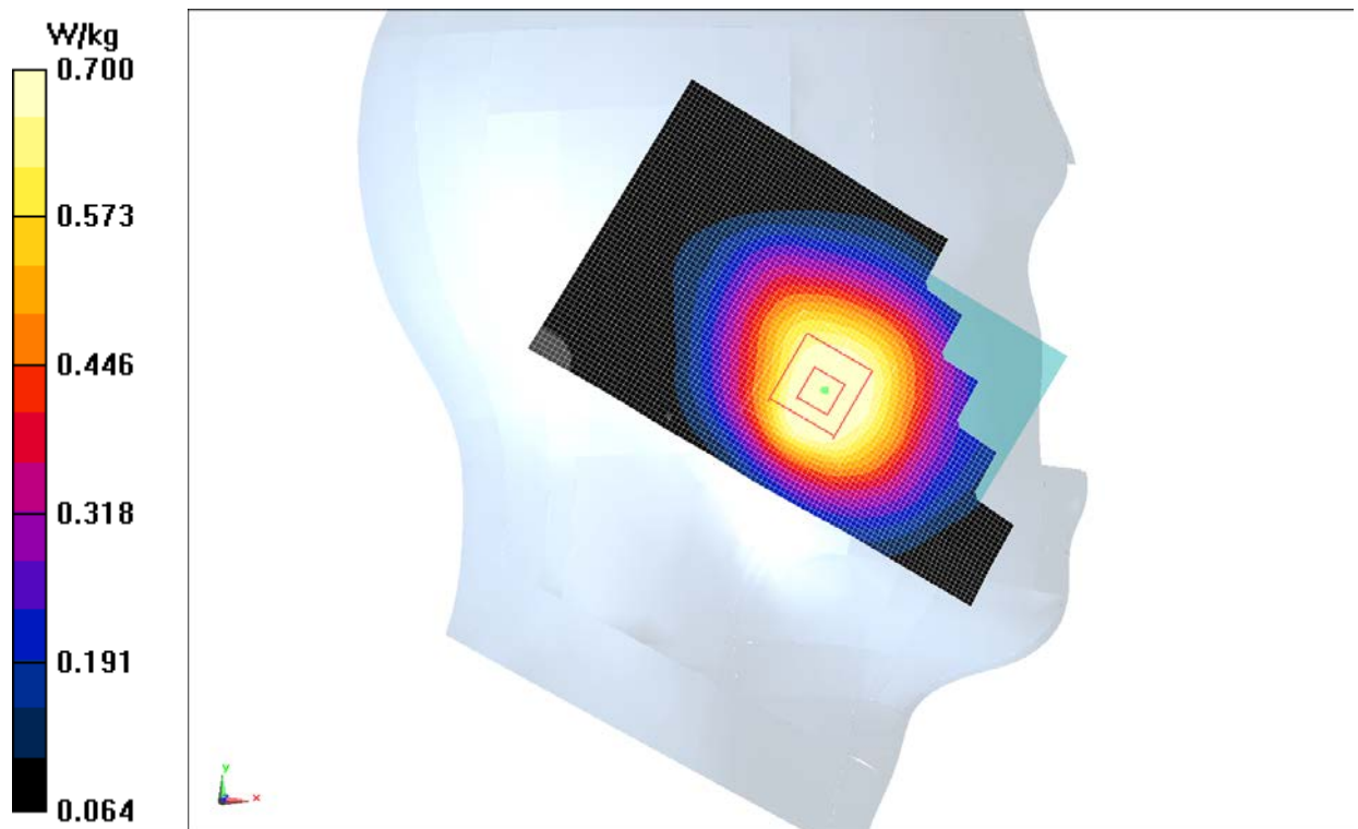
Fig.5 WCDMA 850 CH4233
