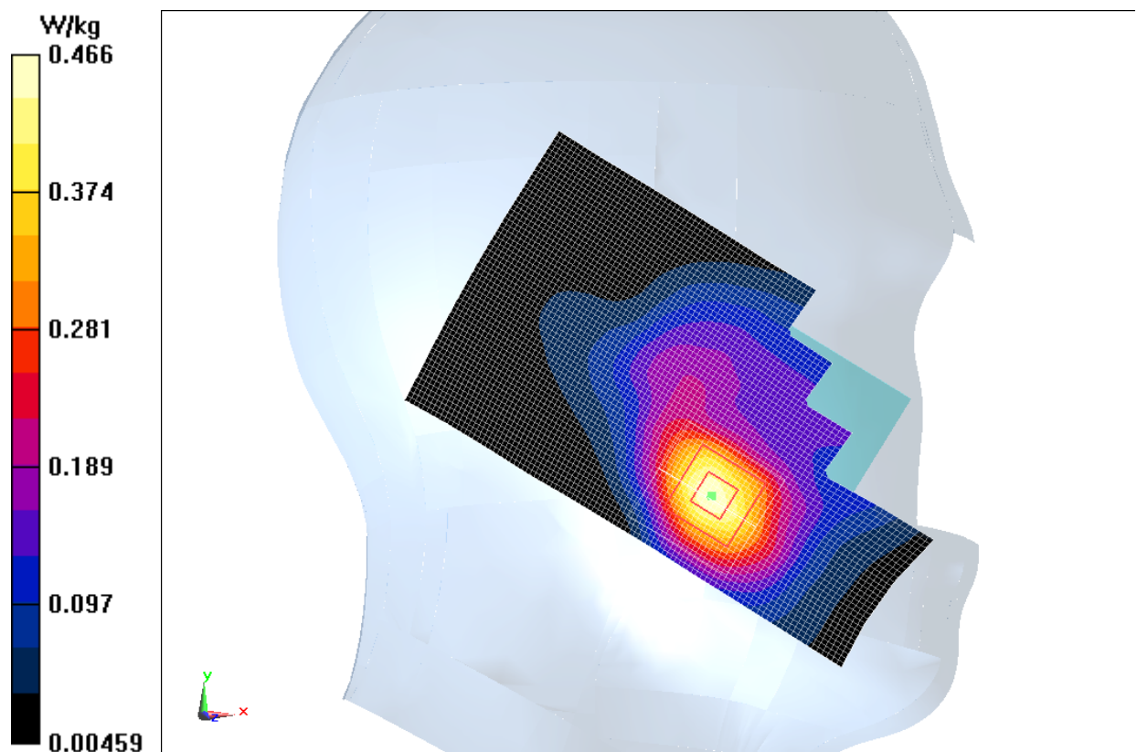
Fig.3 1900 MHz CH512
