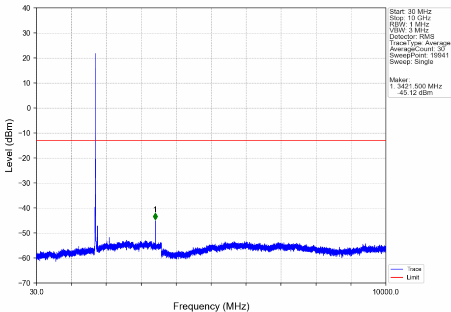
Band4_5MHz_QPSK_LCH_1712.5MHz_RB_1_0_NTNV
