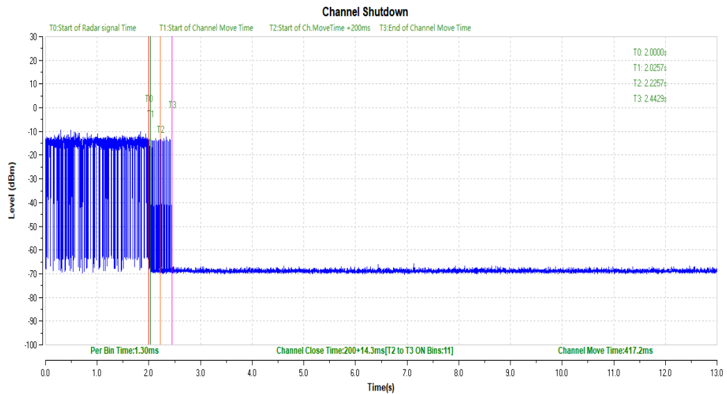
Fig.A.3 Channel move time and channel closing transmission time
