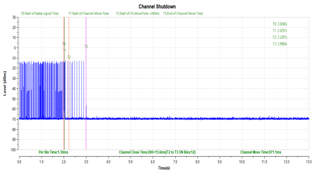
Fig.A.2 Channel move time and channel closing transmission time
