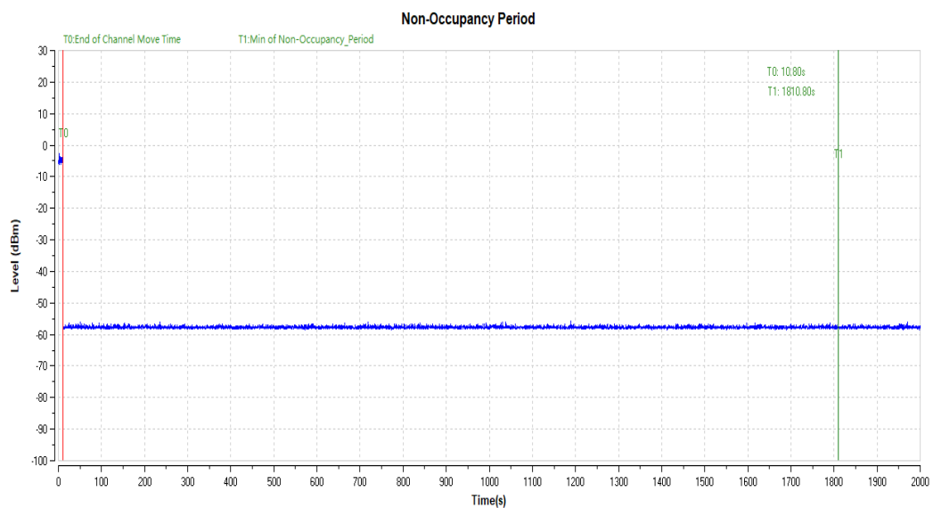
Fig.A.4 Non-Occupancy Period
