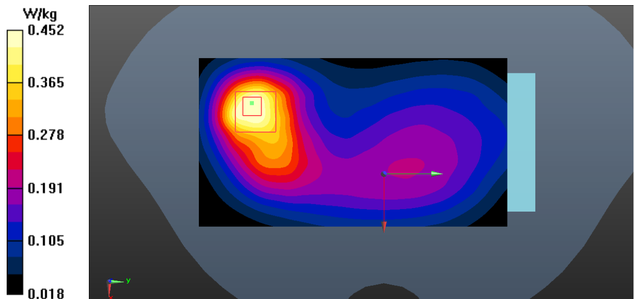
Fig.2 GSM 850 Body
