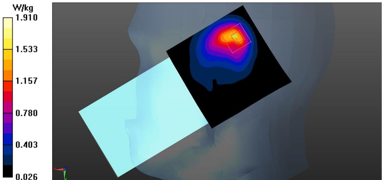
Fig.3 GSM 1900 Head
