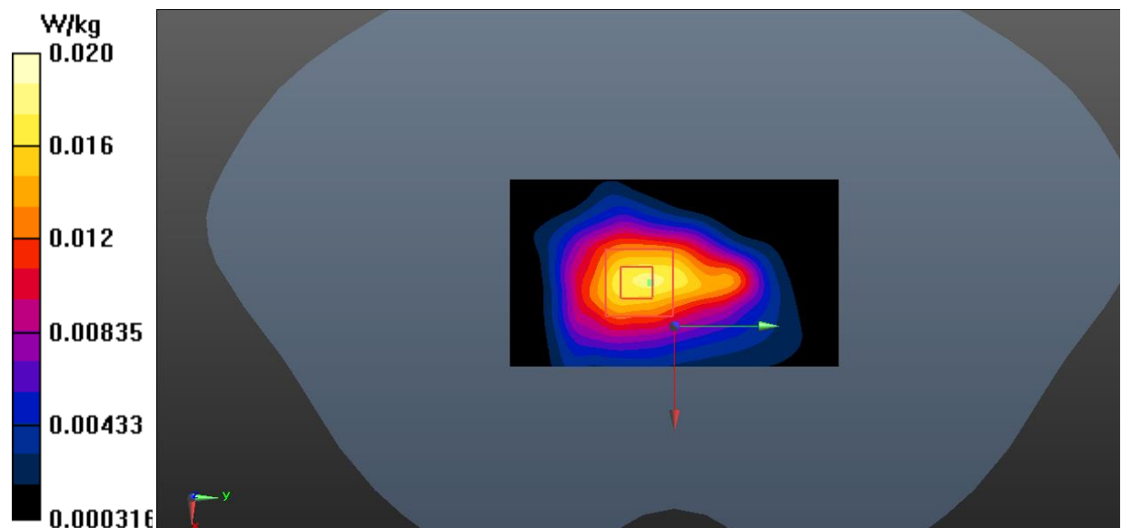
Fig.7 Bluetooth Body
