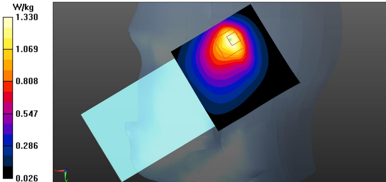
Fig.1 GSM 850 Head
