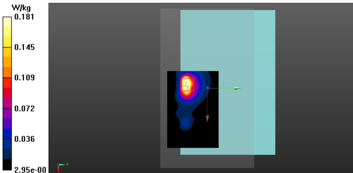
Fig.1 Bluetooth Body
