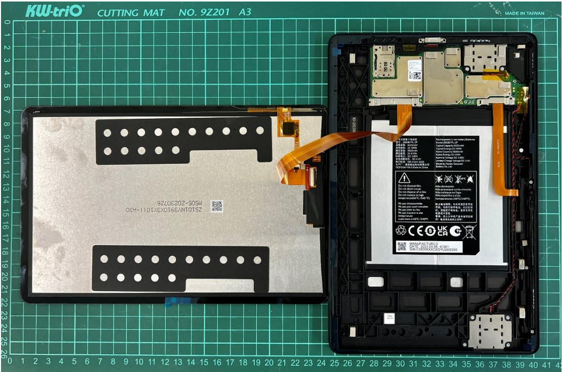
8193A Internal photos
