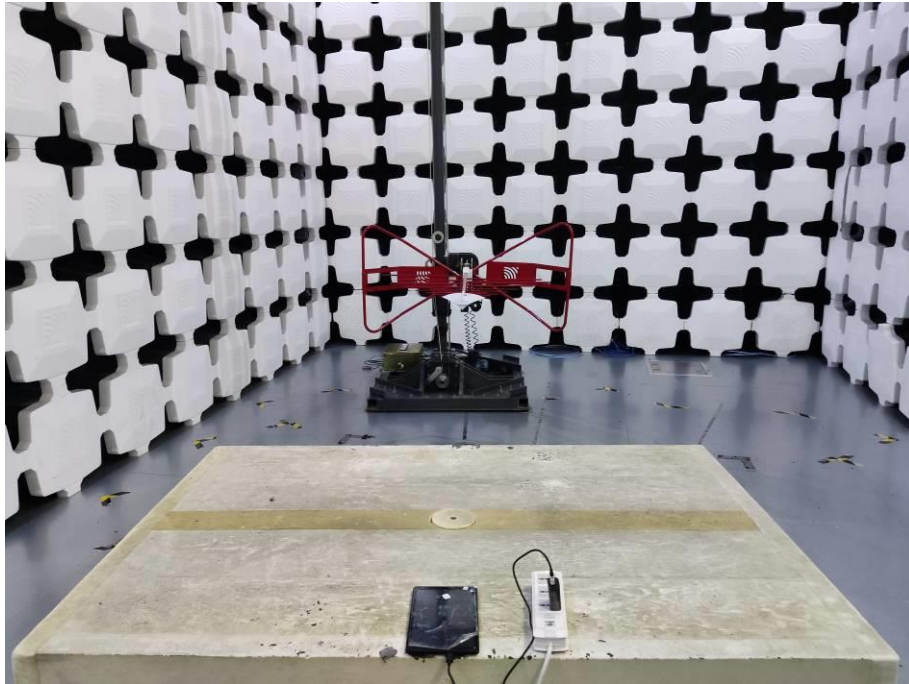
5. Radiated Emissions (Part 15B, Camera/Video Player, 30MHz-1GHz)
