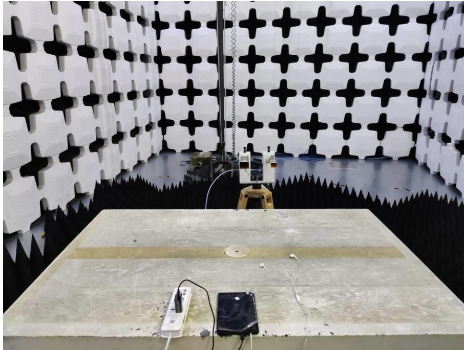
11. Radiated Emissions (Part 15B, FM receiver, 18GHz-26.5GHz)
