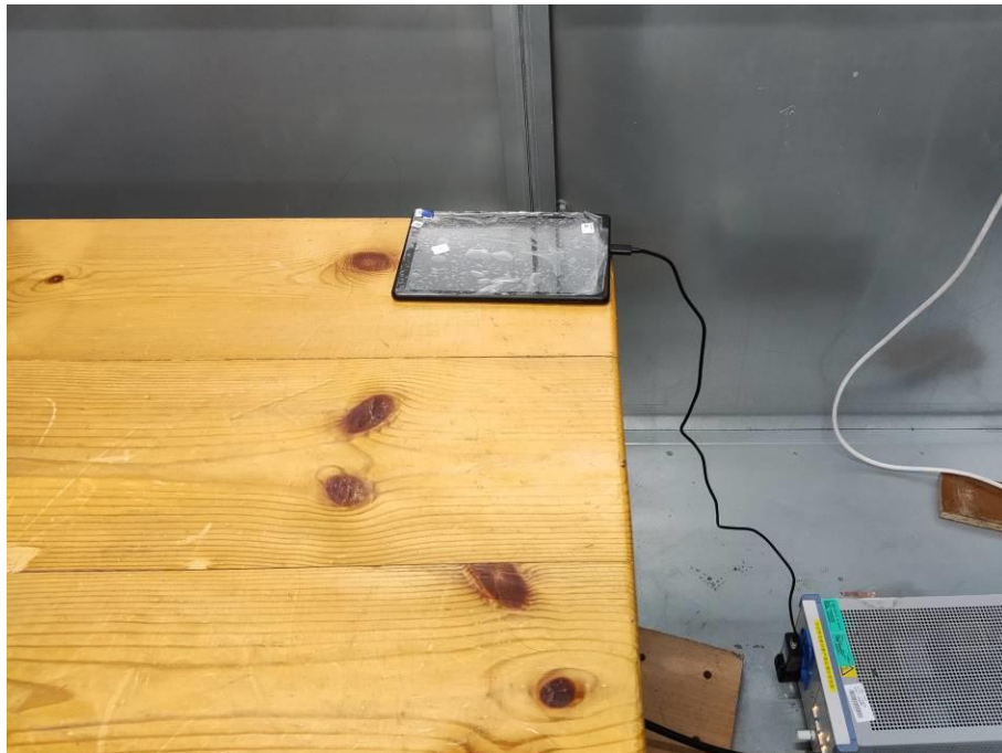
18. Conducted Emission (Part 15B& Part 15C&E, Camera/Video Player/ Wi-Fi/Bluetooth)
