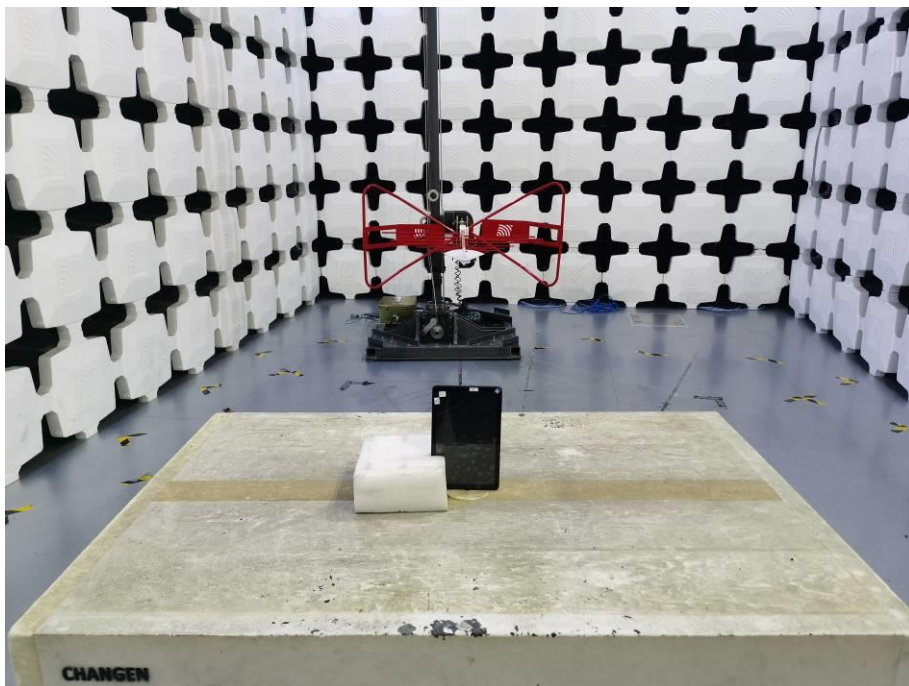
14. Radiated Emissions (Part 15C&Part 15E, 30MHz-1GHz)
