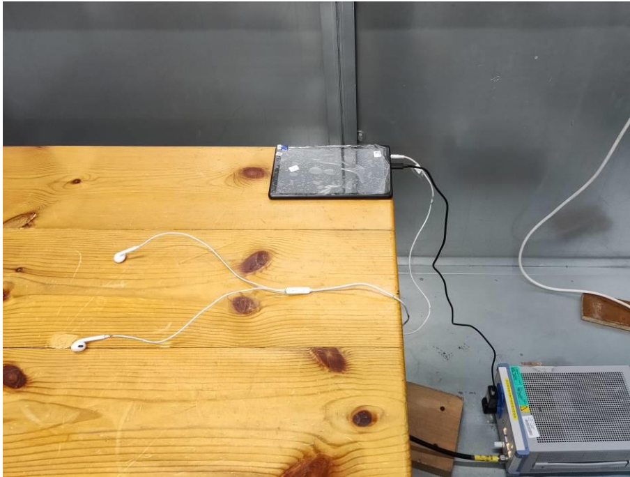
19. Conducted Emission (Part 15B, FM receiver)
