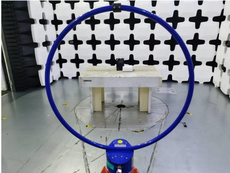
13. Radiated Emissions (Part 15C&Part 15E, 9kHz-30MHz)
