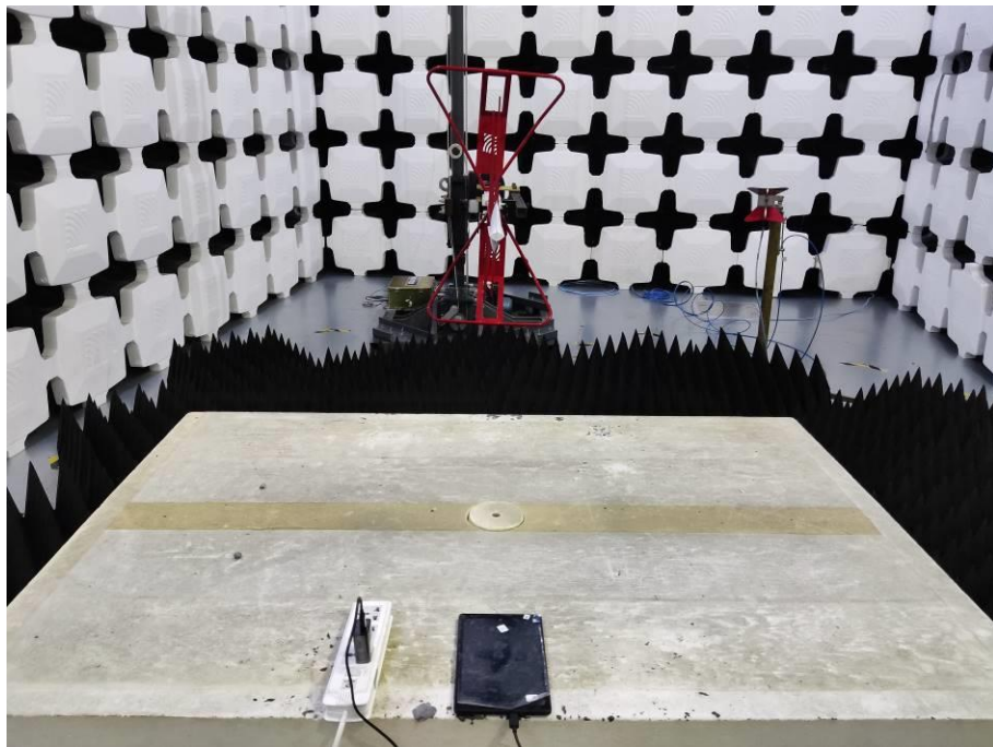
6. Radiated Emissions (Part 15B, Camera/Video Player, 1GHz-18GHz)
