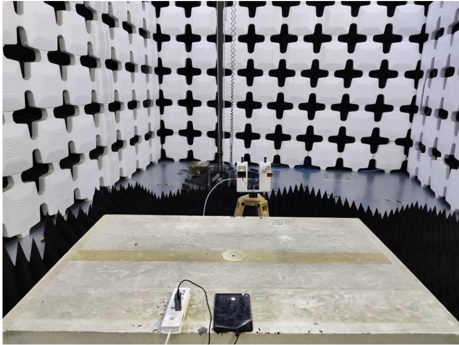
7. Radiated Emissions (Part 15B, Camera/Video Player, 18GHz-26.5GHz)
