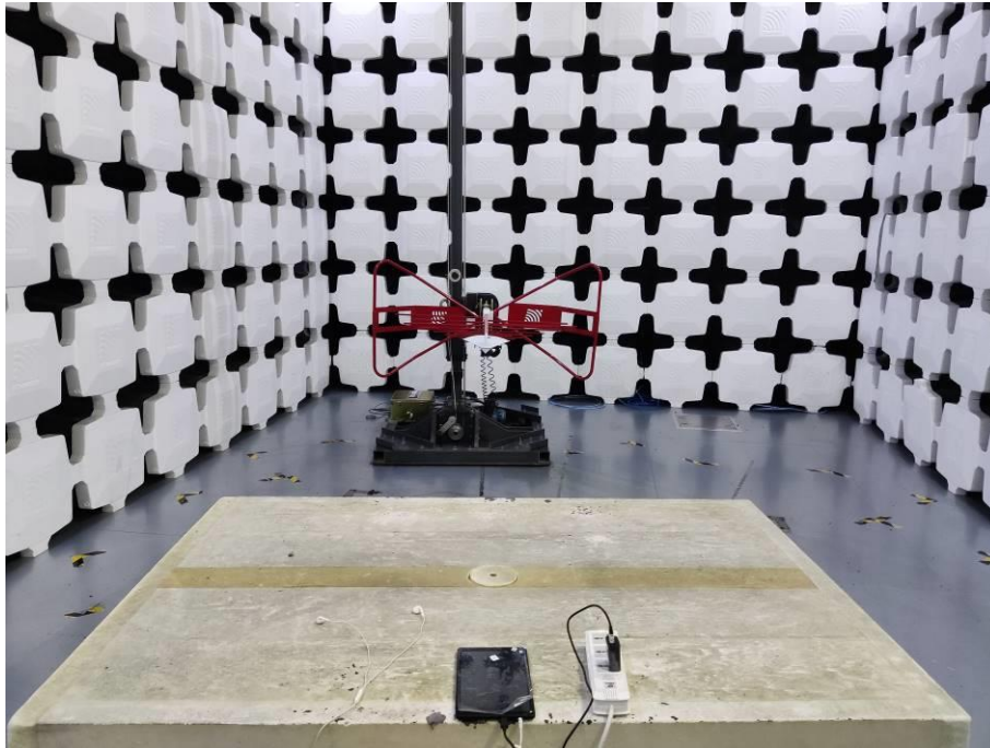
9. Radiated Emissions (Part 15B, FM receiver, 30MHz-1GHz)
