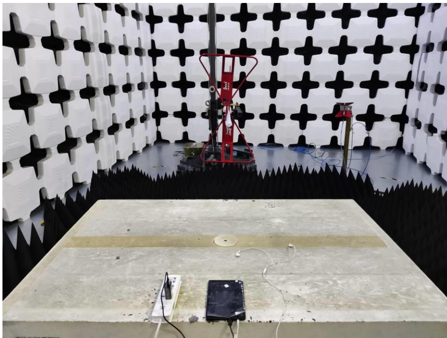
10. Radiated Emissions (Part 15B, FM receiver, 1GHz-18GHz)
