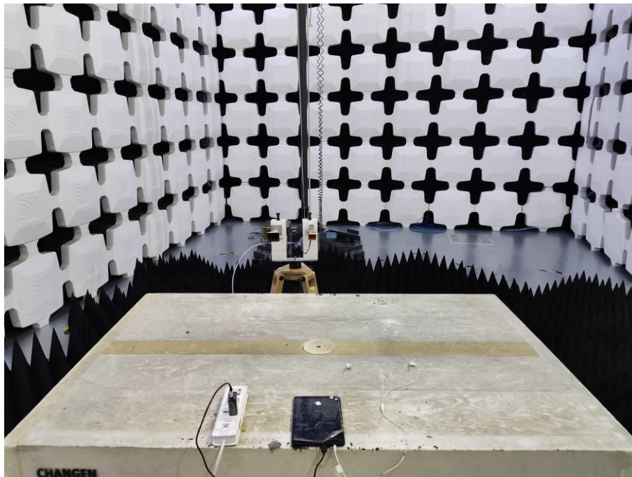
12. Radiated Emissions (Part 15B, FM receiver, 26.5GHz-40GHz)
