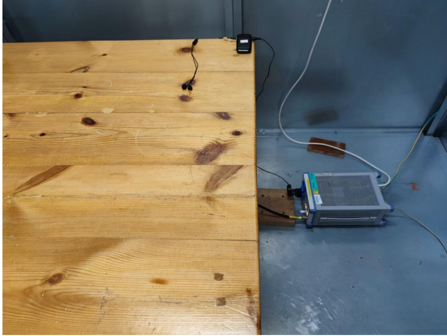
13. Conducted Emission (Part 15C, Bluetooth)
