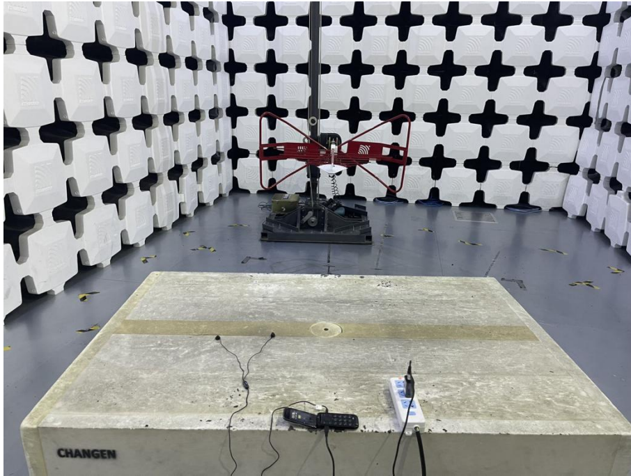
3. Radiated Emissions (Part 15B, Camera/GSM receiver,30MHz-1GHz)
