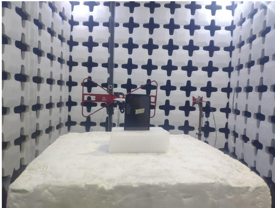
9. Radiated Emissions (Part 15C, 1GHz -18GHz)
