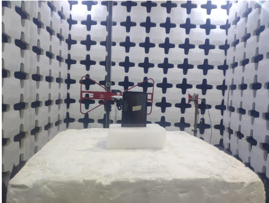
11. Radiated Emissions (Part 22/24/27,30MHz-18GHz)
