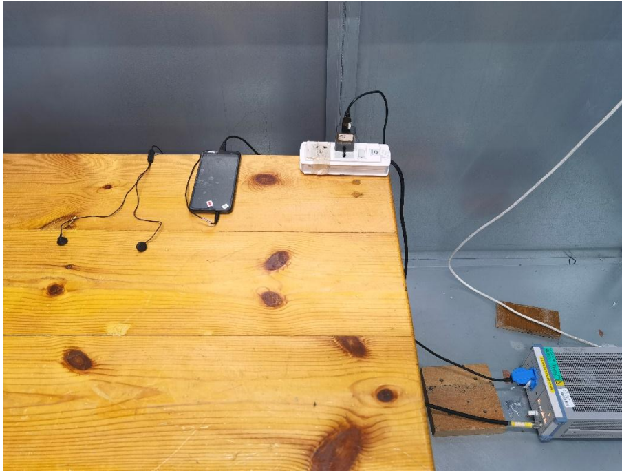
13. Conducted Emission (Part 15B, FM receiver /Camera/Video Player)
