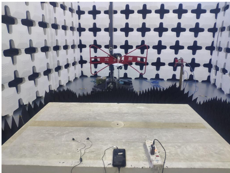
4. Radiated Emissions (Part 15B, FM receiver /Camera/Video Player /GSM receiver/WCDMA receiver/LTE receiver,30MHz-1GHz)
