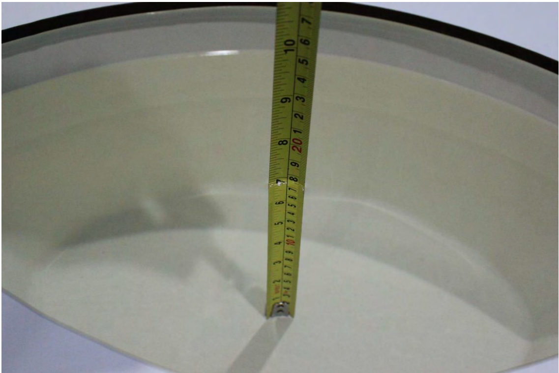
Picture 8-7 Liquid depth in the Head Phantom (3700 MHz)
