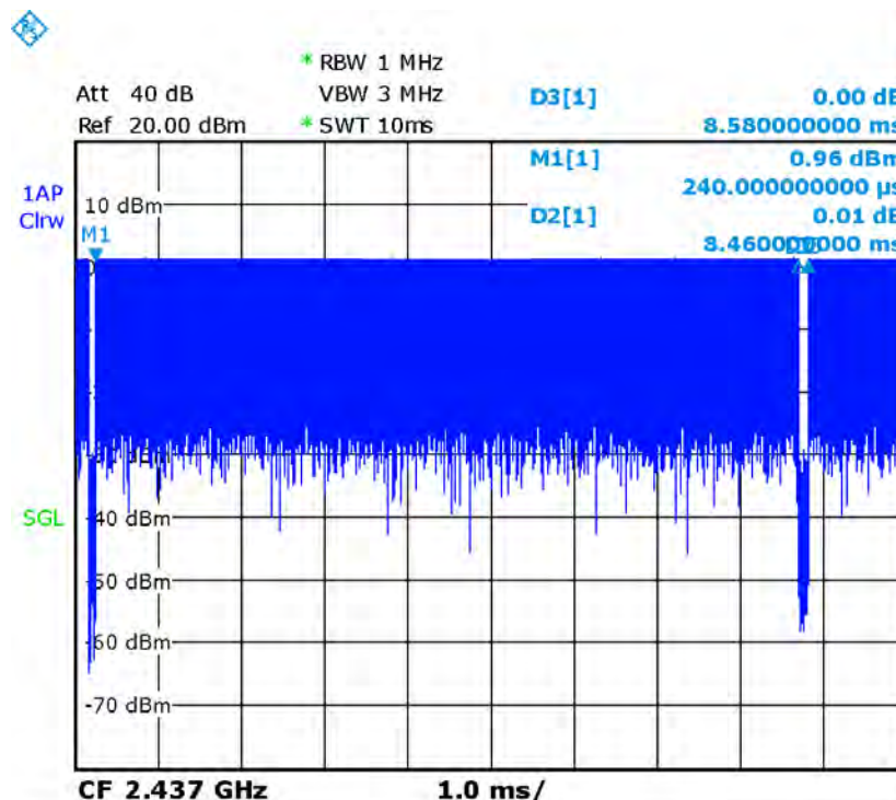
Picture 15.3 Duty factor plot for head
