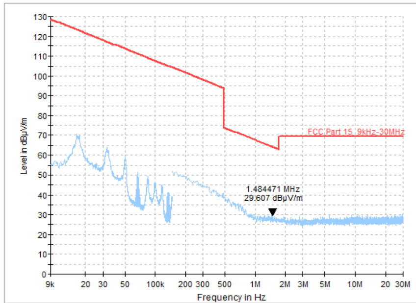
Fig.65 Radiated Spurious Emission (All Channels, 9KHz-30MHz)
