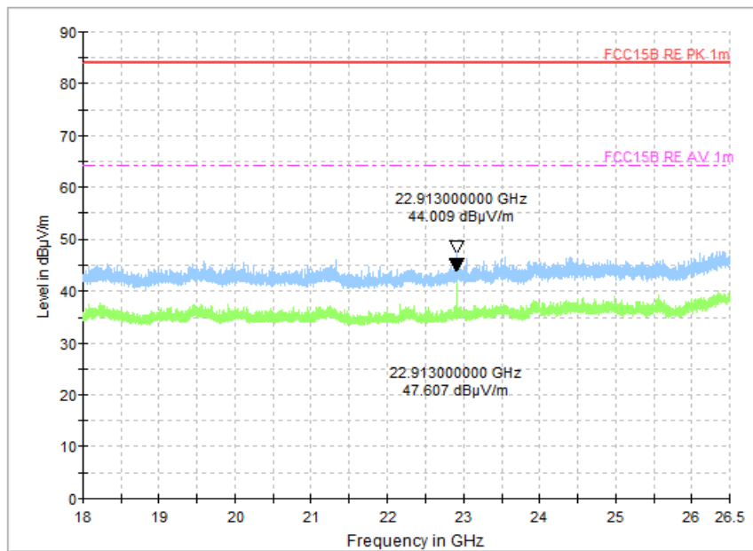
Fig.67 Radiated Spurious Emission (All Channels, 18GHz-26.5GHz)
