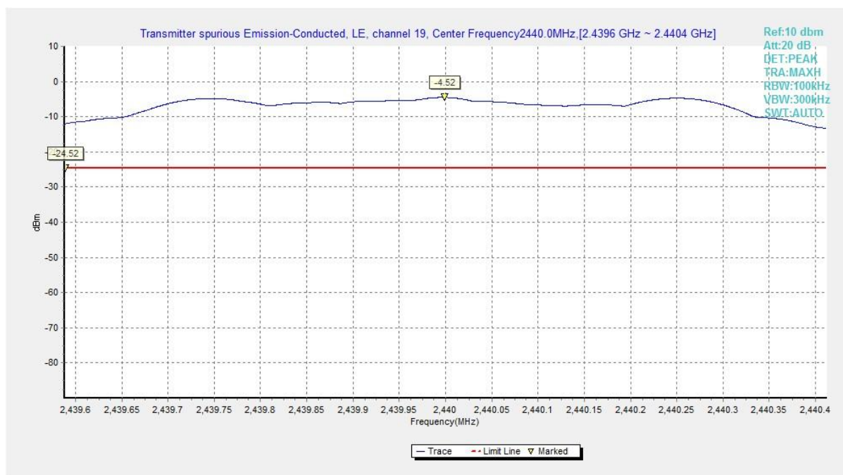
Fig.12 Conducted Spurious Emission (Ch19, Center Frequency), LE 1M
