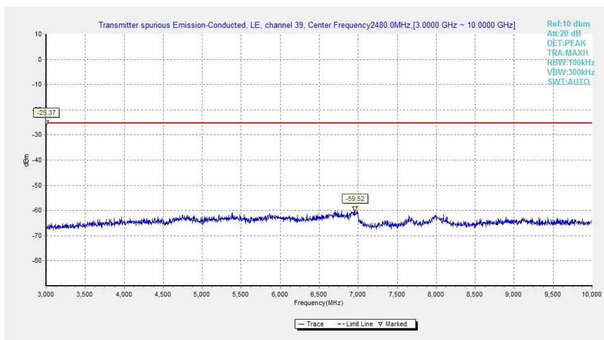
Fig.17 Conducted Spurious Emission (Ch39, 3 GHz-10 GHz), LE 1M
