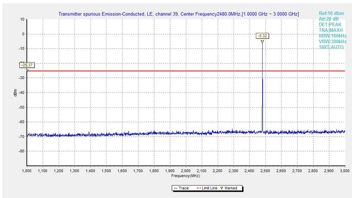
Fig.16 Conducted Spurious Emission (Ch39, 1 GHz-3 GHz), LE 1M
