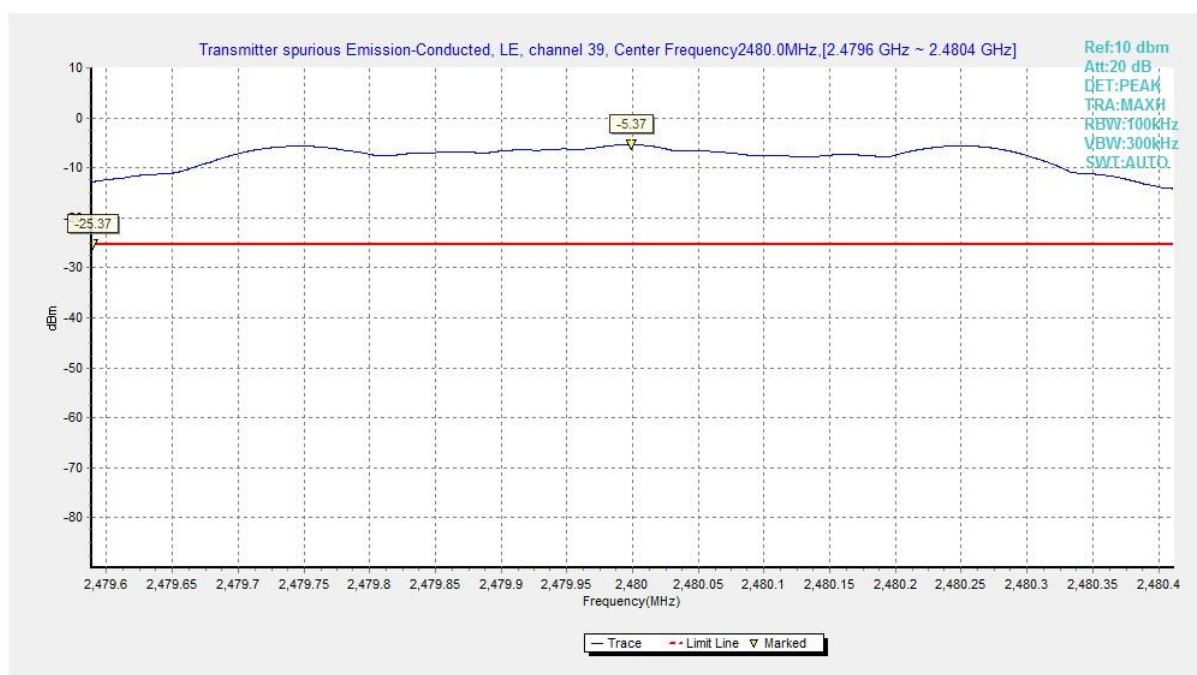
Fig.15 Conducted Spurious Emission (Ch39, Center Frequency), LE 1M
