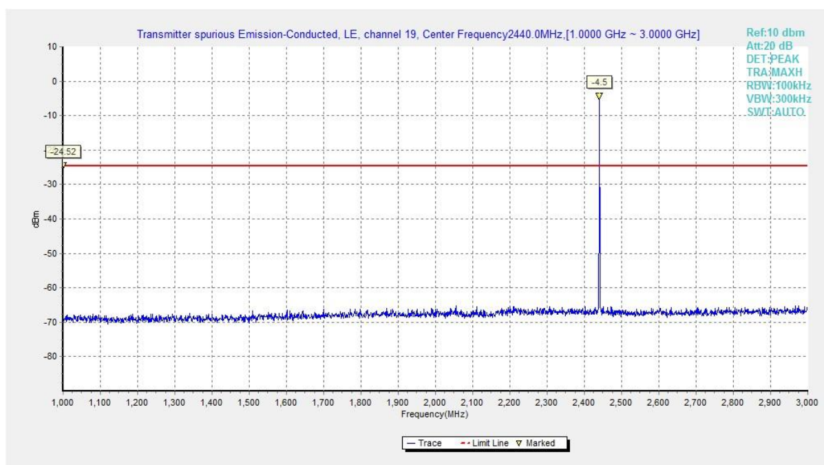
Fig.13 Conducted Spurious Emission (Ch19, 1 GHz-3 GHz), LE 1M
