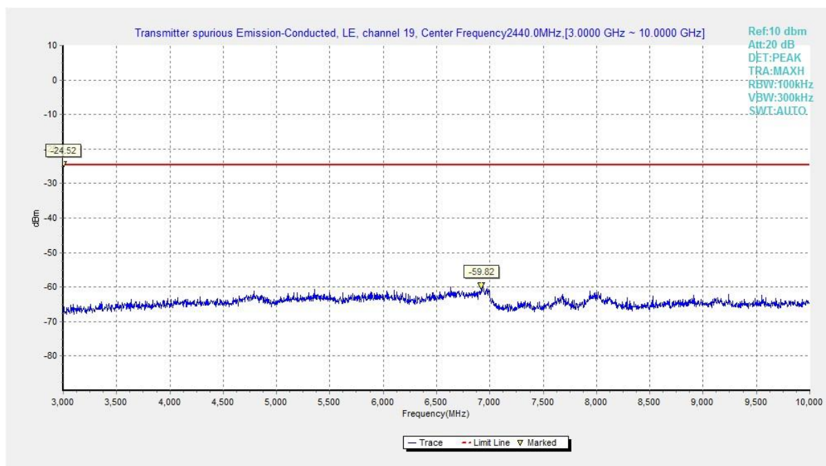
Fig.14 Conducted Spurious Emission (Ch19, 3 GHz-10 GHz), LE 1M
