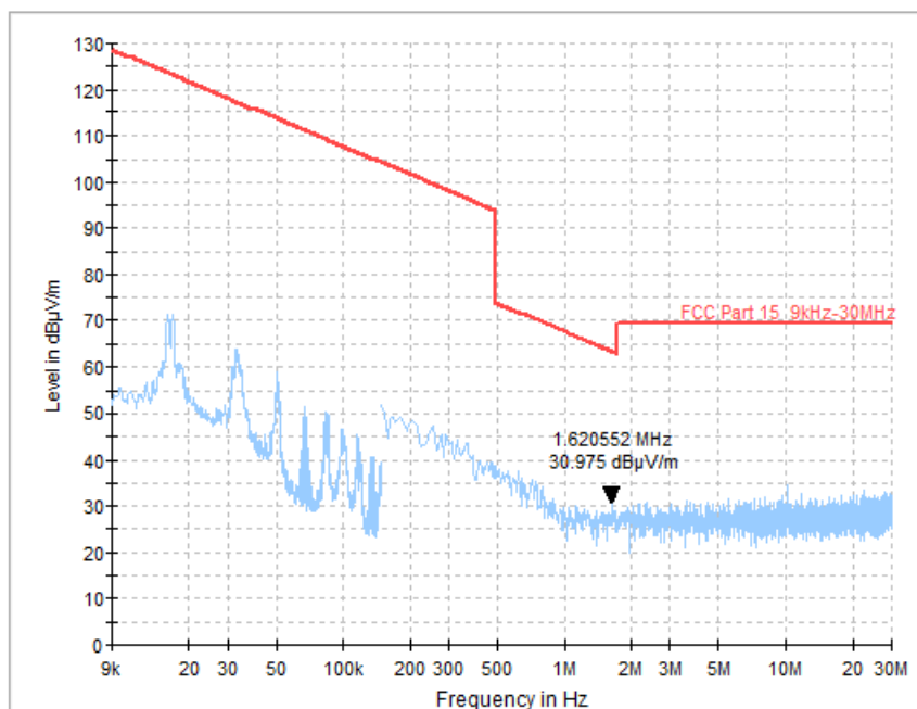
Fig.21 Radiated Spurious Emission (Ch19, 9 kHz - 30 MHz), 1M
