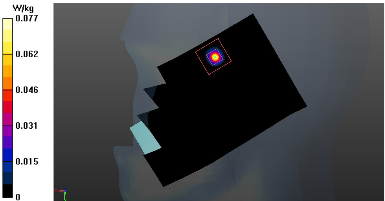
Fig.21 Bluetooth Head
