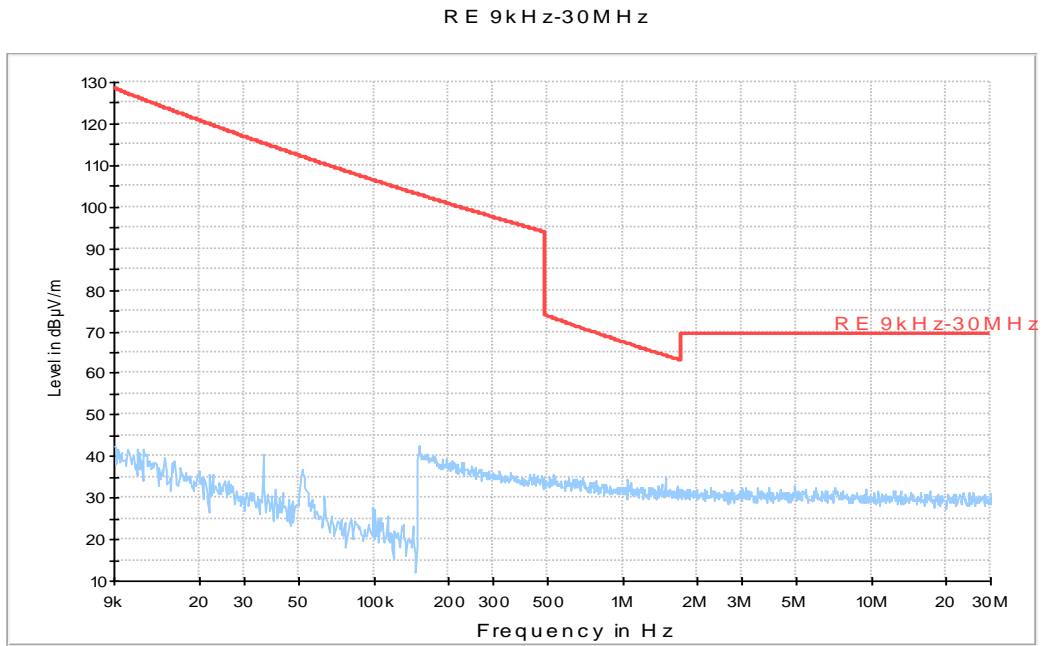
Fig.A.6.2.4 Transmitter Spurious Emission - Radiated (802.11b, Ch6, 9kHz-30 MHz)
