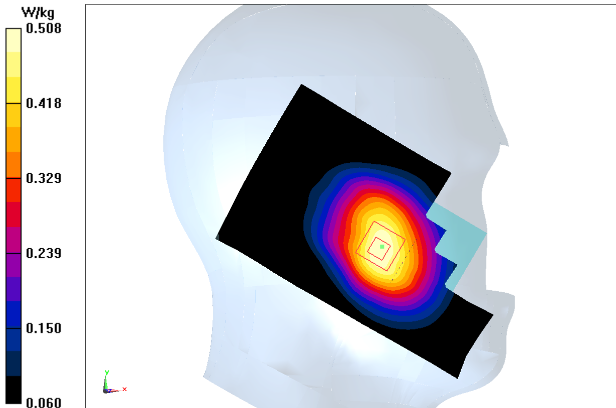
Fig.1 850MHz
