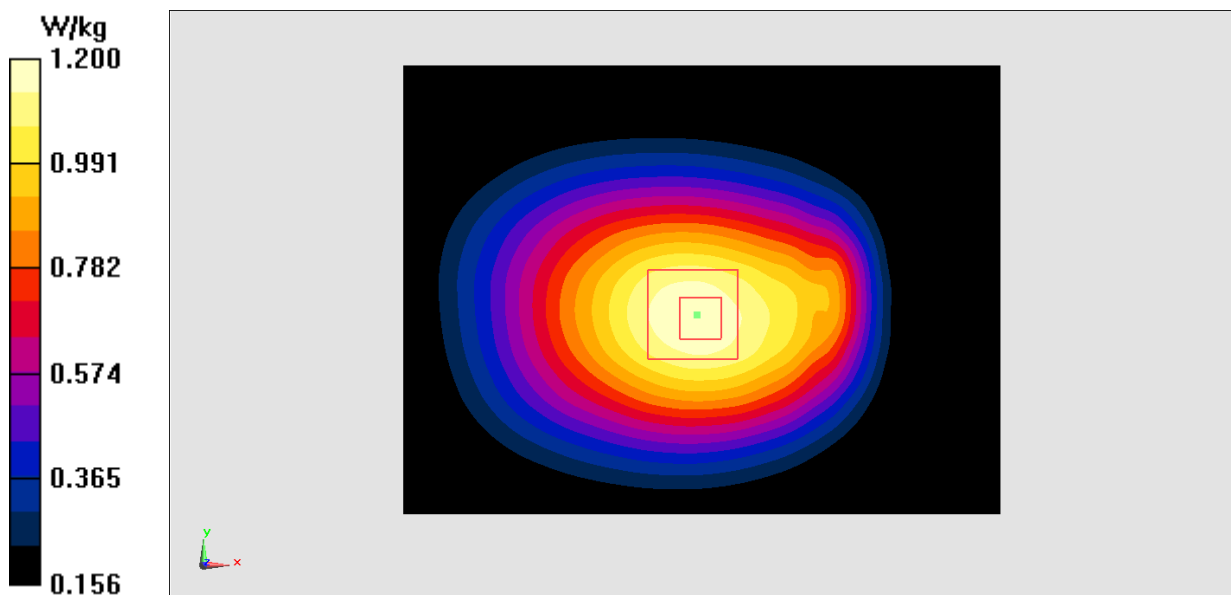
Fig.2 850 MHz
