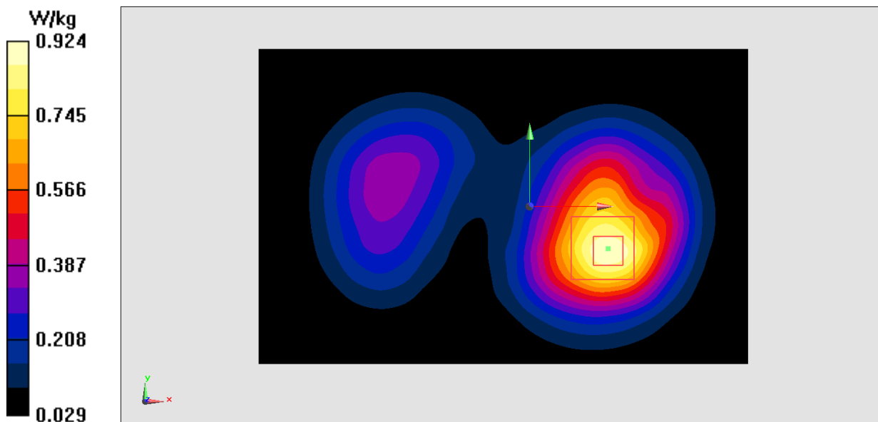
Fig.4 1900 MHz
