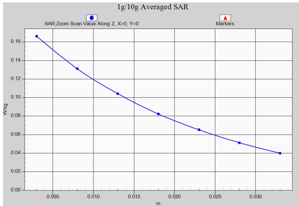
Fig. 19-1 Z-Scan at power reference point (LTE Band13)
