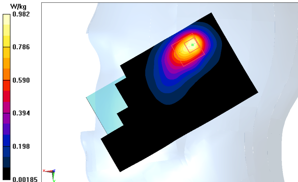
Fig.21 2450 MHz
