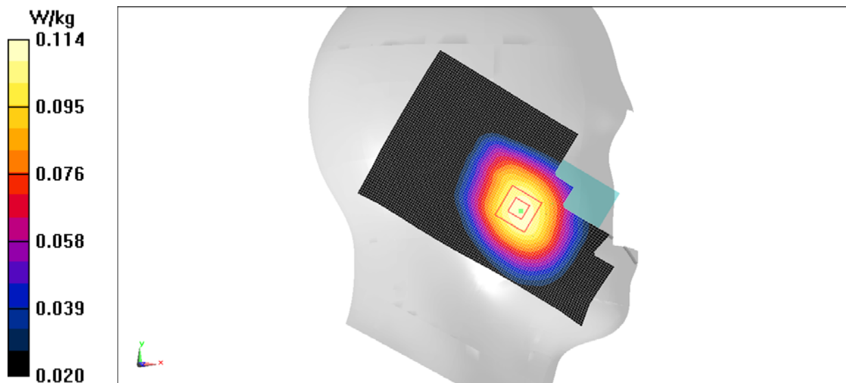
Fig.17 LTE Band12
