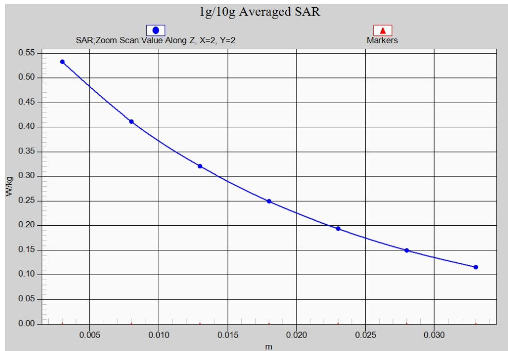
Fig. 20-1 Z-Scan at power reference point (LTE Band13)
