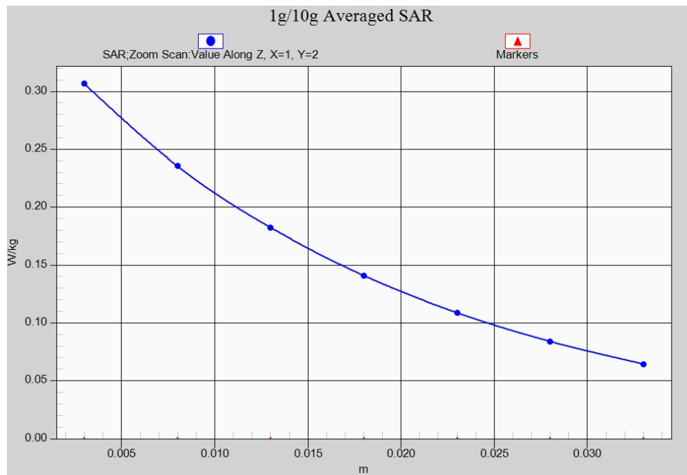
Fig. 18-1 Z-Scan at power reference point (LTE Band12)
