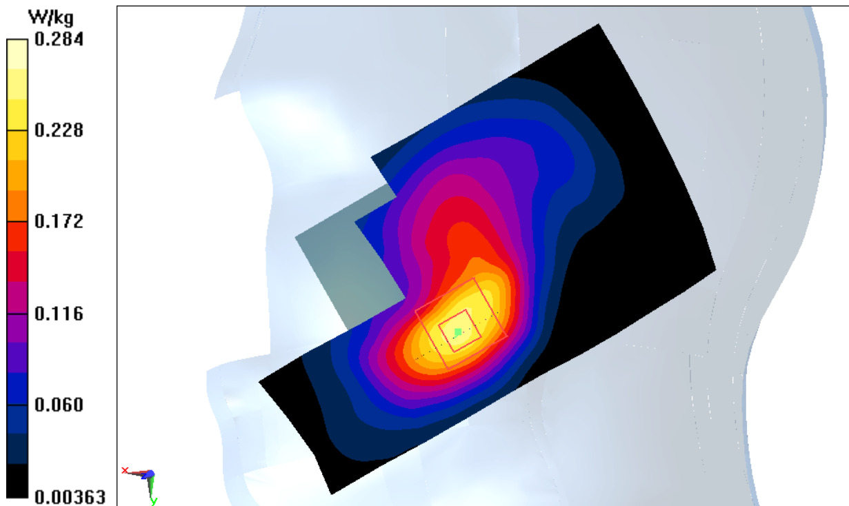
Fig.3 1900 MHz
