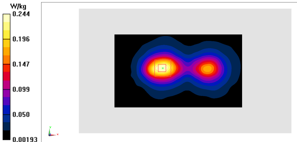
Fig.22 2450 MHz
