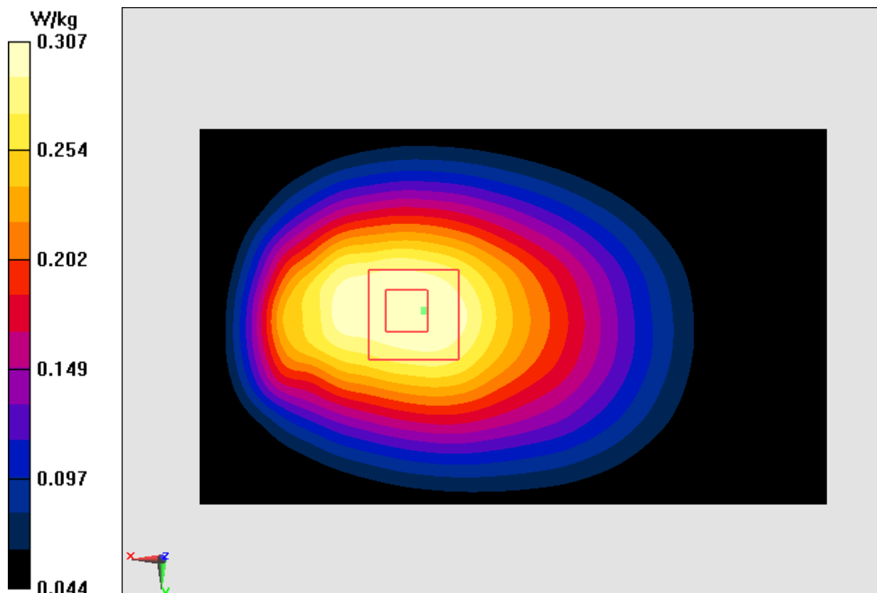
Fig.18 LTE Band12
