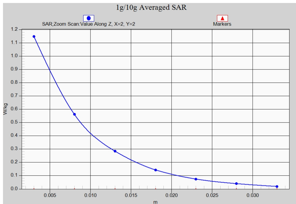
Fig. 16-1 Z-Scan at power reference point (LTE Band7) AP ON
