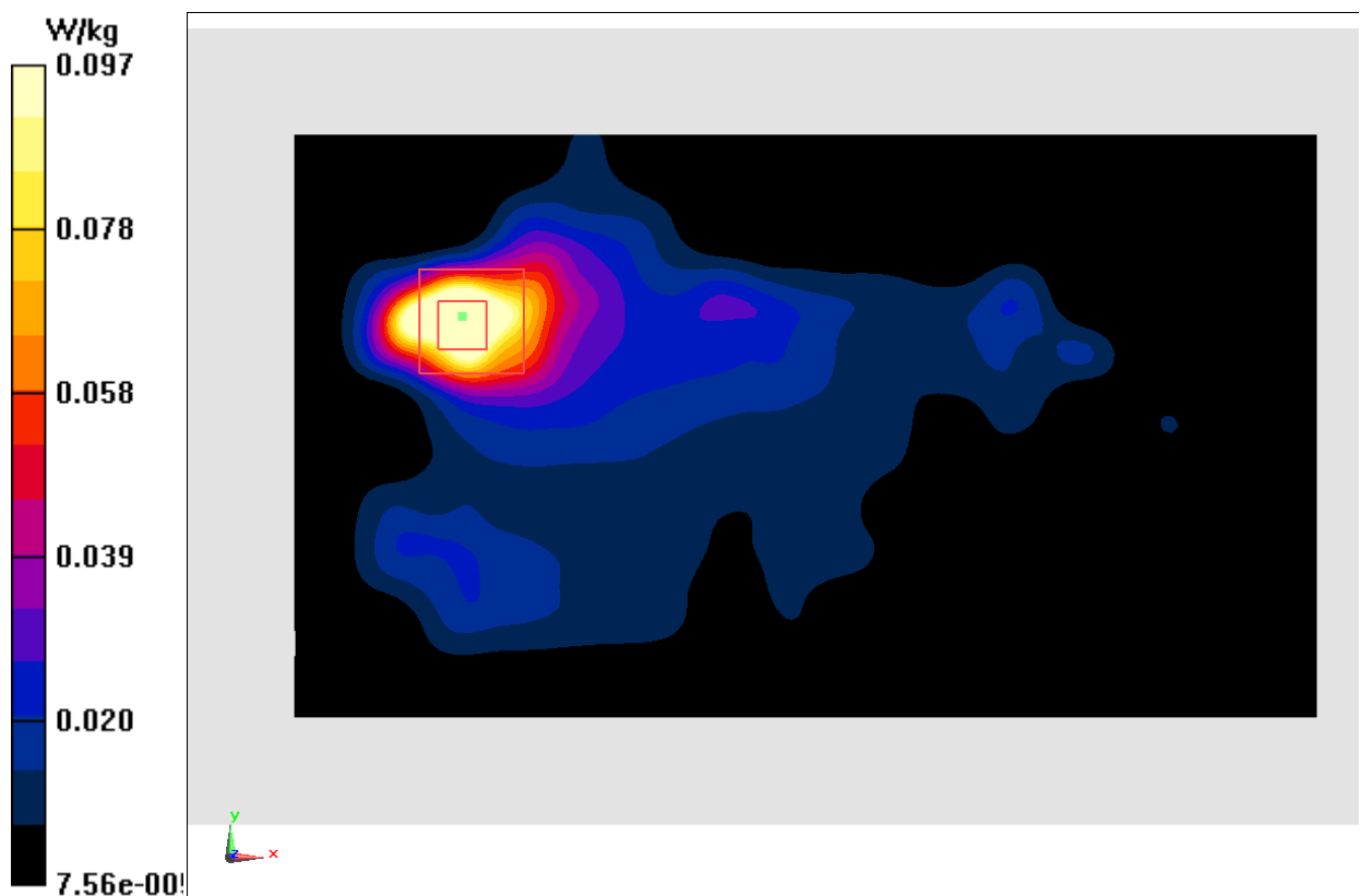
Fig.25 2450 MHz
