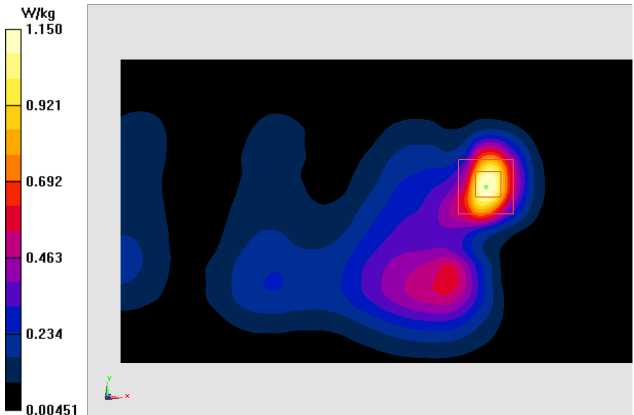
Fig.16 LTE Band7 AP ON
