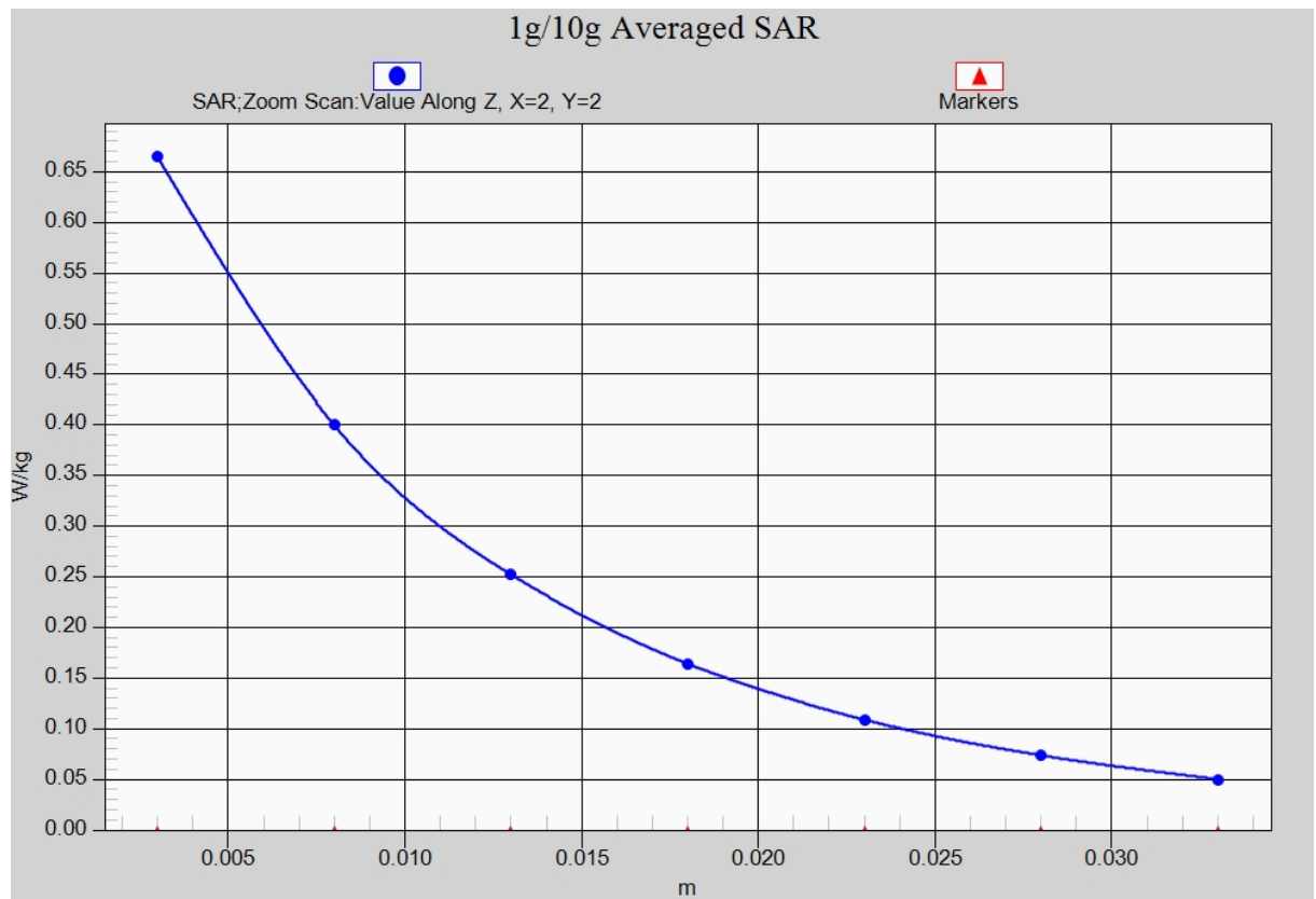
Fig. 23-1 Z-Scan at power reference point (LTE Band5)
