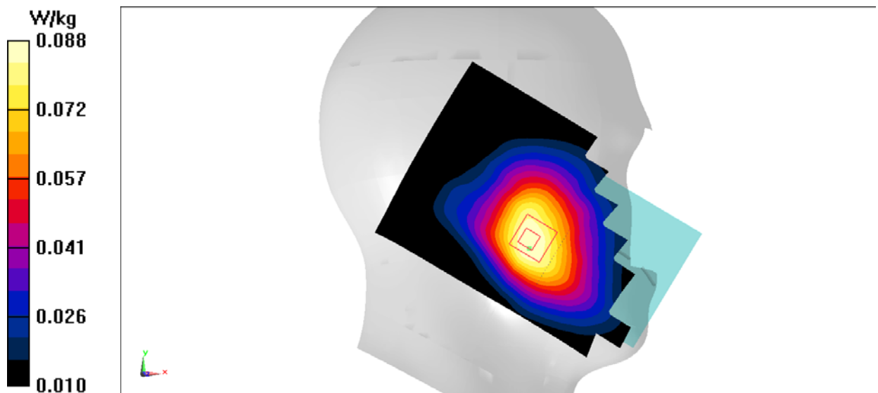
Fig.18 LTE Band12
