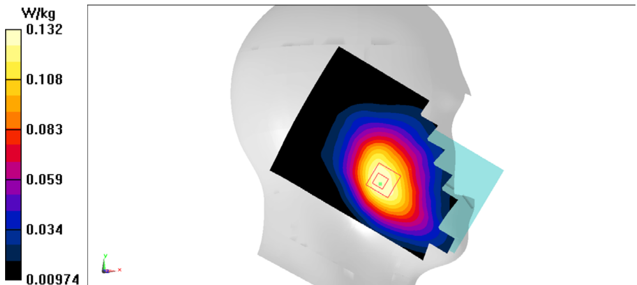
Fig.22 LTE Band5
