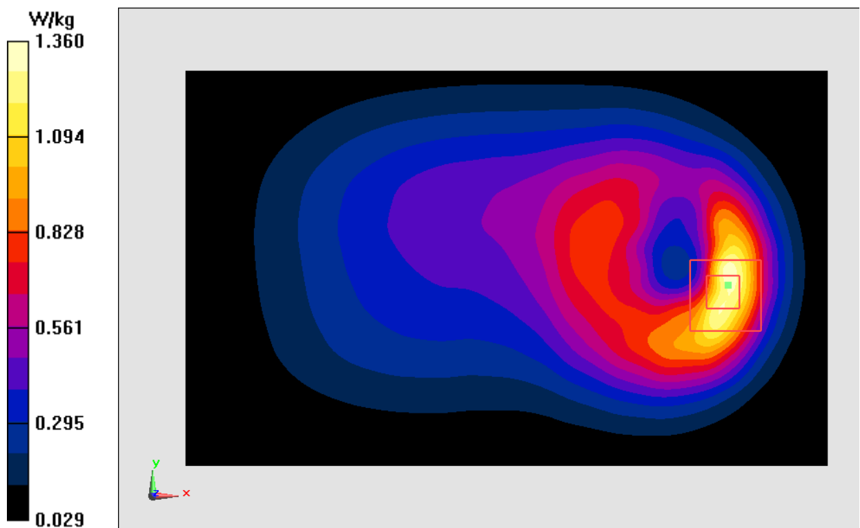
Fig.2 850 MHz
