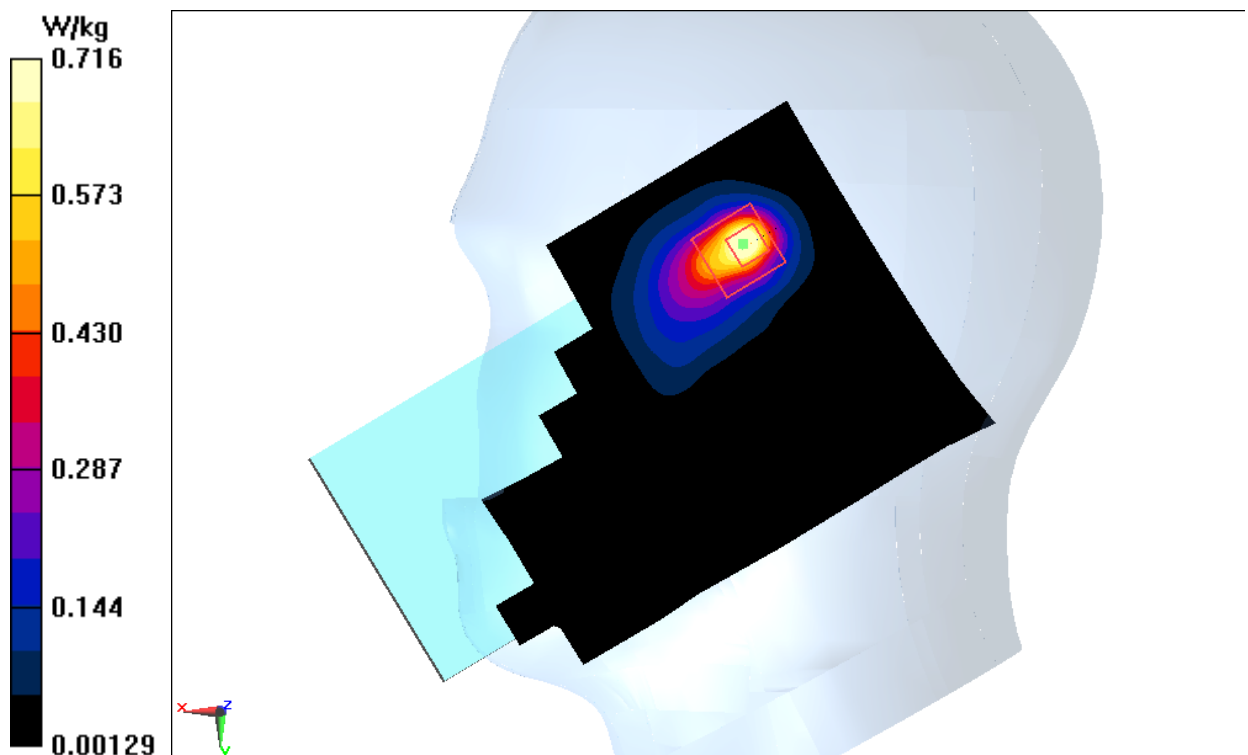
Fig.24 2450 MHz
