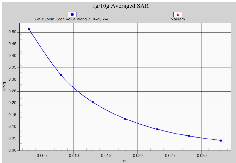
Fig. 21-1 Z-Scan at power reference point (LTE Band13)
