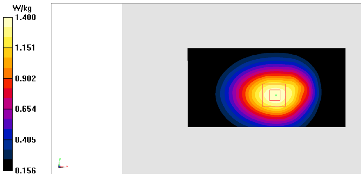
Fig.2 850 MHz
