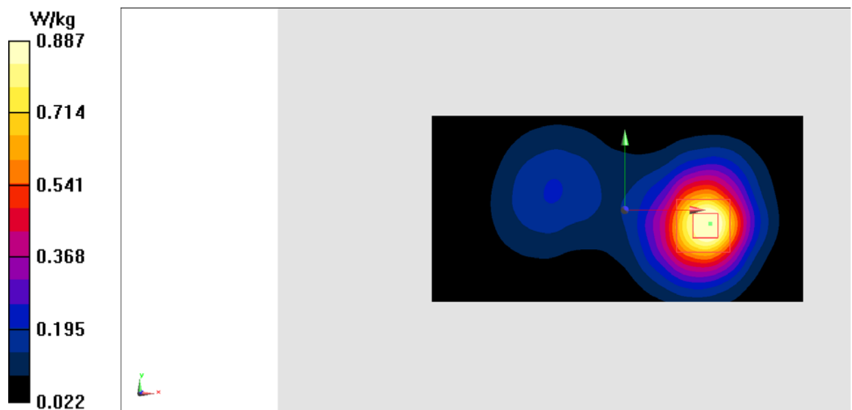
Fig.4 1900 MHz
