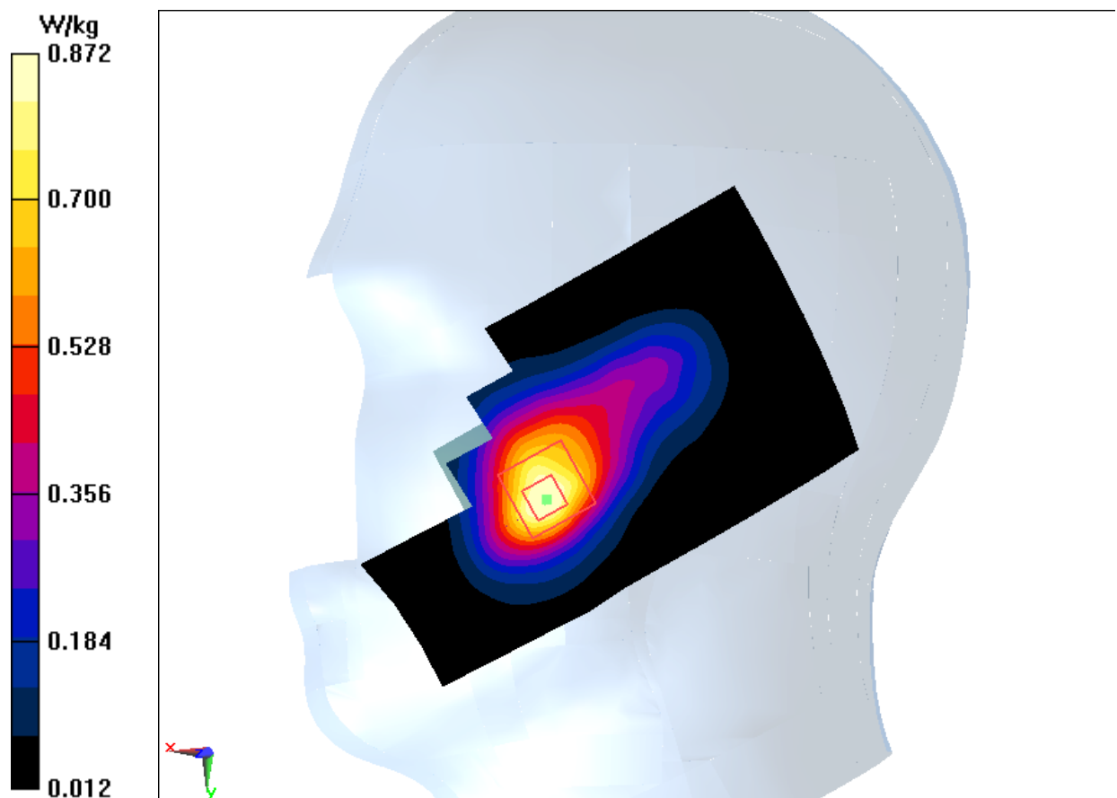
Fig.3 1900 MHz
