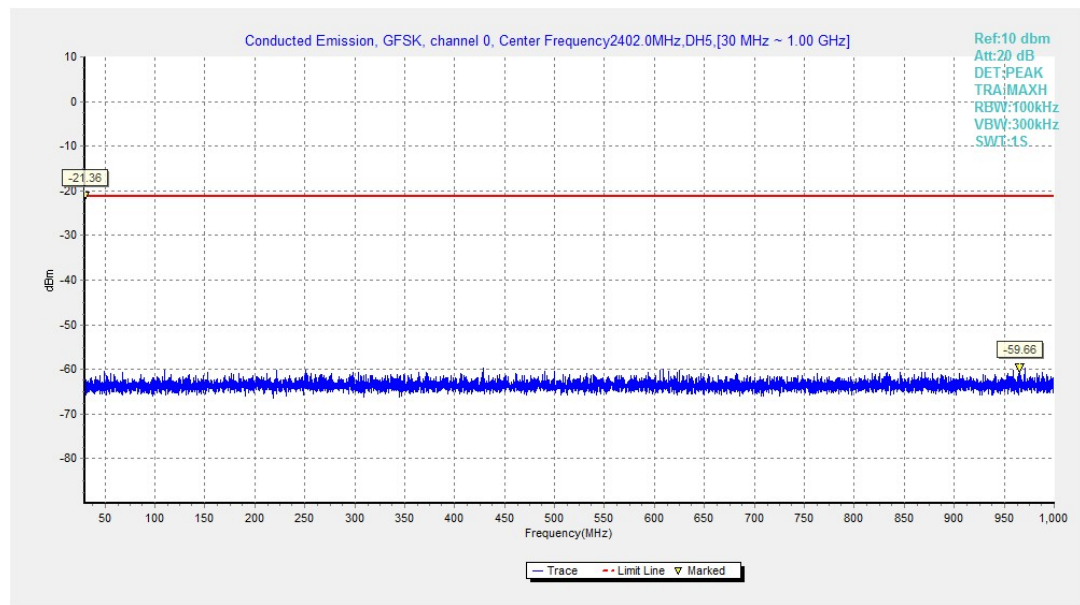
Fig.14. Conducted spurious emission: GFSK, Channel 0, 30MHz - 1GHz
