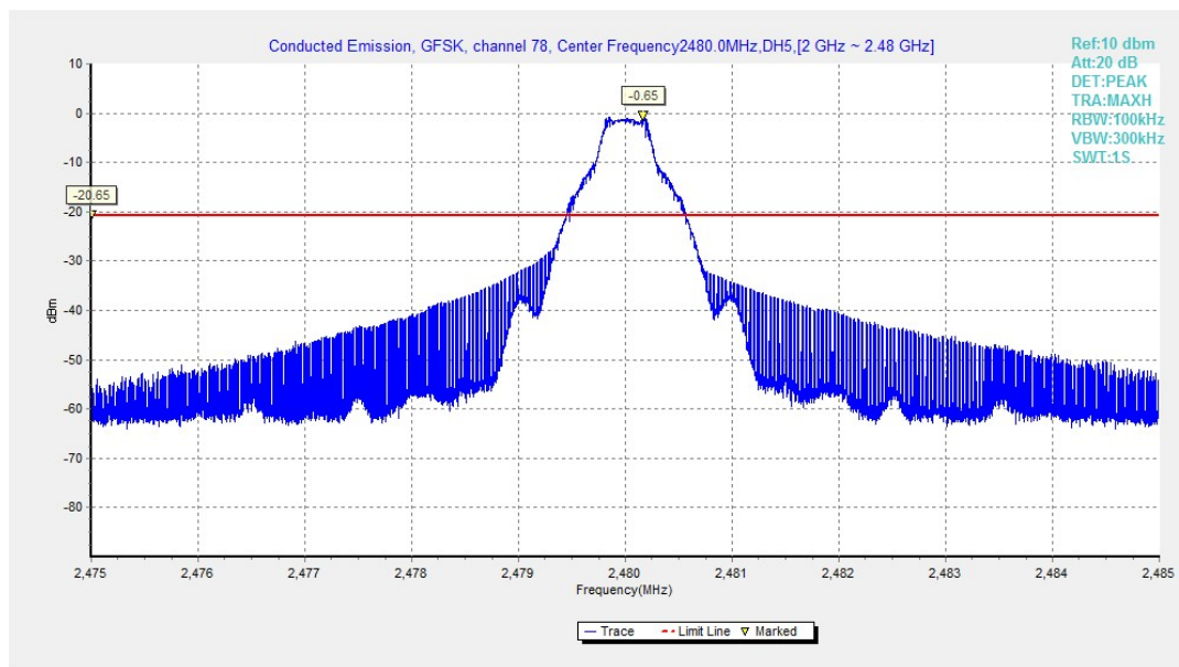
Fig.23. Conducted spurious emission: GFSK, Channel 78, 2480MHz
