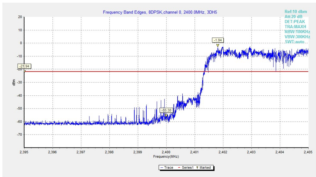
Fig.10. Frequency Band Edges: 8DPSK, Channel 0, Hopping On
