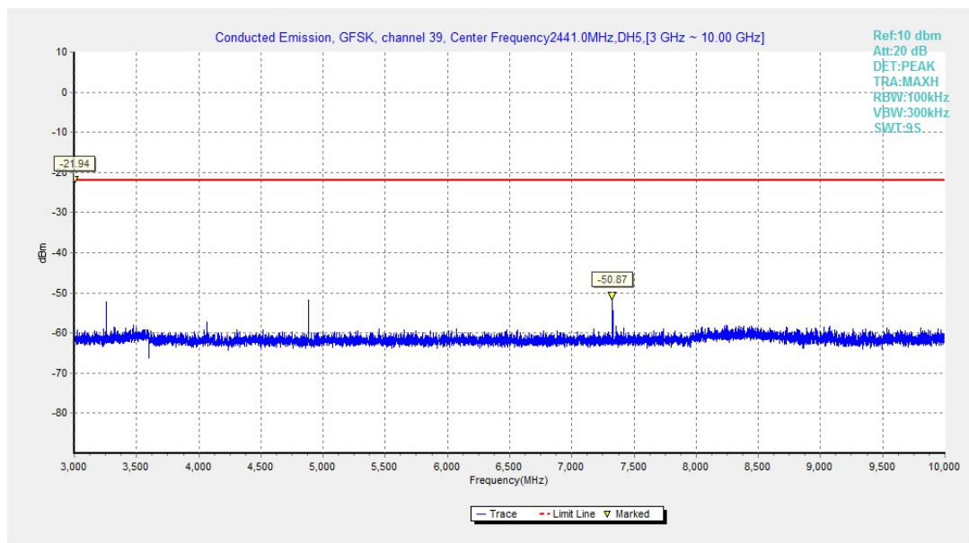
Fig.21. Conducted spurious emission: GFSK, Channel 39, 3GHz – 10GHz
