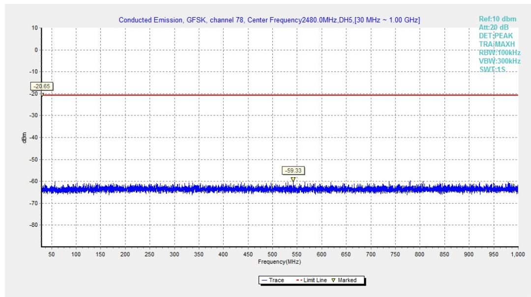
Fig.24. Conducted spurious emission: GFSK, Channel 78, 30MHz - 1GHz
