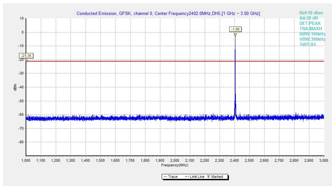
Fig.15. Conducted spurious emission: GFSK, Channel 0, 1GHz - 3GHz
