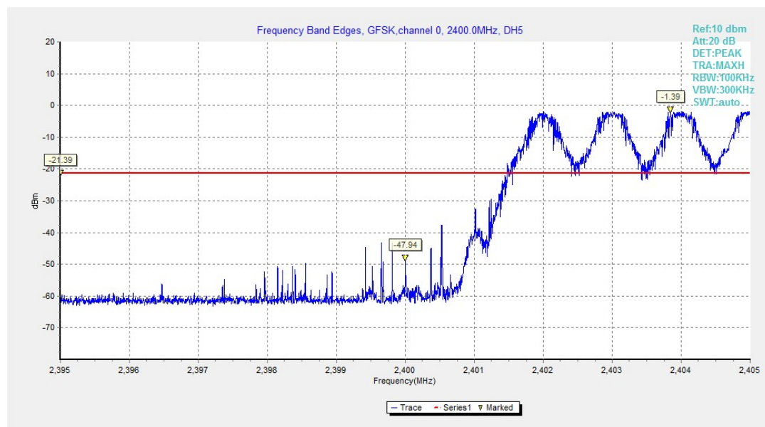
Fig.2. Frequency Band Edges: GFSK, Channel 0, Hopping On
