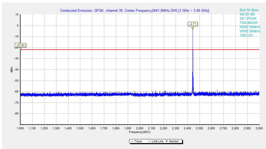
Fig.20. Conducted spurious emission: GFSK, Channel 39, 1GHz – 3GHz
