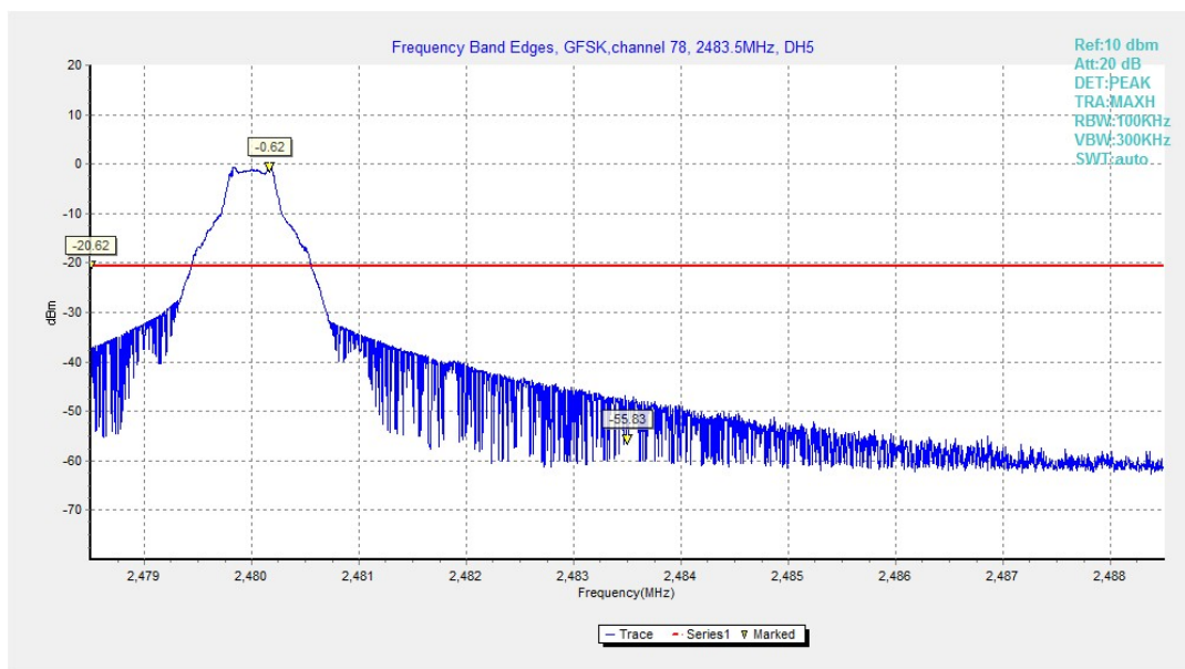
Fig.3. Frequency Band Edges: GFSK, Channel 78, Hopping Off
