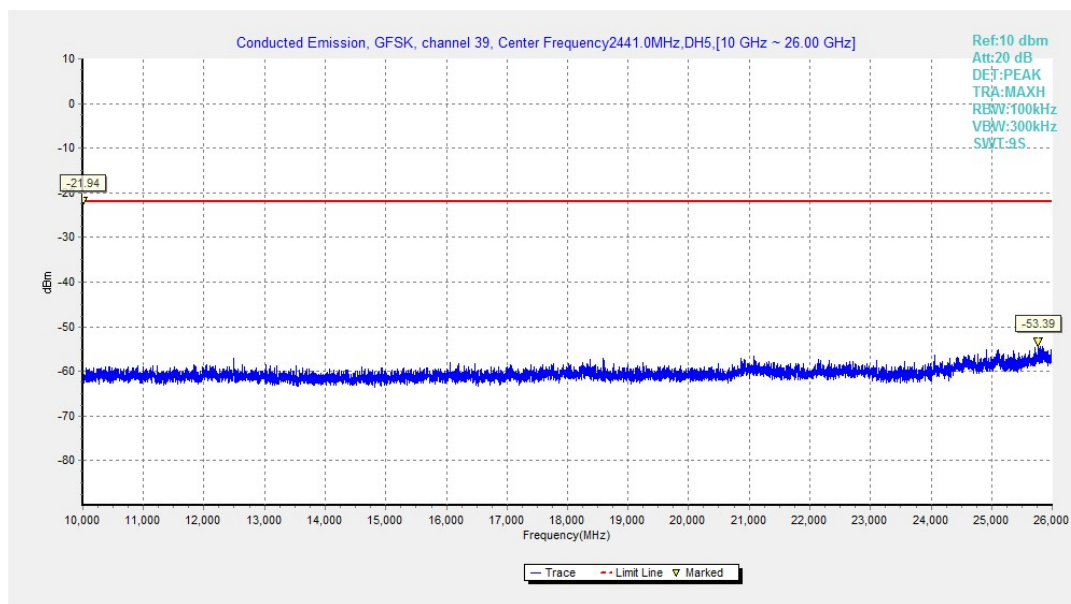
Fig.22. Conducted spurious emission: GFSK, Channel 39, 10GHz – 26GHz
