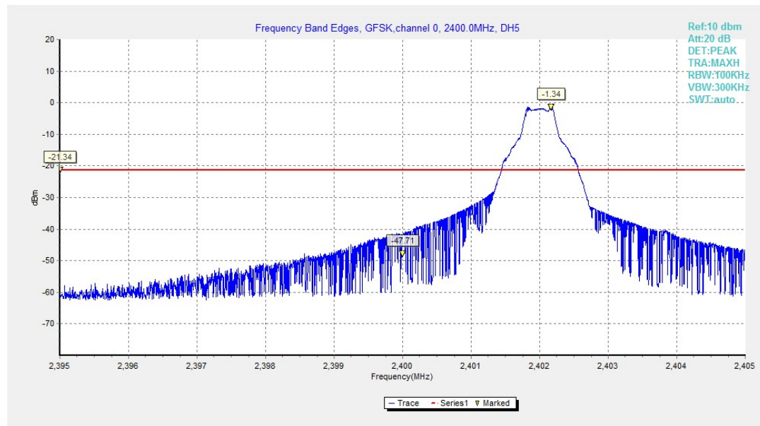
Fig.1. Frequency Band Edges: GFSK, Channel 0, Hopping Off
