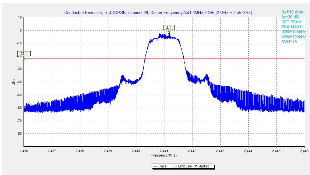
Fig.33. Conducted spurious emission: \pi/4 DQPSK, Channel 39, 2441MHz
