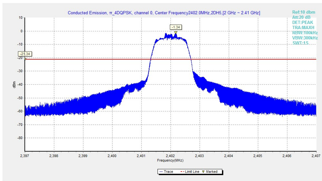
Fig.28. Conducted spurious emission: \pi/4 DQPSK, Channel 0, 2402MHz
