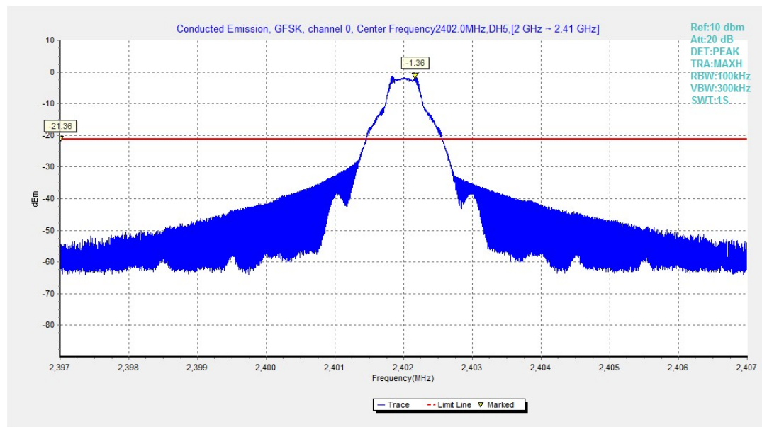
Fig.13. Conducted spurious emission: GFSK, Channel 0, 2402MHz
