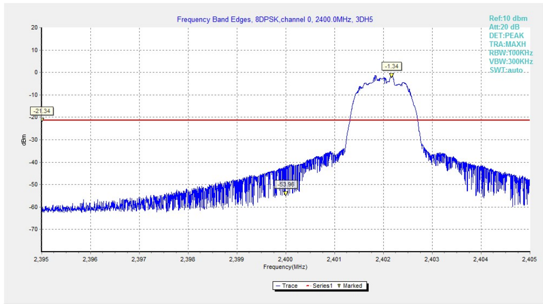
Fig.9. Frequency Band Edges: 8DPSK, Channel 0, Hopping Off
