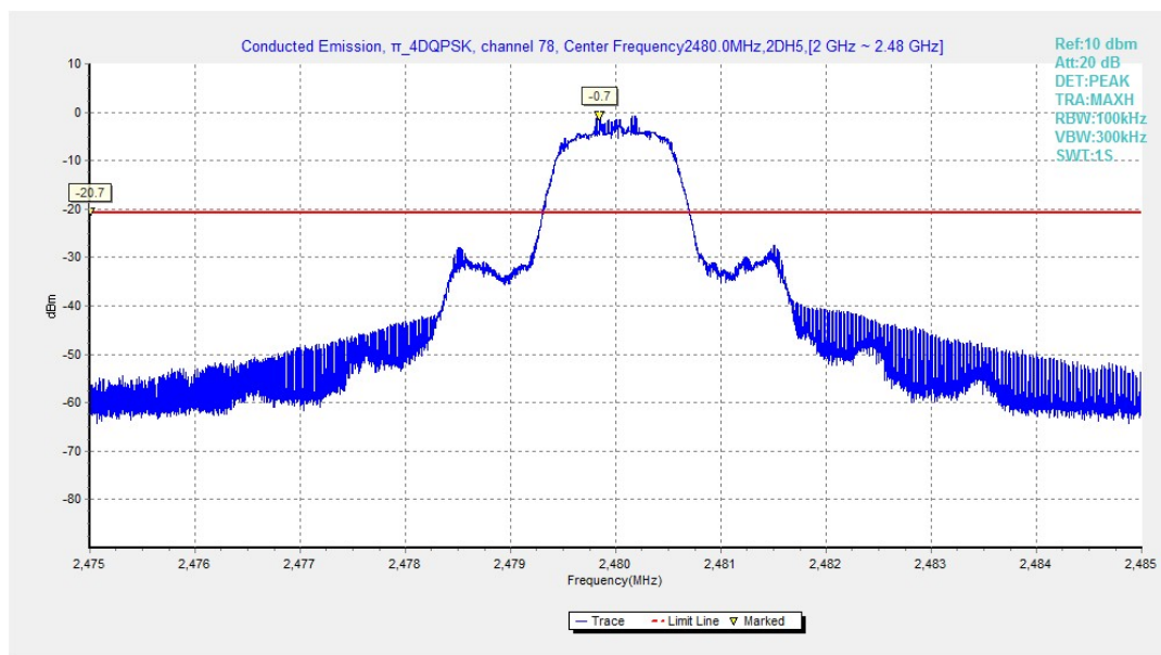
Fig.38. Conducted spurious emission: \pi/4 DQPSK, Channel 78, 2480MHz
