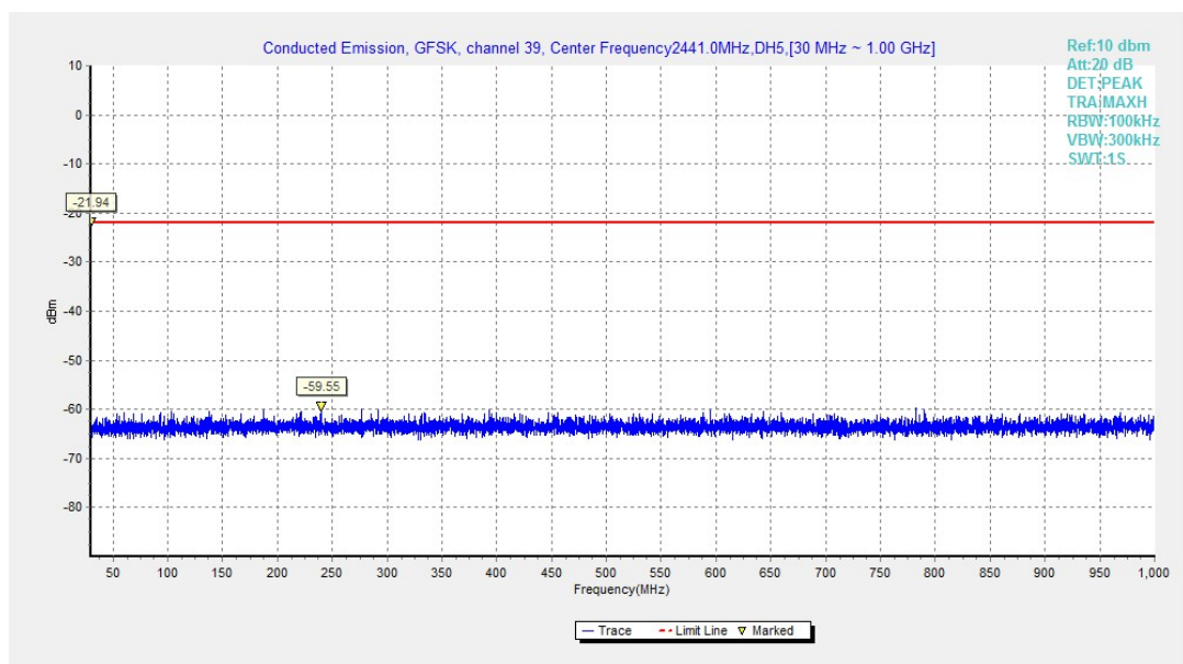
Fig.19. Conducted spurious emission: GFSK, Channel 39, 30MHz - 1GHz
