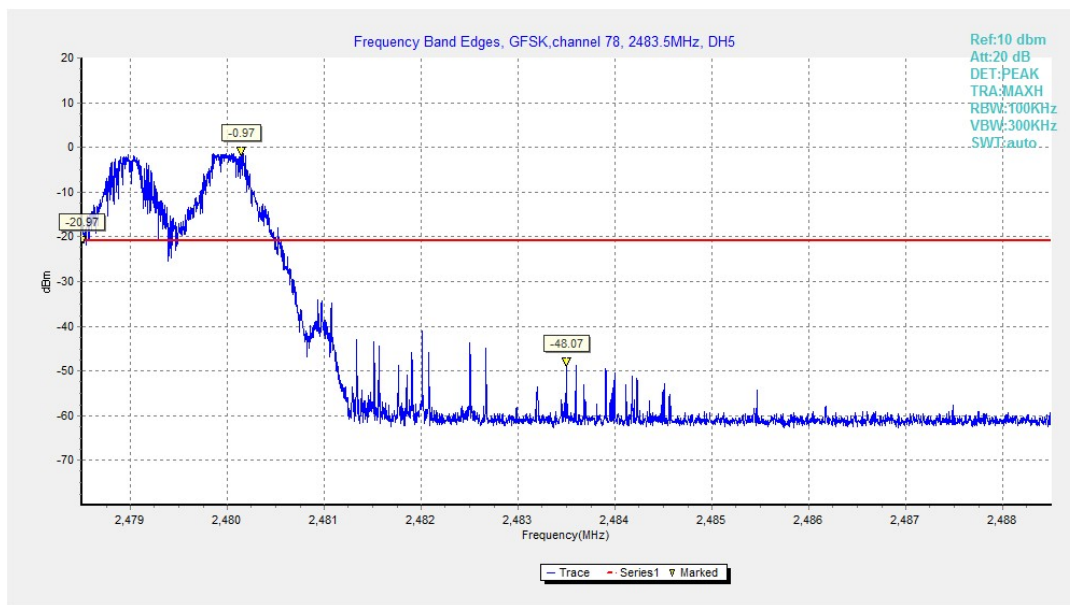
Fig.4. Frequency Band Edges: GFSK, Channel 78, Hopping On
