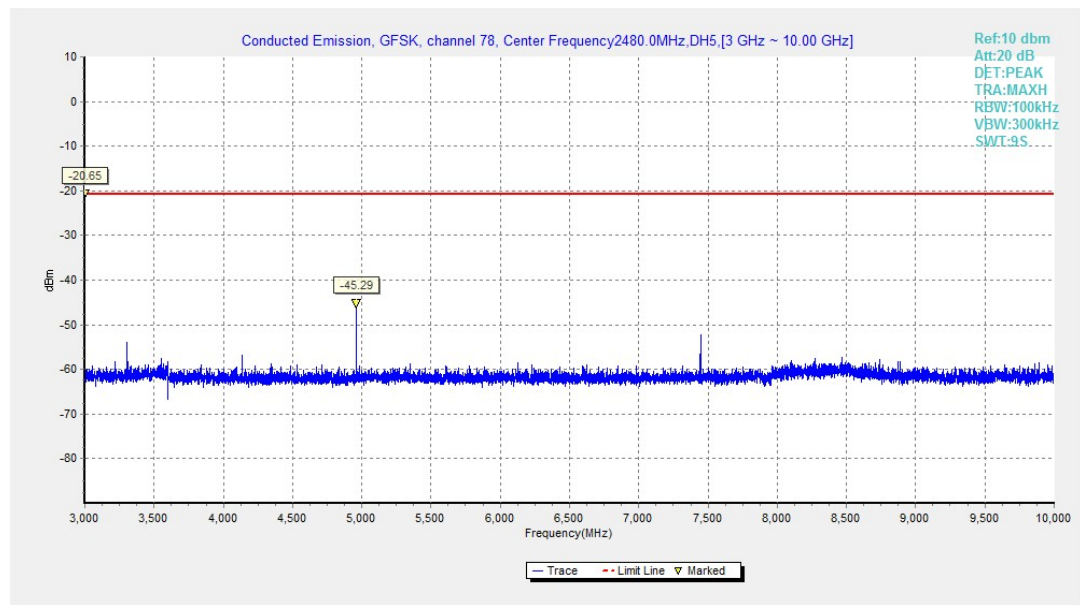
Fig.26. Conducted spurious emission: GFSK, Channel 78, 3GHz - 10GHz
