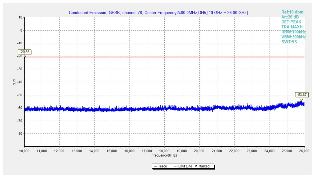
Fig.27. Conducted spurious emission: GFSK, Channel 78, 10GHz - 26GHz
