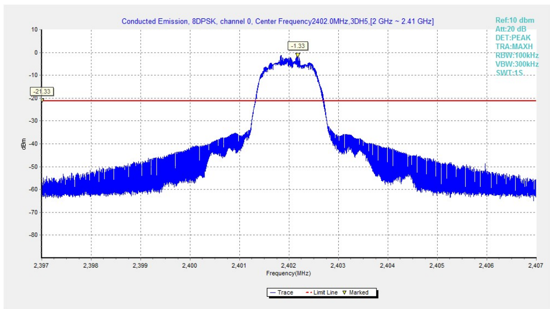
Fig.43. Conducted spurious emission: 8DPSK, Channel 0,2402MHz
