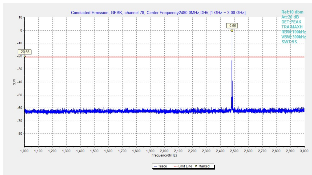
Fig.25. Conducted spurious emission: GFSK, Channel 78, 1GHz - 3GHz
