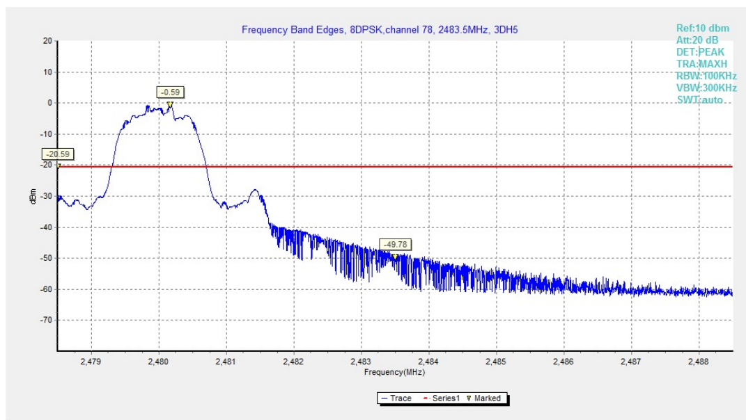
Fig.11. Frequency Band Edges: 8DPSK, Channel 78, Hopping Off
