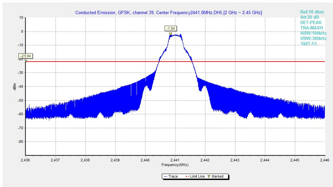
Fig.18. Conducted spurious emission: GFSK, Channel 39, 2441MHz
