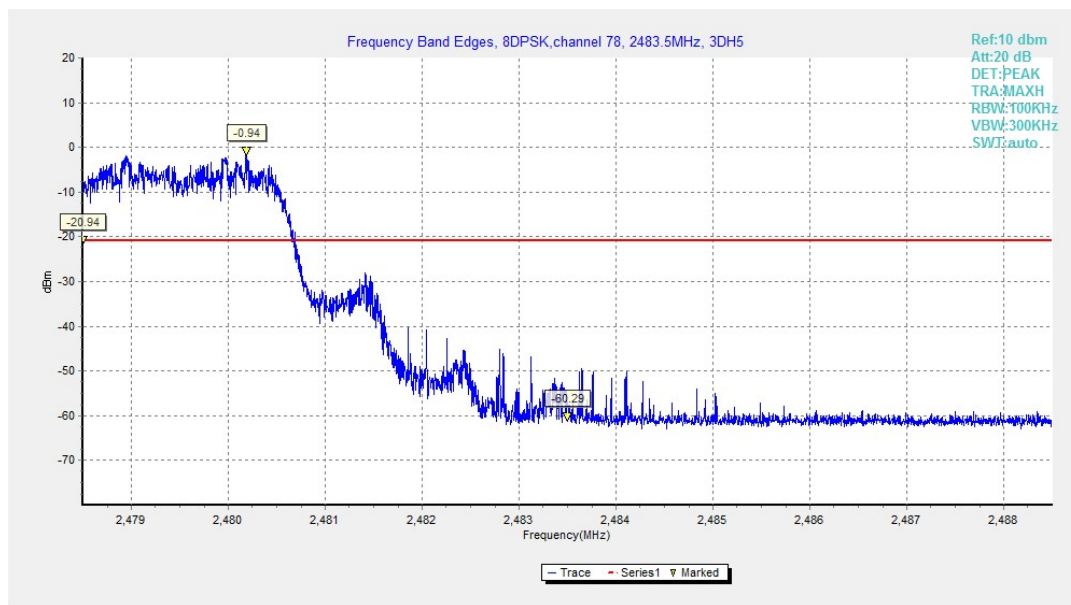
Fig.12. Frequency Band Edges: 8DPSK, Channel 78, Hopping On
