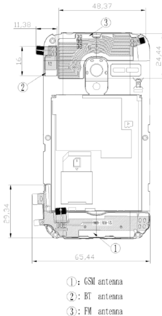
Picture 12.1 Antenna Locations
