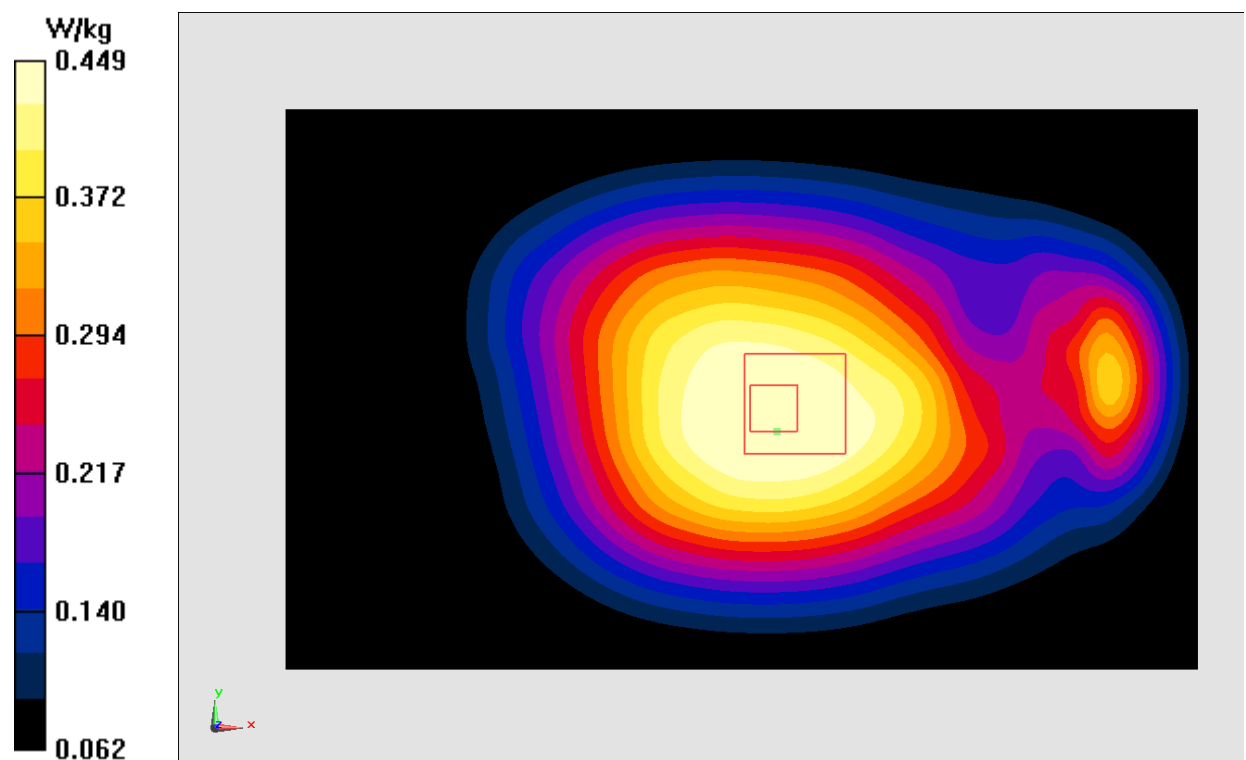
Fig.22 LTE Band5
