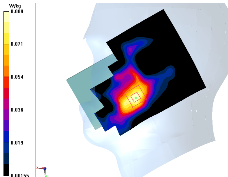
Fig.3 1900 MHz
