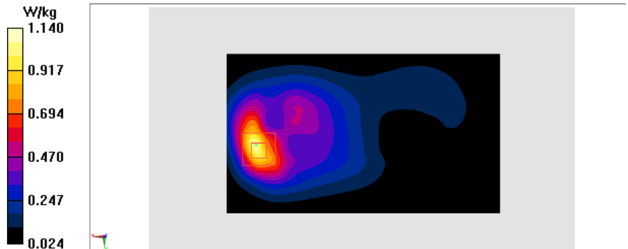
Fig.20 1700 MHz
