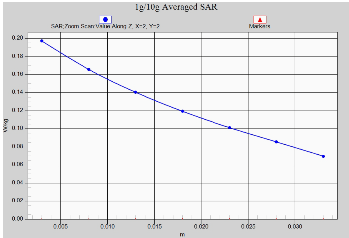
Fig. 23-1 Z-Scan at power reference point (LTE Band12)
