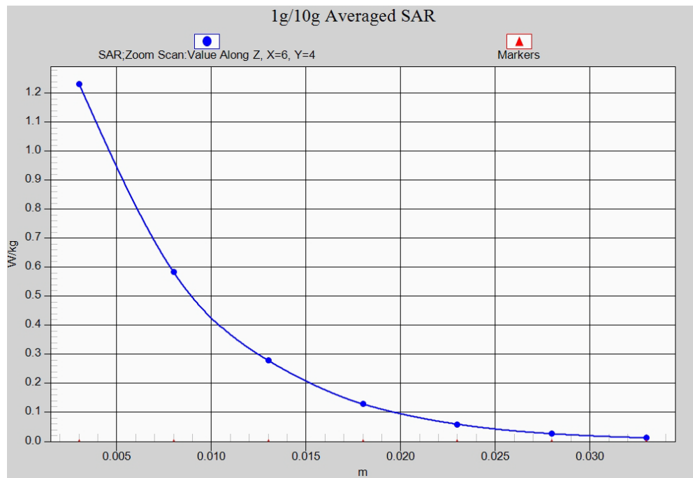
Fig. 19-1 Z-Scan at power reference point (LTE Band30)
