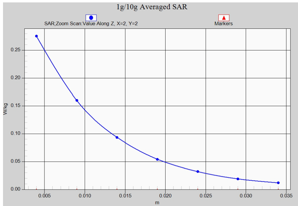
Fig. 21-1 Z-Scan at power reference point (LTE Band30)
