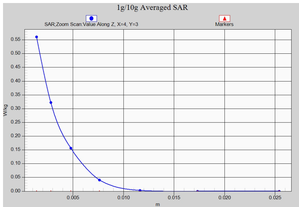
Fig. 29-1 Z-Scan at power reference point (5GHz)
