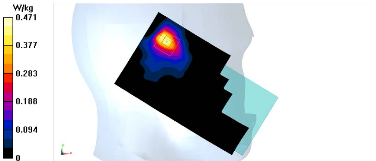
Fig.26 5GHz
