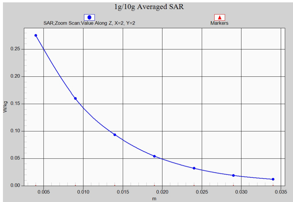
Fig. 20-1 Z-Scan at power reference point (LTE Band30)
