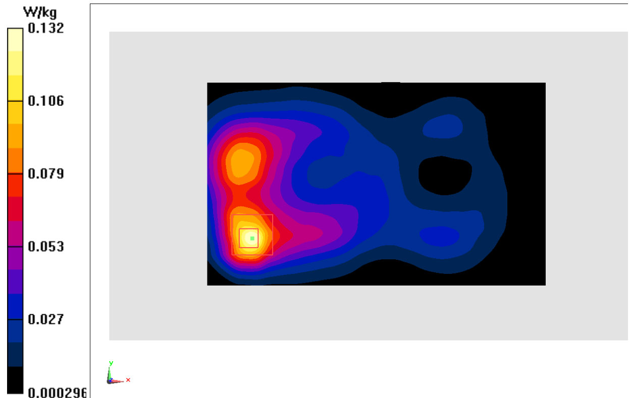
Fig.23 2450 MHz
