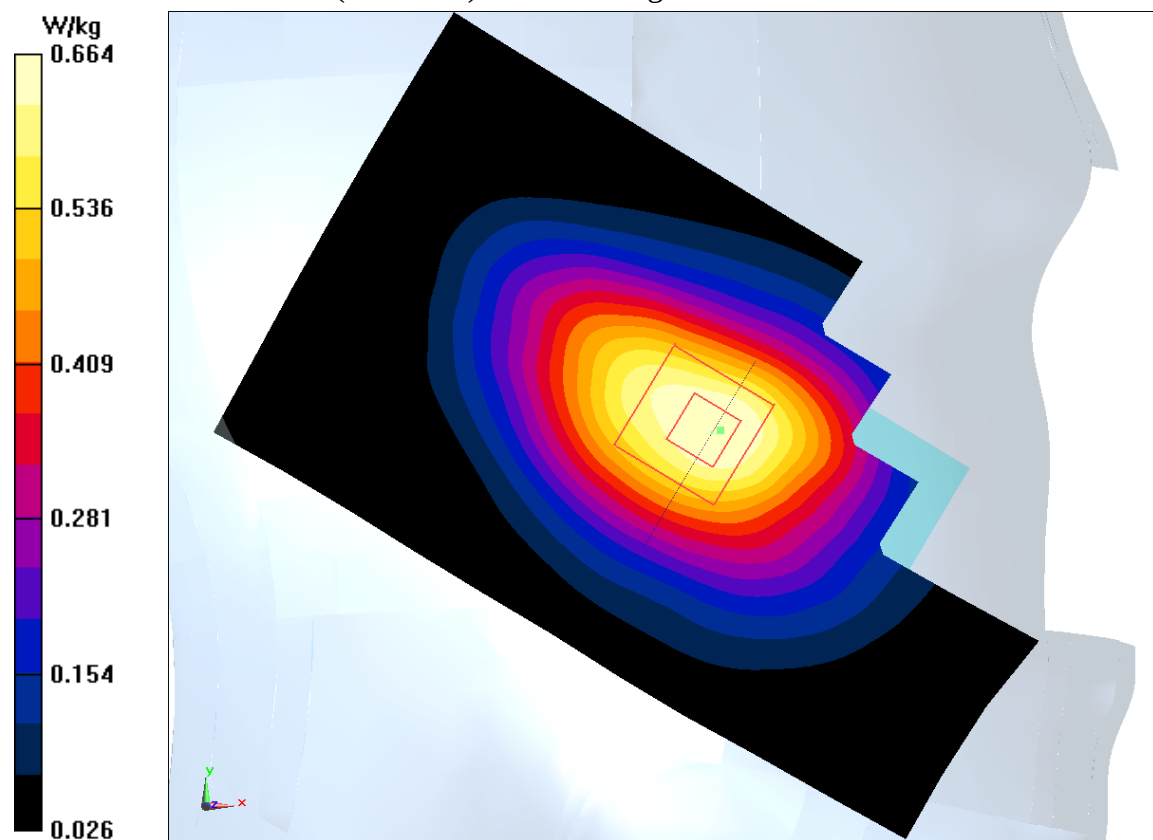
Fig.1 850MHz
