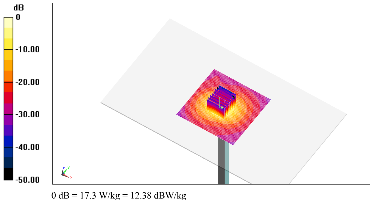
Fig.B.16 validation 5250MHz 100mW
