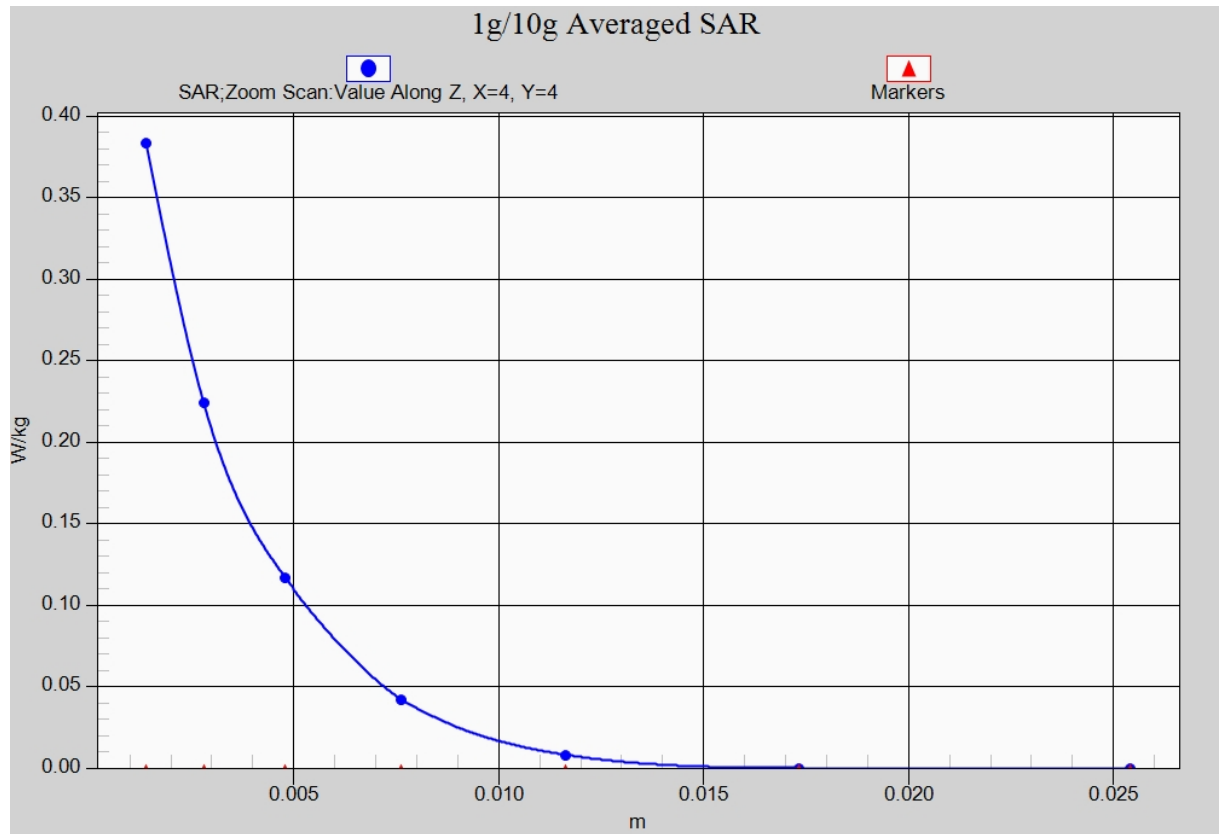
Fig. 37-1 Z-Scan at power reference point (5GHz)
