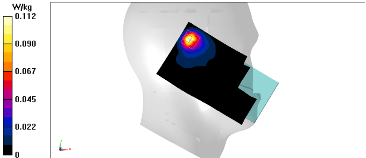
Fig.35 2450 MHz
