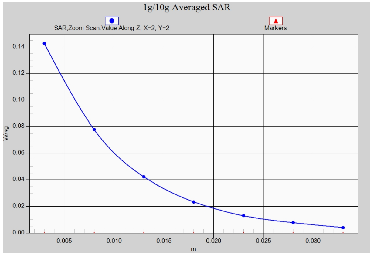
Fig. 32-1 Z-Scan at power reference point (LTE Band30)
