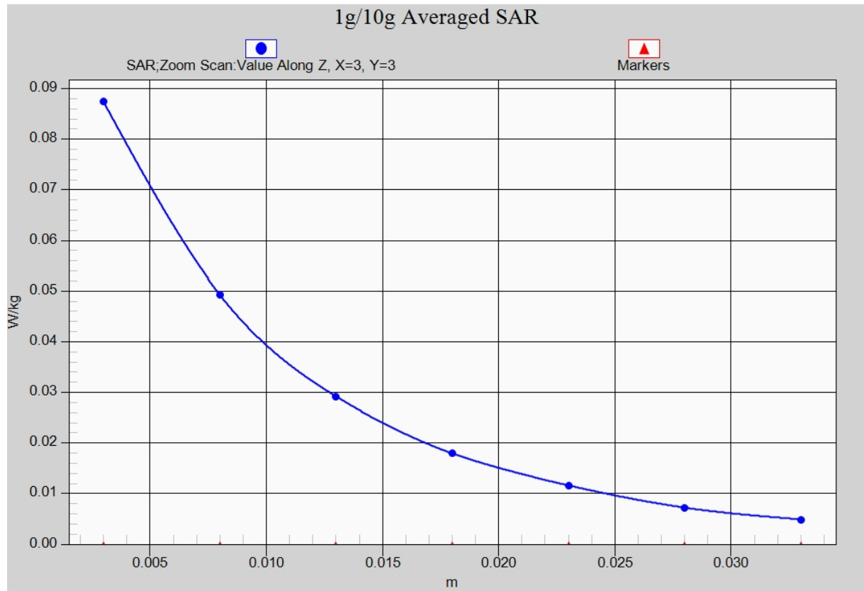
Fig. 31-1 Z-Scan at power reference point (LTE Band30)
