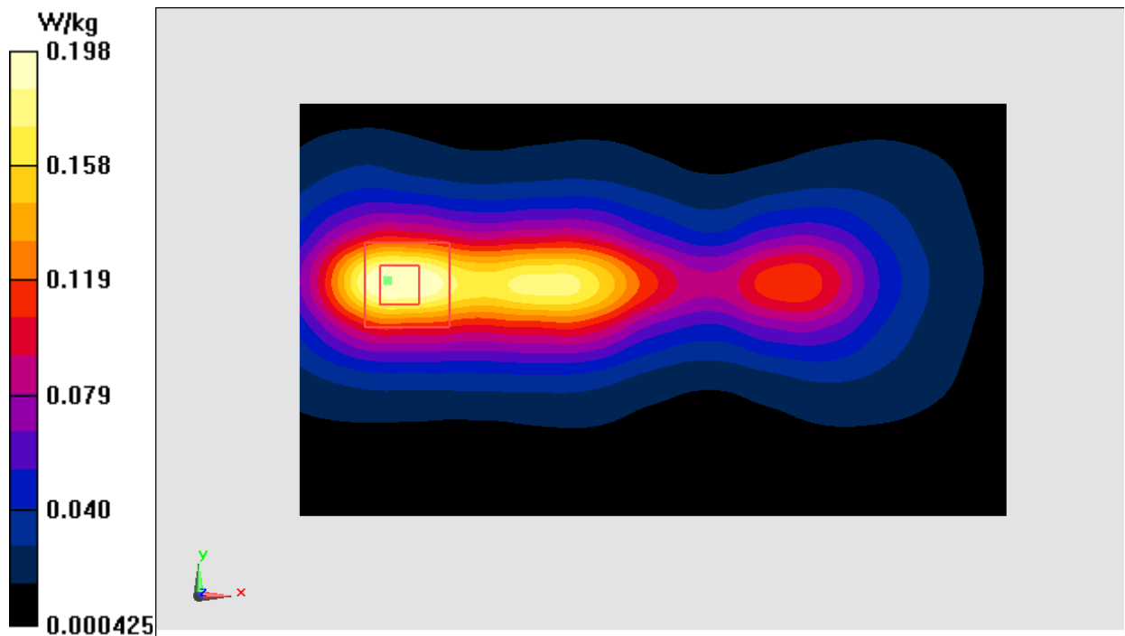
Fig.34 2450 MHz
