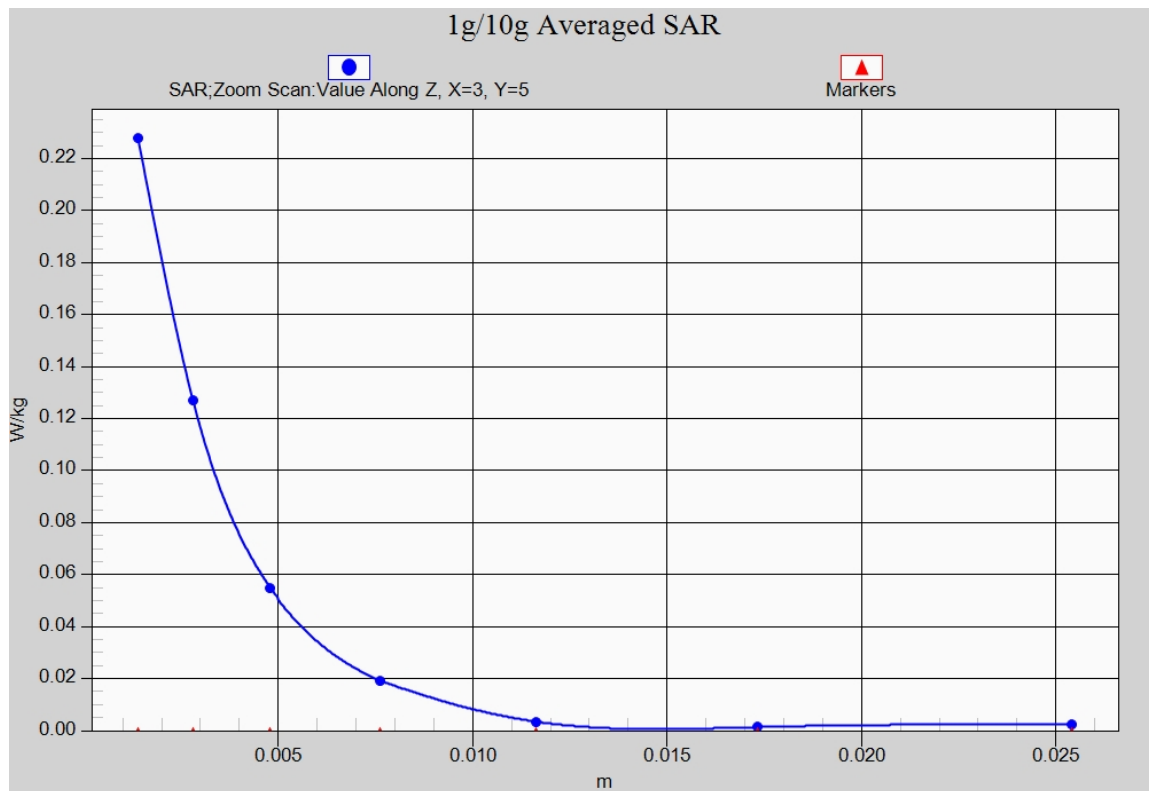
Fig. 38-1 Z-Scan at power reference point (5GHz)
