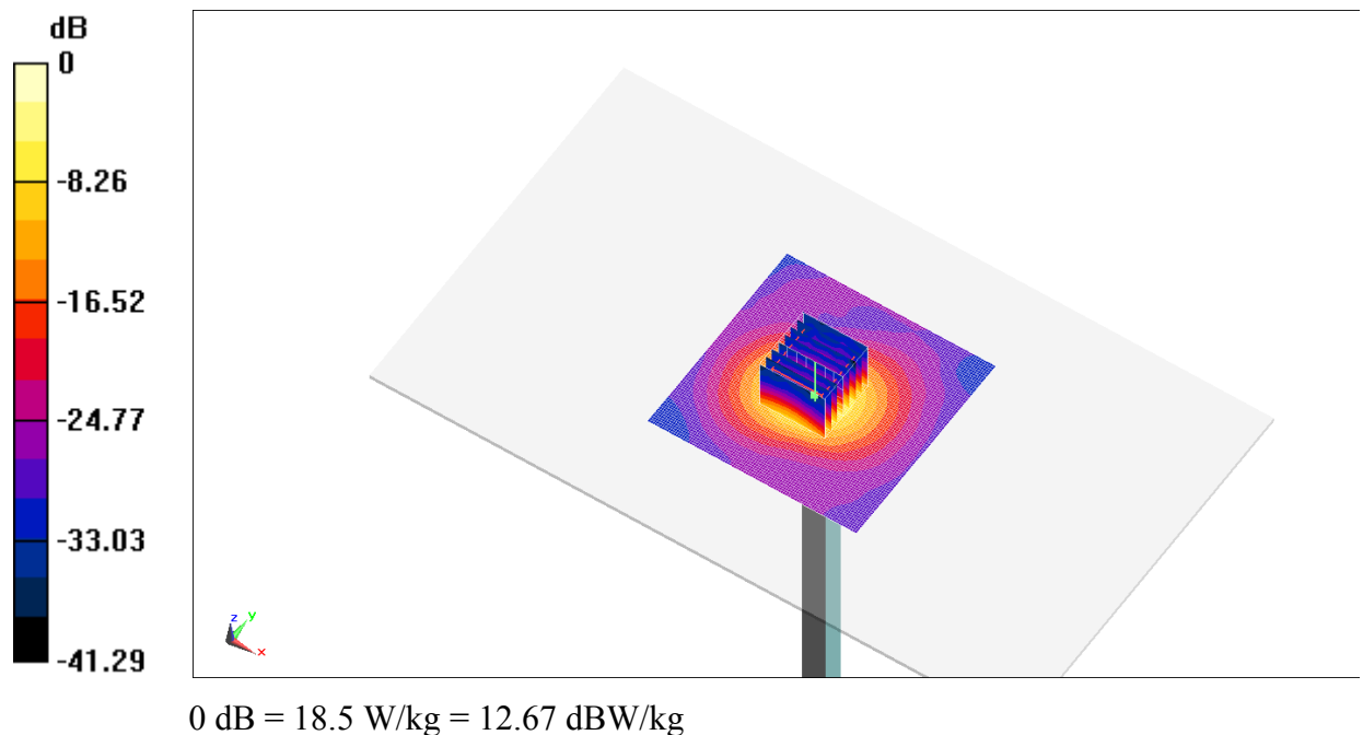
Fig.B.18 validation 5600MHz 100mW
