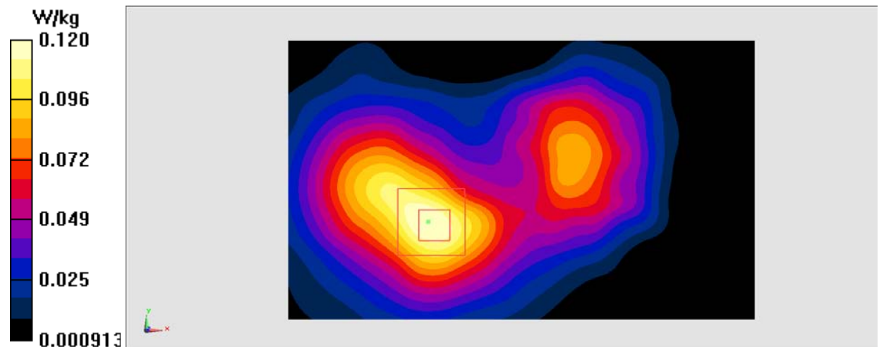
Fig.10 2450 MHz
