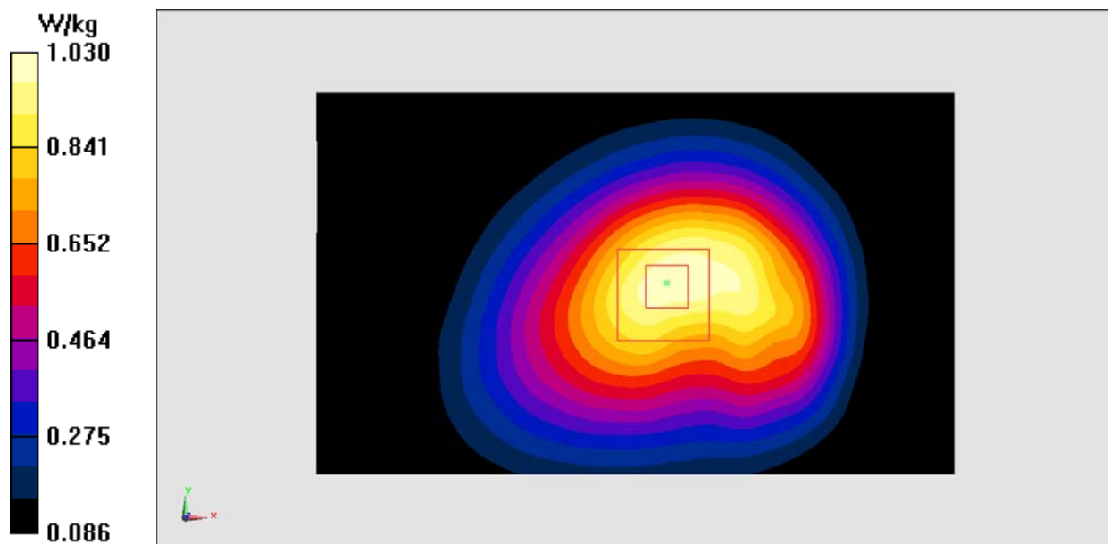
Fig.8 LTE Band 13
