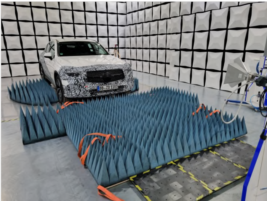
Photograph 2: EUT test setup for measurement > 1 GHz in the anechoic chamber, overview
