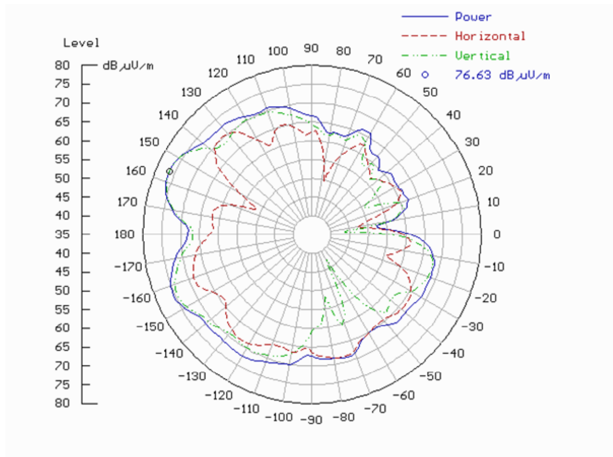
Fig. 9: Maximum EIRP value found for 434 MHz antenna when attached to real car in worst case scenario and when set to appropriate modulation, timing and power value 0x2D.
