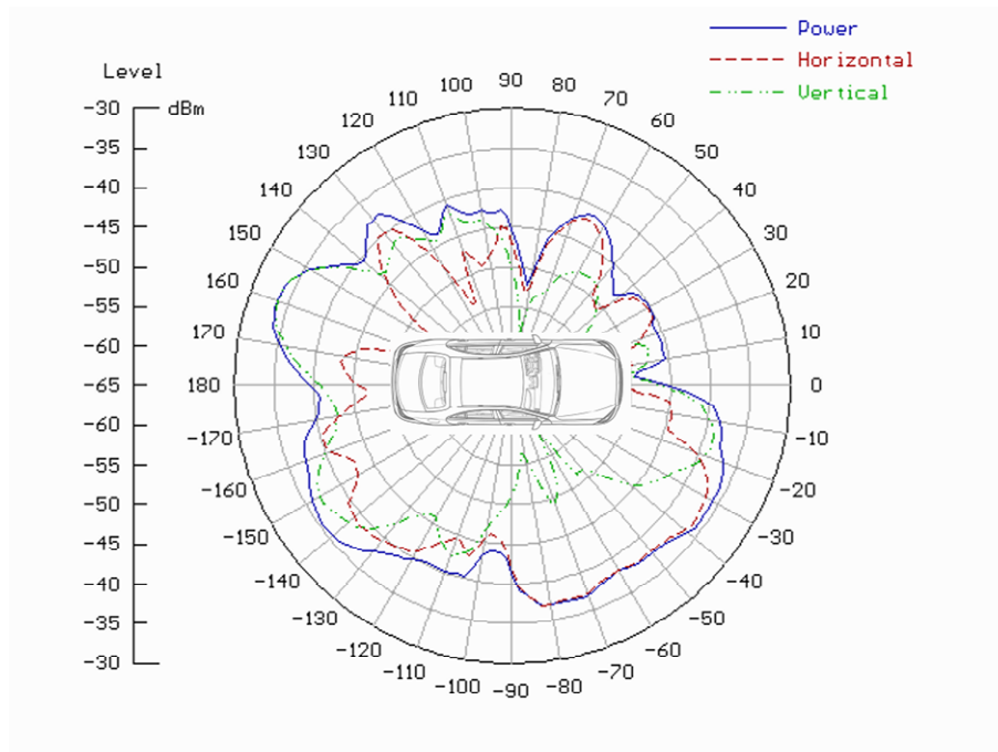
Fig. 7: Example pattern measured at 434 MHz from ANT1 with the installed module BASE (raw data for measurement antenna at 1 m height).
