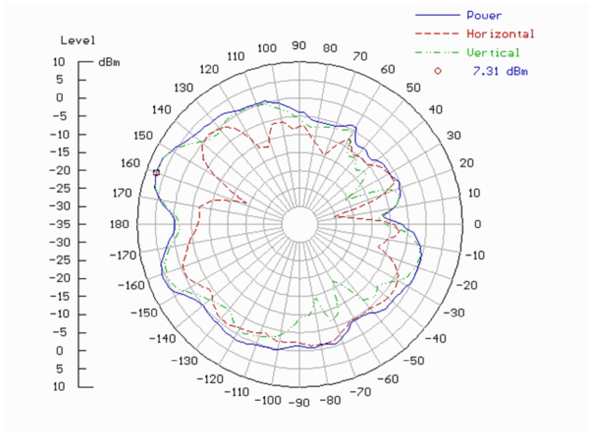
Fig. 10: Maxim EIRP value found for 434 MHz antenna when attached to real car in a worst case scenario and when set to appropriate modulation, and power value 0x34.
