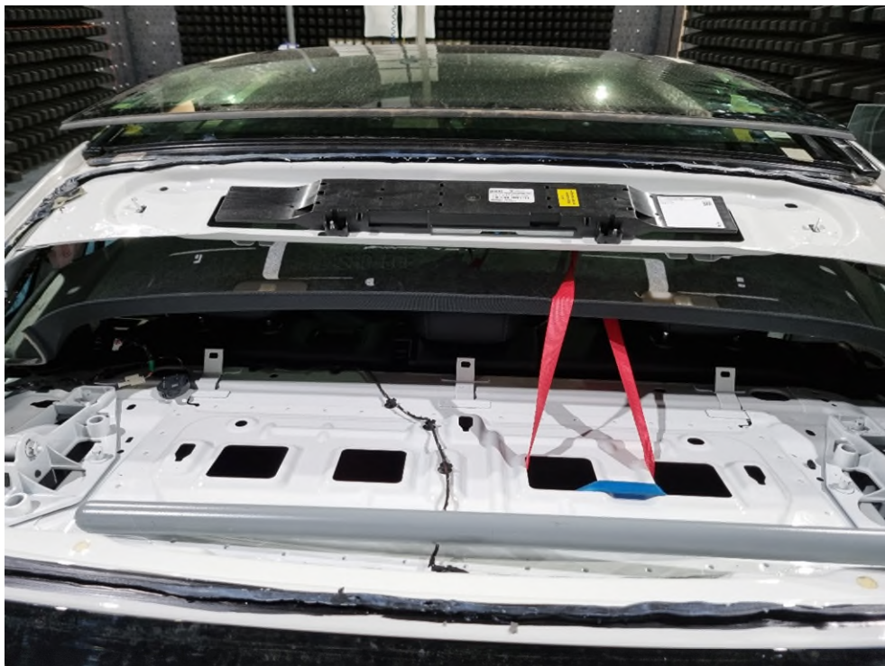
Fig. 6: EUT support details: set up when measuring the real antenna installed at the car (but cover removed).
