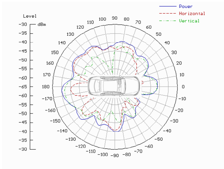
Fig. 8: Example pattern measured at 434 MHz from ANT2 with the installed module BASE (raw data for measurement antenna at 2.5 m height).
