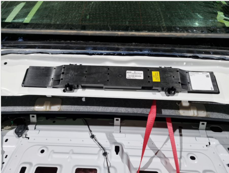
Photograph 3: AE 2 (Antenna placement)
