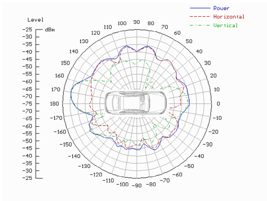
Fig. 8: Example pattern measured at 434 MHz from ANT2 with the installed module BASE (raw data for measurement antenna at 1.0 m height).
