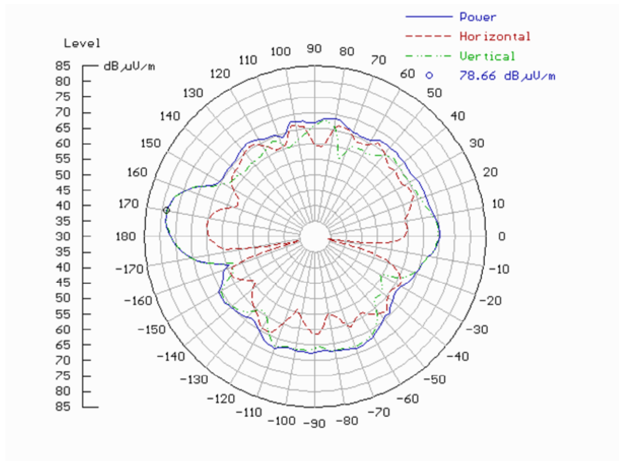
Fig. 9: Maximum field strength value found for 434 MHz antenna when attached to real car in worst case scenario and when set to appropriate modulation, timing and power value (Hex 0x30).
