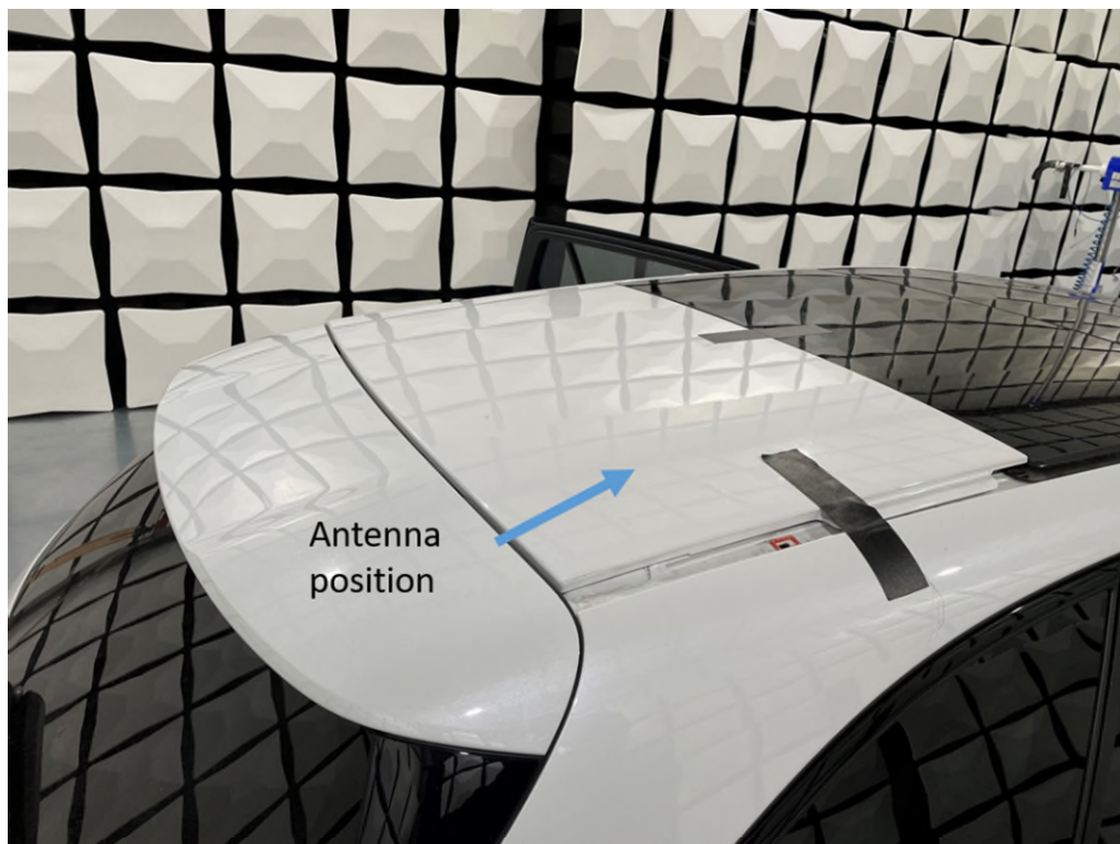
Fig. 3: Photo and indication of antenna position.
