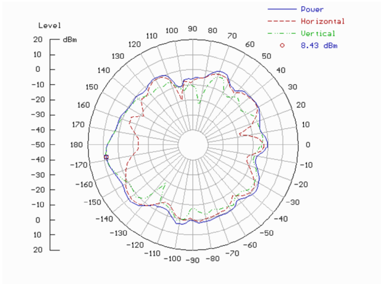
Fig. 10: Maxim EIRP value found for 434 MHz antenna when attached to real car in a worst case scenario and when set to appropriate modulation, and power value (Hex 0x37).
