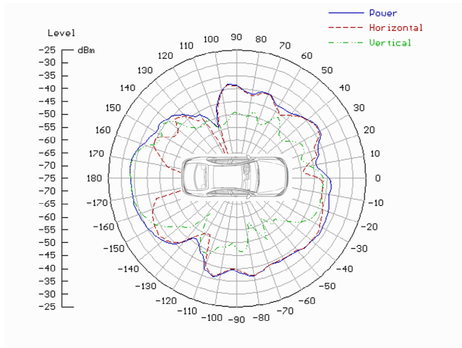
Fig. 7: Example pattern measured at 434 MHz from ANT1 with the installed module BASE (raw data for measurement antenna at 1.0 m height).
