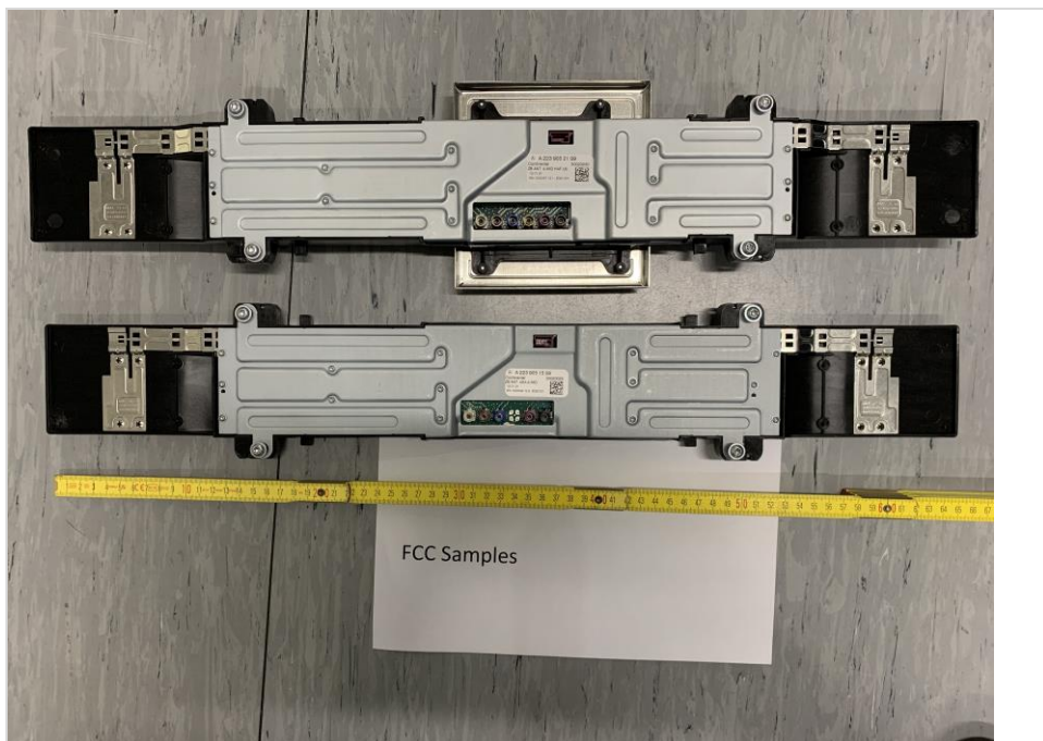
Photograph 2: EUT 1_Rear side view - EUT 1 (upper) and EUT 2 (lower)
