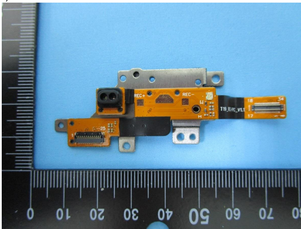
(22) EUT Photo
