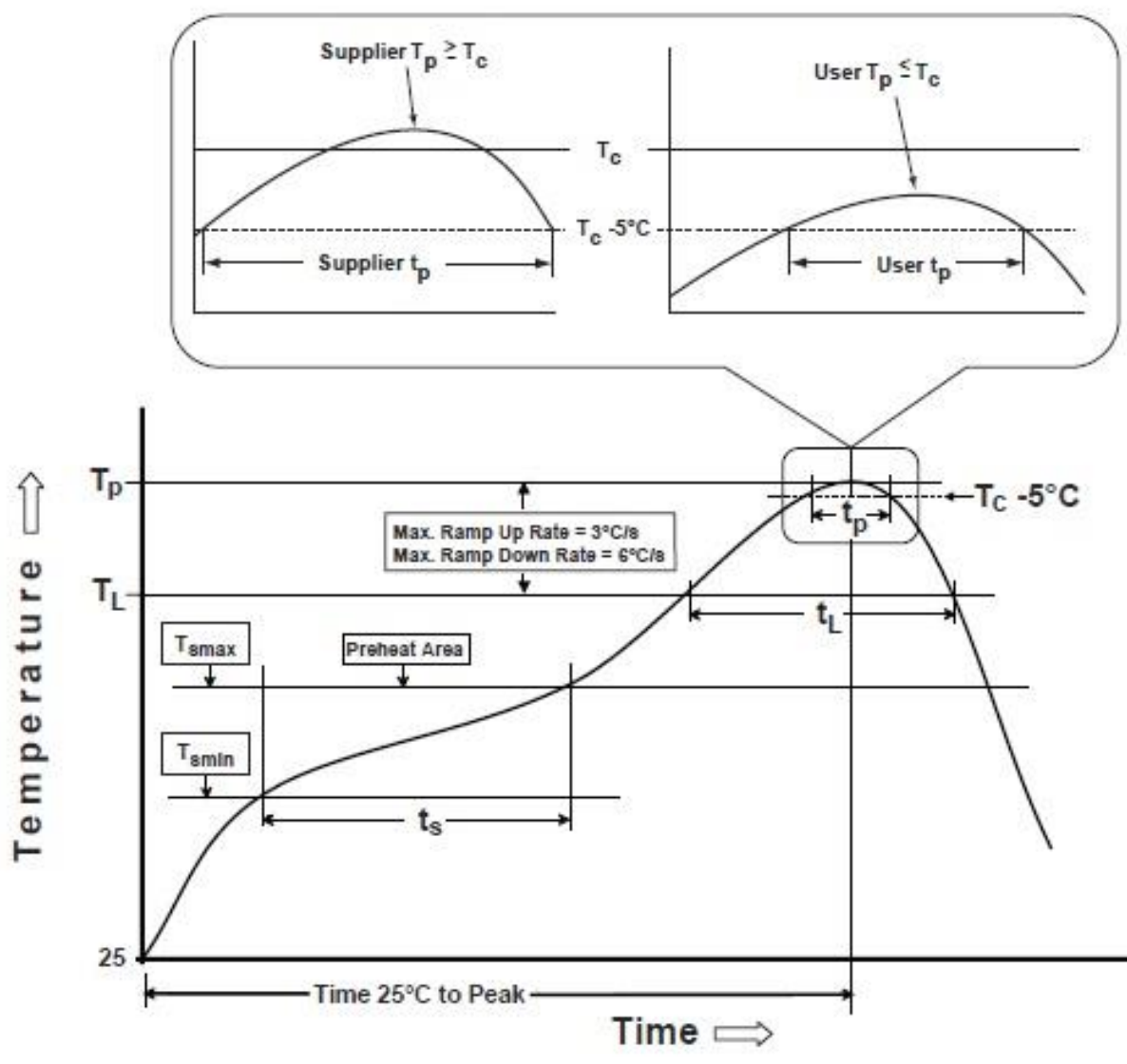
Figure 11: Classification Reflow Profile (not to scale) [12]
