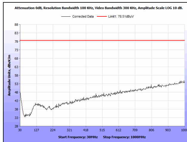
Plot 37. Radiated Spurious Emissions, 20 dBc, 30 MHz – 1 GHz, Mid Channel
