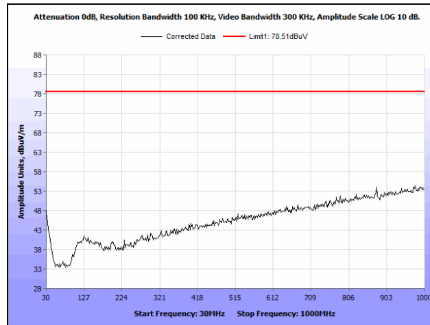
Plot 40. Radiated Spurious Emissions, 20 dBc, 30 MHz – 1 GHz, High Channel
