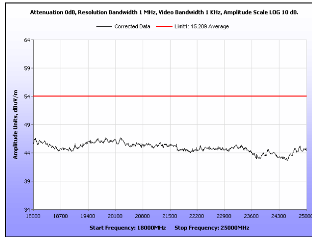
Plot 22. Radiated Spurious Emissions, Low Channel, 18 GHz – 25 GHz, Average
