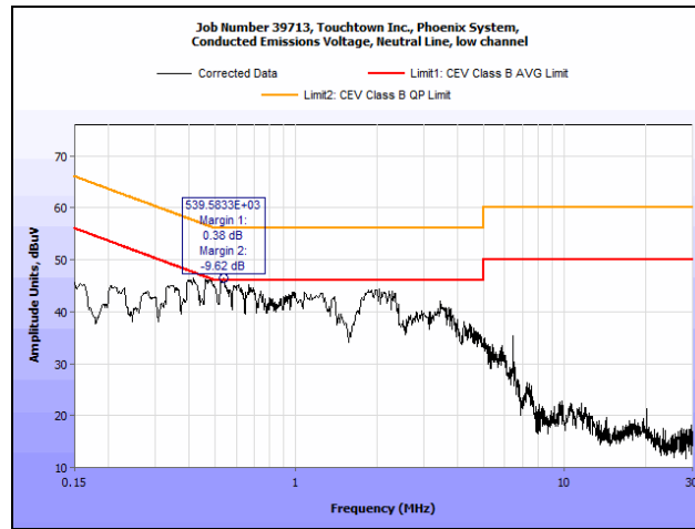
Plot 7. Conducted Emissions, 15.207(a), Neutral Line, Low Channel
