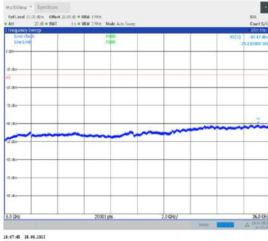
1-N77-3450-3550--30-100-M-1-DFT-QPSK- Edge_1RB_Left-1@0-6000-26000-Ant2--40.47--13- PASS
