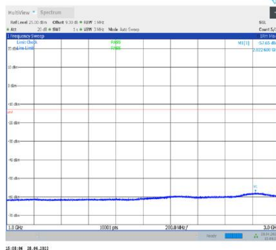
1-N77-3450-3550--30-100-L-1-DFT-QPSK- Edge_1RB_Left-1@0-1000-3000-Ant1--57.65--13- PASS
