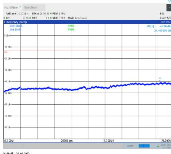
1-N77-3450-3550--30-100-H-1-DFT-QPSK- Edge_1RB_Left-1@0-6000-26000-Ant2--40.38--13- PASS
