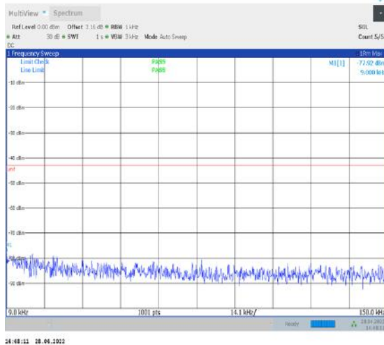
1-N77-3450-3550--30-100-H-1-DFT-QPSK- Edge_1RB_Left-1@0-0.009-0.15-Ant2--77.92--43- PASS
