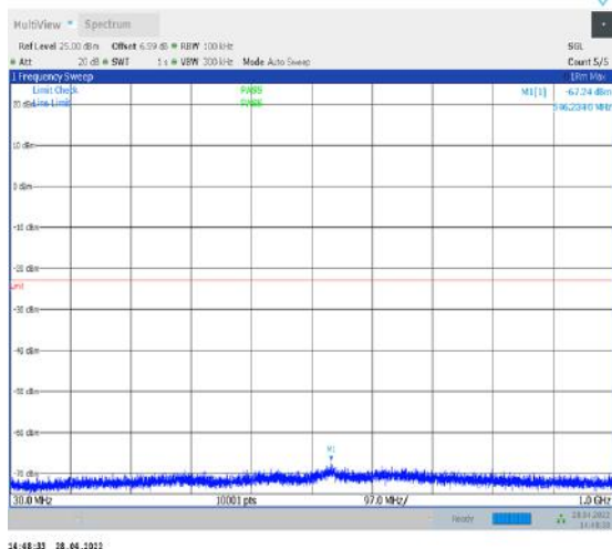
1-N77-3450-3550--30-100-H-1-DFT-QPSK- Edge_1RB_Left-1@0-30-1000-Ant2--67.24--23- PASS
