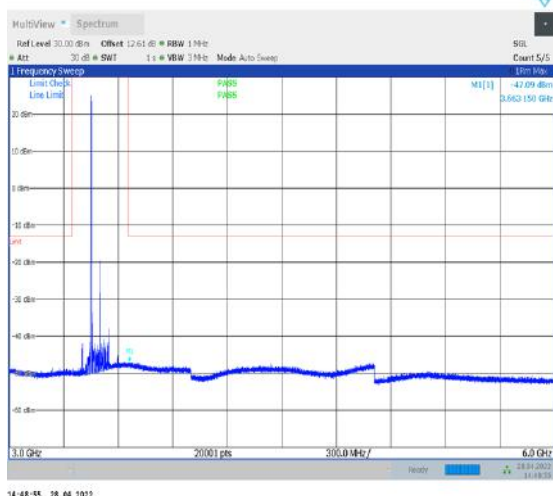
1-N77-3450-3550--30-100-H-1-DFT-QPSK- Edge_1RB_Left-1@0-3000-6000-Ant2--47.09--13- PASS
