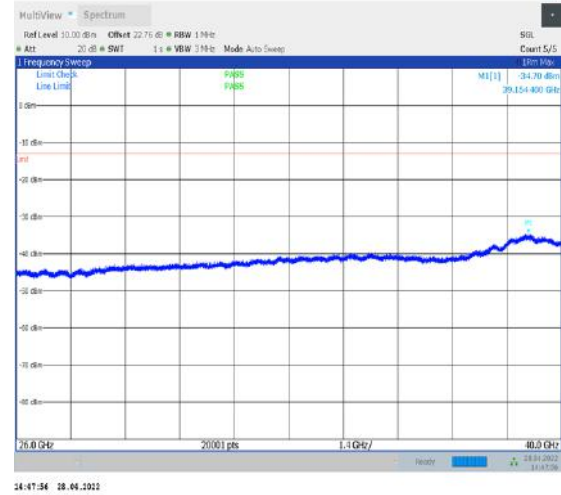
1-N77-3450-3550--30-100-M-1-DFT-QPSK- Edge_1RB_Left-1@0-26000-40000-Ant2--34.70--13- PASS
