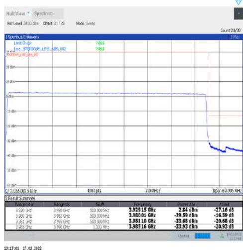
1-N77-3700-3980-30-60-H-6-CP-QPSK-Outer_Full-162@0-Ant1-PASS-see graph
