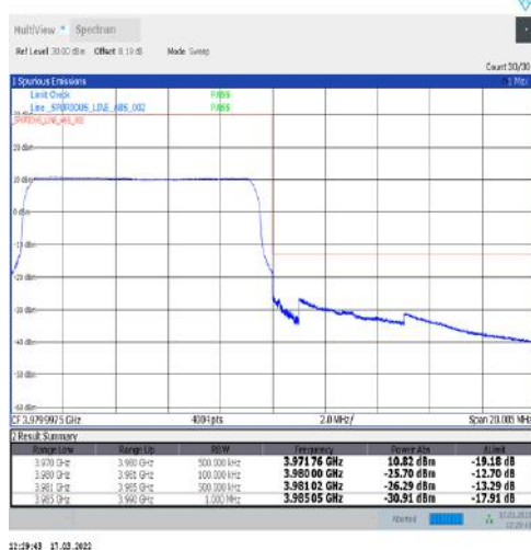
1-N77-3700-3980-30-10-H-6-CP-QPSK-Outer_Full-24@0-Ant1-PASS-see graph
