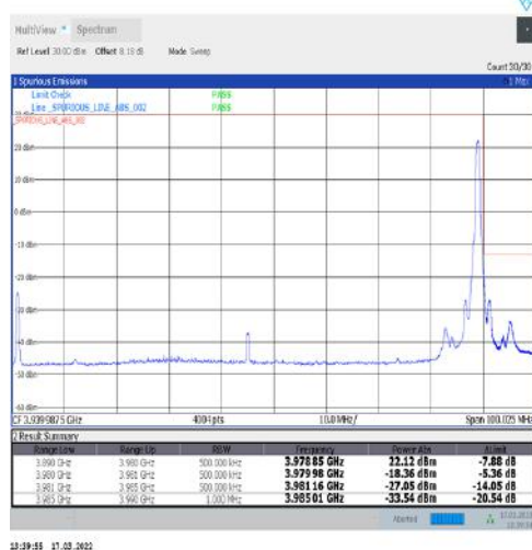
1-N77-3700-3980-30-90-H-5-CP-QPSK-Edge_1RB_Right-1@244-Ant1-PASS-see graph
