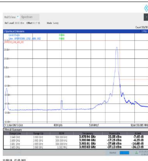
1-N77-3700-3980-30-40-H-2-DFT-PI2BPSK-Edge_1RB_Right-1@105-Ant1-PASS-see graph
