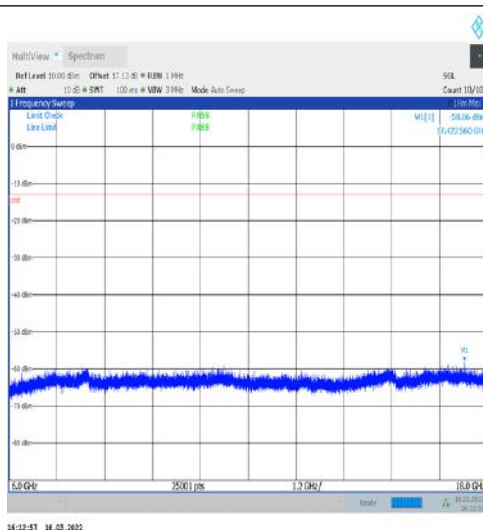
1-N77-3700-3980-30-100-L-1-DFT-PI2BPSK- Inner_1RB_Left-1@1-6000-18000-Ant1--58.06--13- PASS
