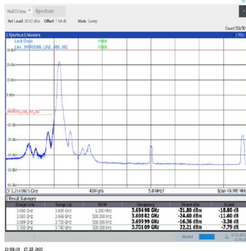
1-N77-3700-3980-30-40-L-4-CP-QPSK-Edge_1RB_Left-1@0-Ant1-PASS-see graph
