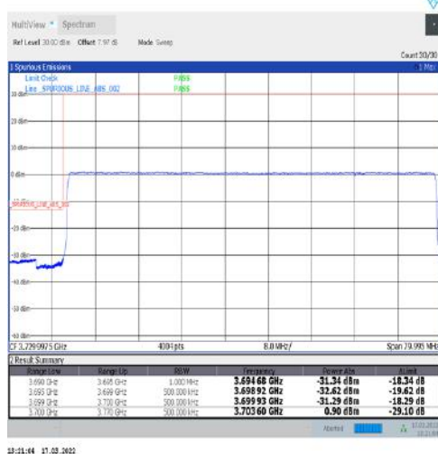
1-N77-3700-3980-30-70-L-6-CP-QPSK-Outer_Full-189@0-Ant1-PASS-see graph
