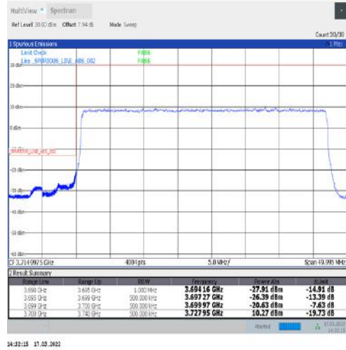
1-N77-3700-3980-30-40-L-3-DFT-PI2BPSK-Outer_Full-100@0-Ant1-PASS-see graph
