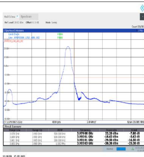
1-N77-3700-3980-30-10-H-2-DFT-PI2BPSK-Edge_1RB_Right-1@23-Ant1-PASS-see graph
