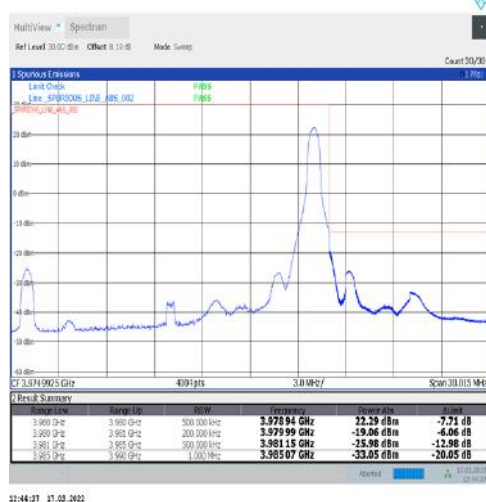
1-N77-3700-3980-30-20-H-5-CP-QPSK-Edge_1RB_Right-1@50-Ant1-PASS-see graph
