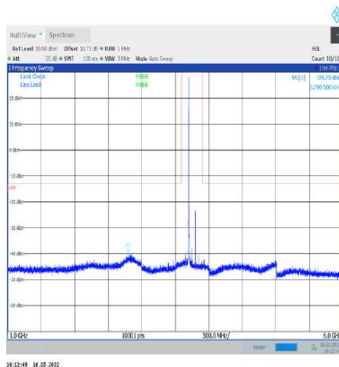
1-N77-3700-3980-30-100-L-1-DFT-PI2BPSK- Inner_1RB_Left-1@1-1000-6000-Ant1--39.73--13- PASS
