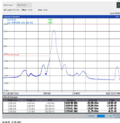
1-N77-3700-3980-30-15-L-4-CP-QPSK-Edge_1RB_Left-1@0-Ant1-PASS-see graph
