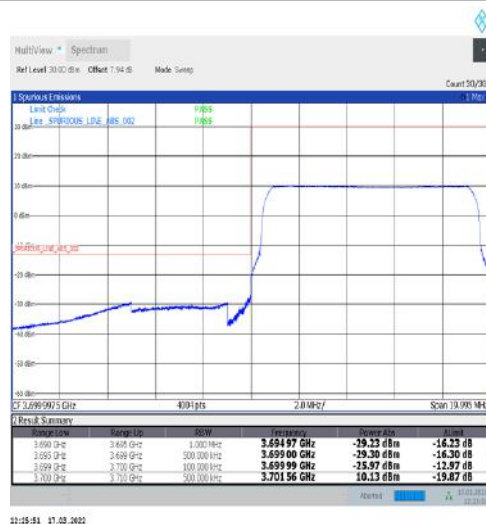
1-N77-3700-3980-30-10-L-6-CP-QPSK-Outer_Full-24@0-Ant1-PASS-see graph
