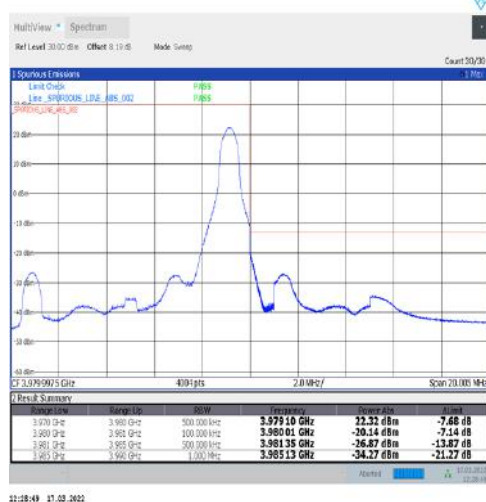
1-N77-3700-3980-30-10-H-5-CP-QPSK-Edge_1RB_Right-1@23-Ant1-PASS-see graph
