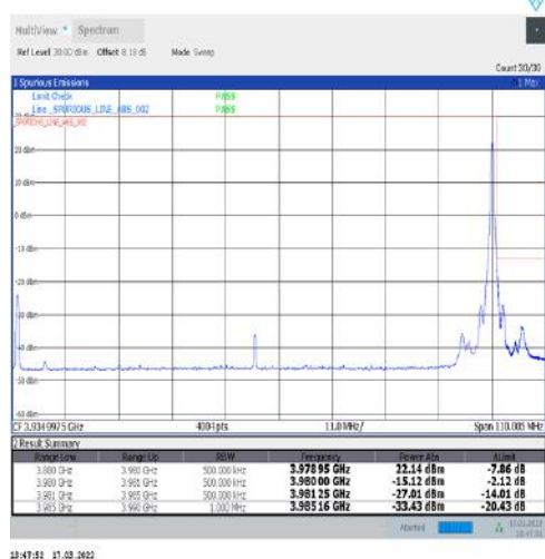
1-N77-3700-3980-30-100-H-5-CP-QPSK-Edge_1RB_Right-1@272-Ant1-PASS-see graph
