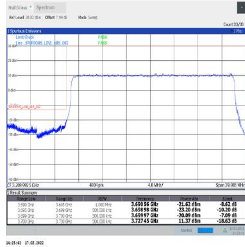
1-N77-3700-3980-30-30-L-3-DFT-PI2BPSK-Outer_Full-75@0-Ant1-PASS-see graph
