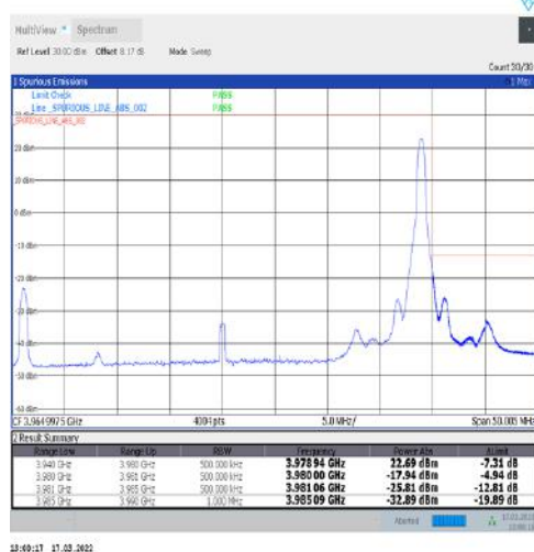
1-N77-3700-3980-30-40-H-5-CP-QPSK-Edge_1RB_Right-1@105-Ant1-PASS-see graph
