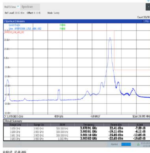
1-N77-3700-3980-30-30-H-5-CP-QPSK-Edge_1RB_Right-1@77-Ant1-PASS-see graph
