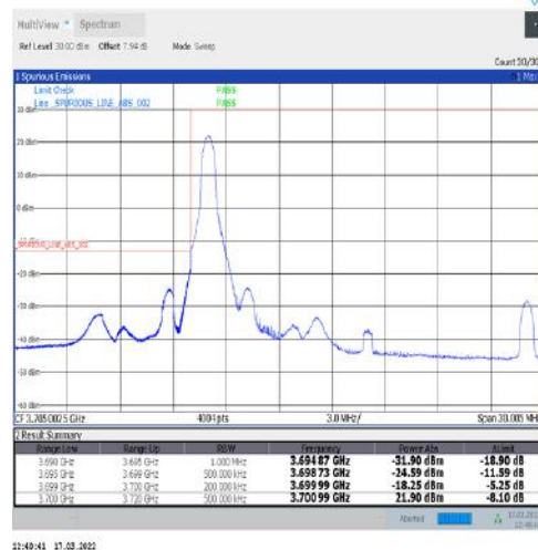
1-N77-3700-3980-30-20-L-4-CP-QPSK-Edge_1RB_Left-1@0-Ant1-PASS-see graph
