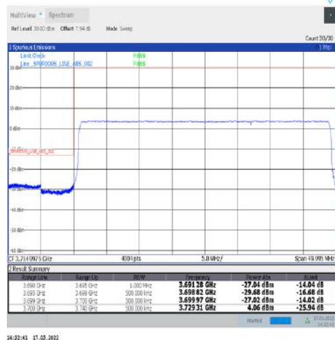
1-N77-3700-3980-30-40-L-6-CP-QPSK-Outer_Full-106@0-Ant1-PASS-see graph
