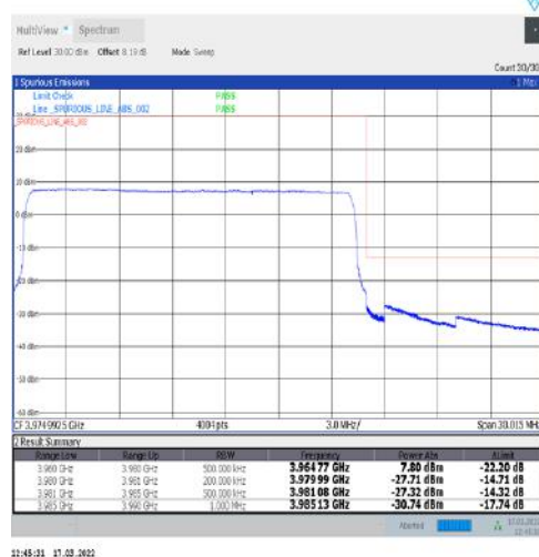
1-N77-3700-3980-30-20-H-6-CP-QPSK-Outer_Full-51@0-Ant1-PASS-see graph
