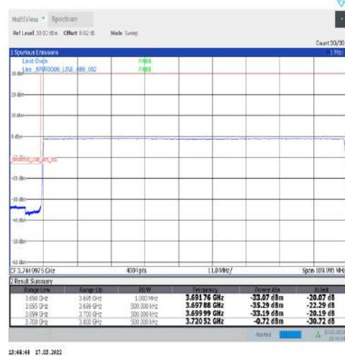
1-N77-3700-3980-30-100-L-6-CP-QPSK-Outer_Full-273@0-Ant1-PASS-see graph
