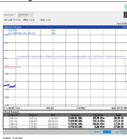
1-N77-3700-3980-30-90-L-3-DFT-PI2BPSK-Outer_Full-240@0-Ant1-PASS-see graph
