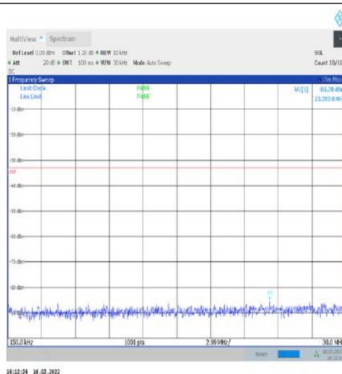
1-N77-3700-3980-30-100-L-1-DFT-PI2BPSK- Inner_1RB_Left-1@1-0.15-30-Ant1--85.28--33-PASS
