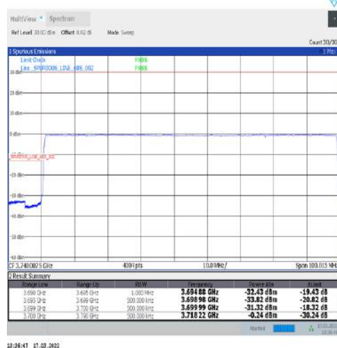
1-N77-3700-3980-30-90-L-6-CP-QPSK-Outer_Full-245@0-Ant1-PASS-see graph
