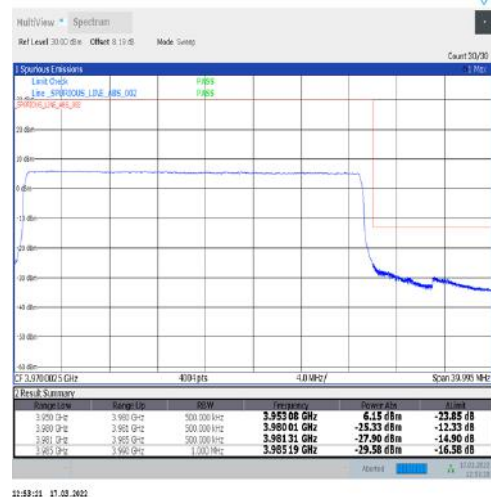
1-N77-3700-3980-30-30-H-6-CP-QPSK-Outer_Full-78@0-Ant1-PASS-see graph
