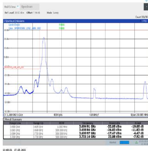
1-N77-3700-3980-30-30-L-4-CP-QPSK-Edge_1RB_Left-1@0-Ant1-PASS-see graph
