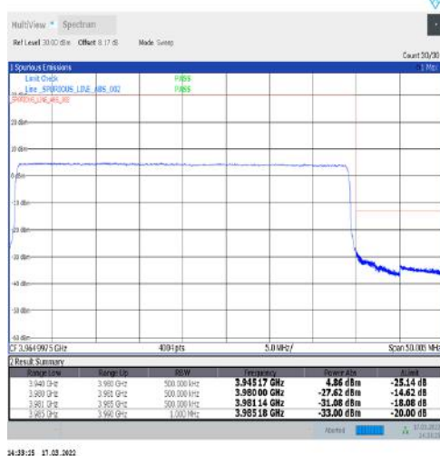
1-N77-3700-3980-30-40-H-6-CP-QPSK-Outer_Full-106@0-Ant1-PASS-see graph
