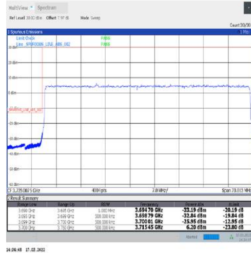
1-N77-3700-3980-30-60-L-3-DFT-PI2BPSK-Outer_Full-162@0-Ant1-PASS-see graph
