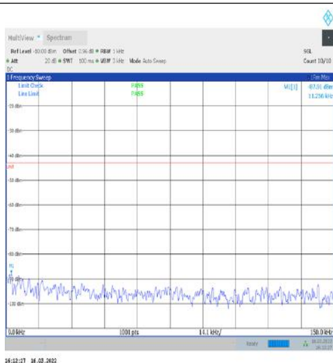
1-N77-3700-3980-30-100-L-1-DFT-PI2BPSK- Inner_1RB_Left-1@1-0.009-0.15-Ant1--87.91--43- PASS
