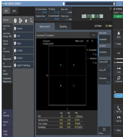
1-N77-3700-3980-30-100-M-1-DFT-PI2BPSK- Outer_Full-270@0-Ant1-see graph-PASS
