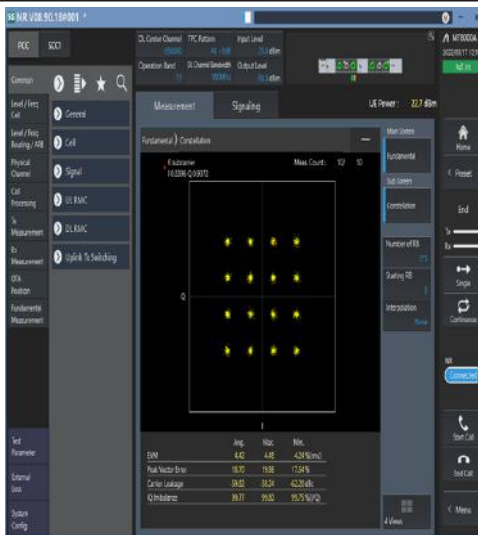
1-N77-3700-3980-30-100-M-7-CP-16QAM-Outer_Full-273@0-Ant1-see graph-PASS
