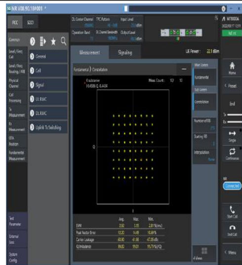
1-N77-3700-3980-30-100-M-8-CP-64QAM-Outer_Full-273@0-Ant1-see graph-PASS
