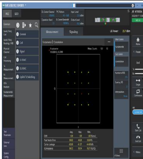
1-N77-3700-3980-30-100-M-3-DFT-16QAM- Outer_Full-270@0-Ant1-see graph-PASS
