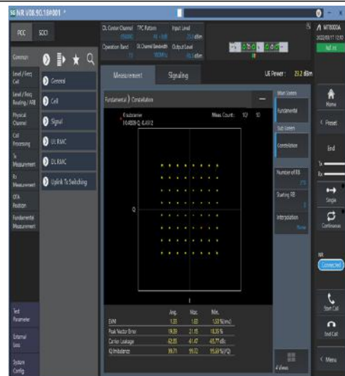
1-N77-3700-3980-30-100-M-4-DFT-64QAM- Outer_Full-270@0-Ant1-see graph-PASS
