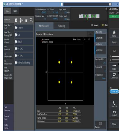
1-N77-3700-3980-30-100-M-6-CP-QPSK-Outer_Full-273@0-Ant1-see graph-PASS
