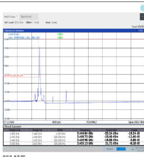
1-N77-3450-3550-30-40-L-1-DFT-PI2BPSK-Edge_1RB_Left-1@0-Ant1-PASS-see graph
