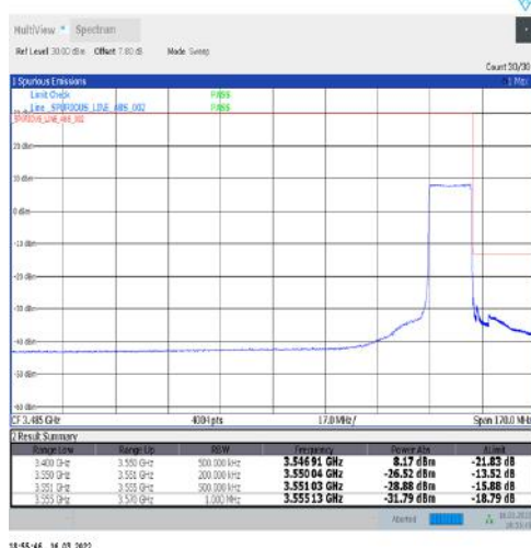
1-N77-3450-3550-30-15-H-6-CP-QPSK-Outer_Full-38@0-Ant1-PASS-see graph
