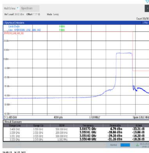
1-N77-3450-3550-30-20-H-6-CP-QPSK-Outer_Full-51@0-Ant1-PASS-see graph
