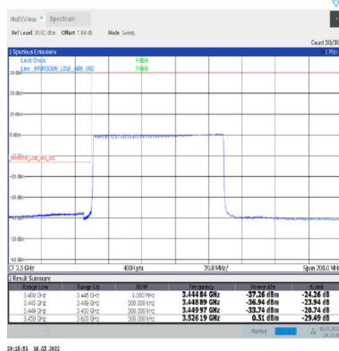
1-N77-3450-3550-30-80-L-6-CP-QPSK-Outer_Full-217@0-Ant1-PASS-see graph
