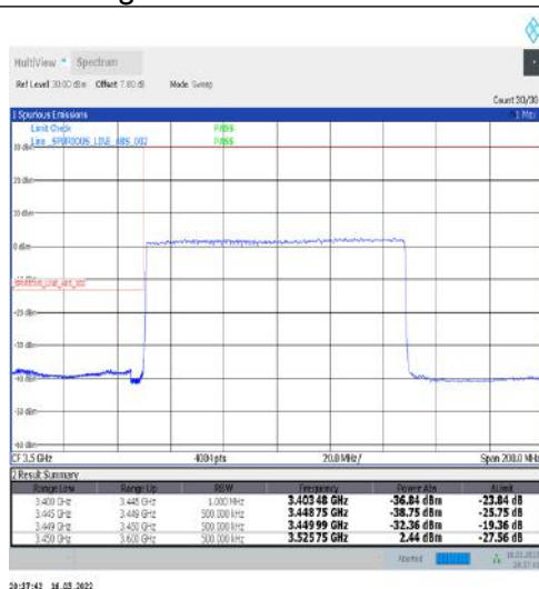
1-N77-3450-3550-30-100-L-3-DFT-PI2BPSK-Outer_Full-270@0-Ant1-PASS-see graph
