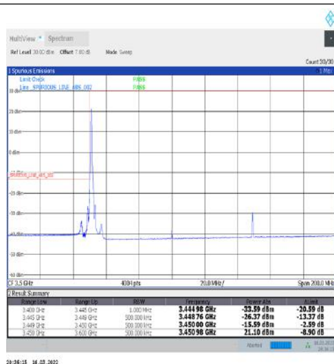
1-N77-3450-3550-30-100-L-1-DFT-PI2BPSK-Edge_1RB_Left-1@0-Ant1-PASS-see graph
