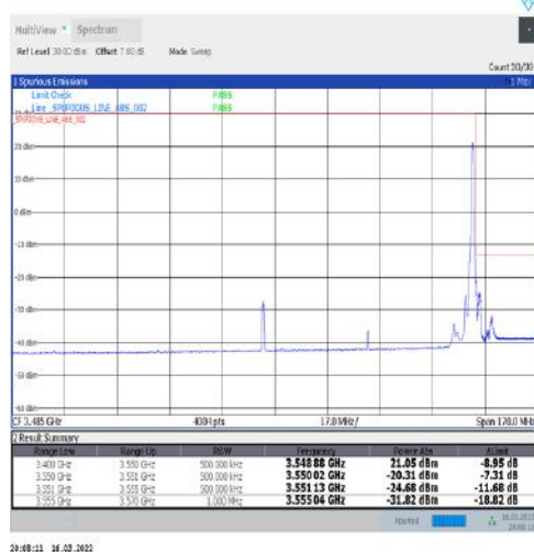
1-N77-3450-3550-30-70-H-5-CP-QPSK-Edge_1RB_Right-1@188-Ant1-PASS-see graph
