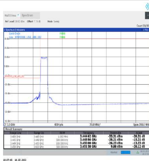
1-N77-3450-3550-30-10-L-6-CP-QPSK-Outer_Full-24@0-Ant1-PASS-see graph
