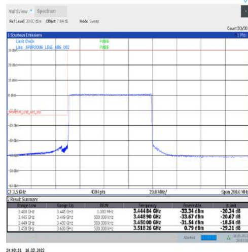
1-N77-3450-3550-30-70-L-6-CP-QPSK-Outer_Full-189@0-Ant1-PASS-see graph
