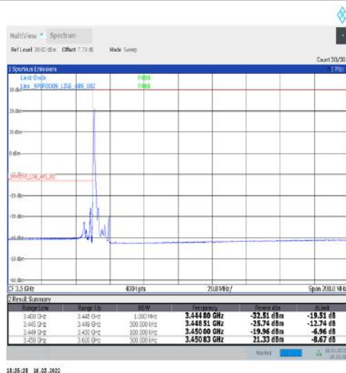
1-N77-3450-3550-30-10-L-4-CP-QPSK-Edge_1RB_Left-1@0-Ant1-PASS-see graph
