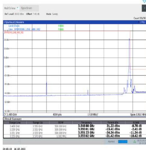
1-N77-3450-3550-30-100-H-5-CP-QPSK-Edge_1RB_Right-1@272-Ant1-PASS-see graph
