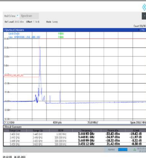
1-N77-3450-3550-30-30-L-4-CP-QPSK-Edge_1RB_Left-1@0-Ant1-PASS-see graph
