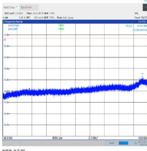
1-N77-3450-3550-30-100-M-1-DFT-PI2BPSK- Inner_1RB_Left-1@1-18000-40000-Ant1--47.81--13- PASS
