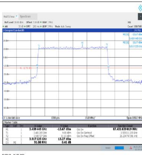
1-N77-3450-3550-30-90-H-8-CP-64QAM-Outer_Full-245@0-Ant1-87.432-91.080-≤90-PASS
