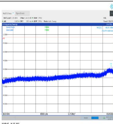
1-N77-3450-3550-30-100-H-1-DFT-PI2BPSK- Inner_1RB_Left-1@1-18000-40000-Ant1--46.91--13- PASS
