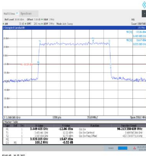
1-N77-3450-3550-30-100-L-1-DFT-QPSK-Outer_Full-270@0-Ant1-96.213-100.200-≤100-PASS
