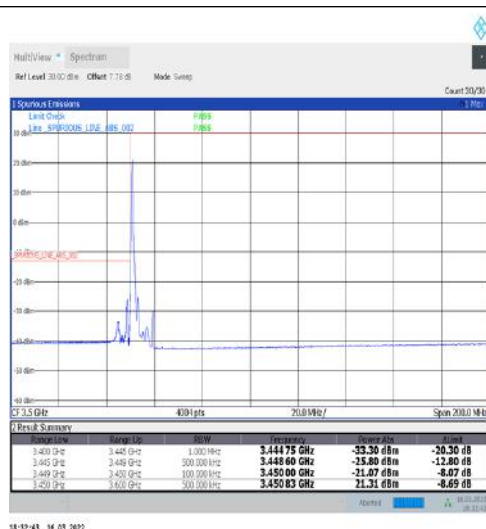
1-N77-3450-3550-30-10-L-1-DFT-PI2BPSK-Edge_1RB_Left-1@0-Ant1-PASS-see graph
