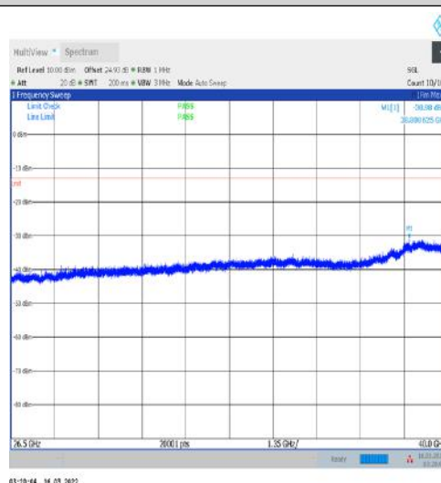
1-N77-3450-3550-30-100-H-1-DFT-PI2BPSK- Inner_1RB_Left-1@1-26500-40000-Ant1--30.98--13- PASS
