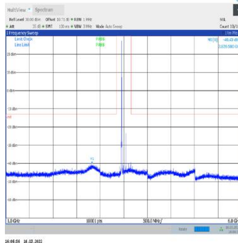
1-N77-3450-3550-30-100-L-1-DFT-PI2BPSK- Inner_1RB_Left-1@1-1000-6000-Ant1--40.43--13- PASS
