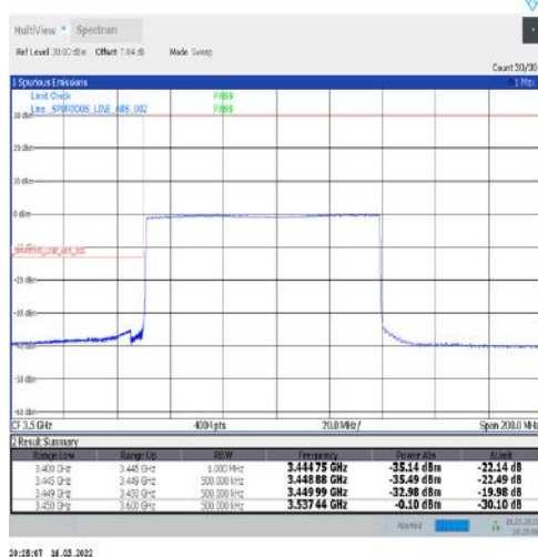
1-N77-3450-3550-30-90-L-6-CP-QPSK-Outer_Full-245@0-Ant1-PASS-see graph
