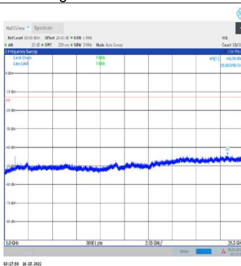
1-N77-3450-3550-30-100-L-1-DFT-PI2BPSK- Inner_1RB_Left-1@1-6000-26500-Ant1--44.28--13- PASS
