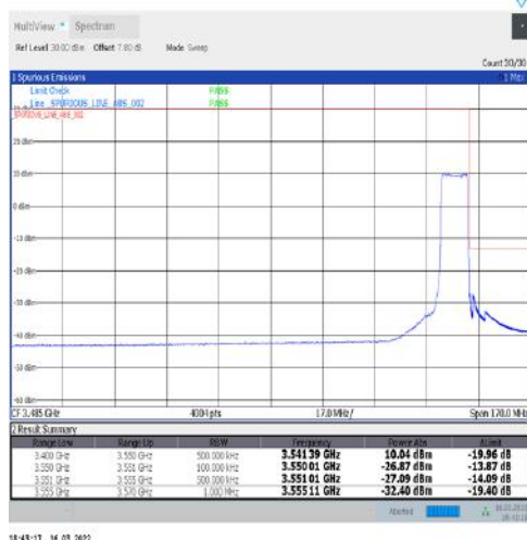
1-N77-3450-3550-30-10-H-6-CP-QPSK-Outer_Full-24@0-Ant1-PASS-see graph
