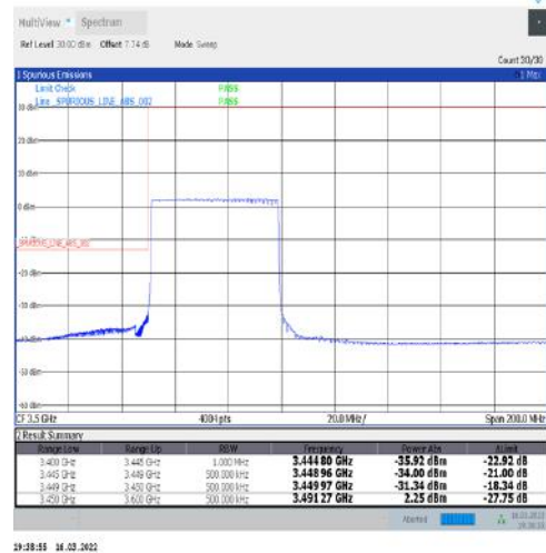
1-N77-3450-3550-30-50-L-6-CP-QPSK-Outer_Full-133@0-Ant1-PASS-see graph
