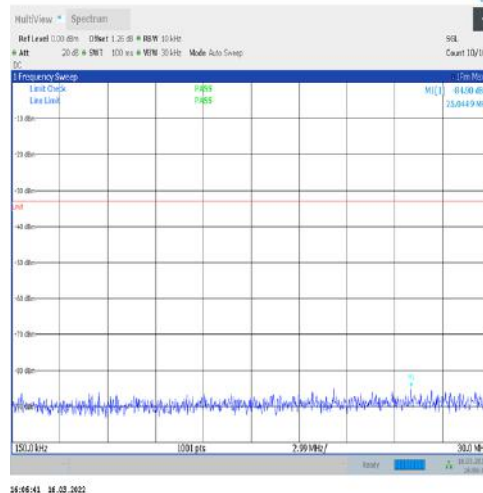
1-N77-3450-3550-30-100-L-1-DFT-PI2BPSK- Inner_1RB_Left-1@1-0.15-30-Ant1--84.90--33-PASS
