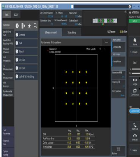
1-N77-3450-3550-30-100-M-7-CP-16QAM-Outer_Full-273@0-Ant1-see graph-PASS
