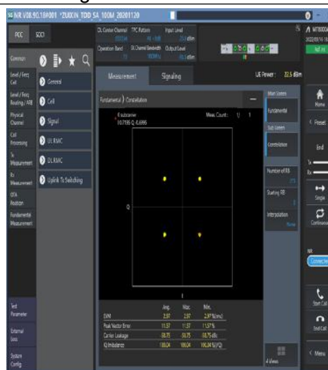
1-N77-3450-3550-30-100-M-6-CP-QPSK-Outer_Full-273@0-Ant1-see graph-PASS
