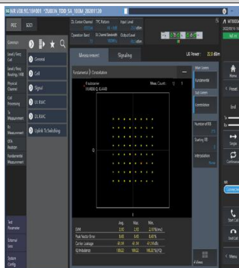
1-N77-3450-3550-30-100-M-8-CP-64QAM-Outer_Full-273@0-Ant1-see graph-PASS
