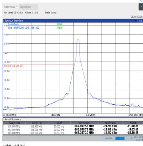
1-N71-15-5-L-4-CP-QPSK-Edge_1RB_Left-1@0-Ant1-PASS-see graph
