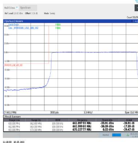
1-N71-15-10-L-6-CP-QPSK-Outer_Full-52@0-Ant1-PASS-see graph
