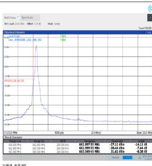
1-N71-15-20-L-1-DFT-PI2BPSK-Edge_1RB_Left-1@0-Ant1-PASS-see graph
