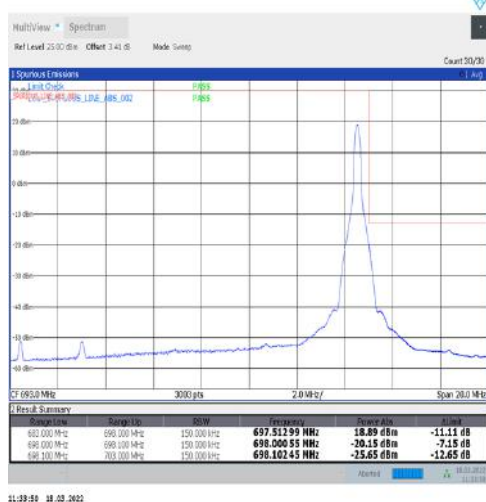
1-N71-15-15-H-5-CP-QPSK-Edge_1RB_Right-1@78-Ant1-PASS-see graph
