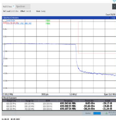
1-N71-15-10-H-6-CP-QPSK-Outer_Full-52@0-Ant1-PASS-see graph
