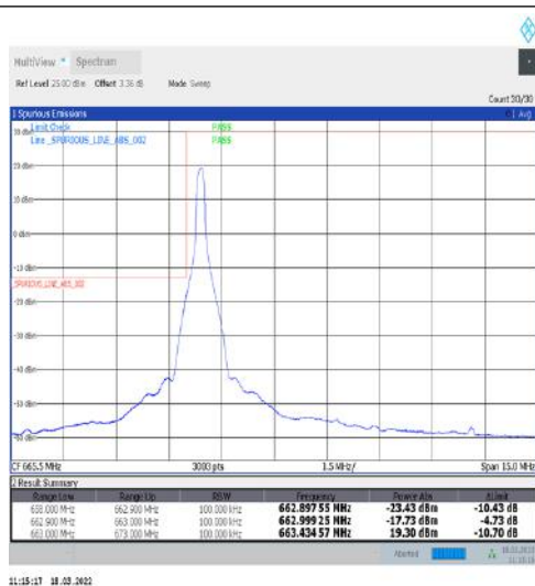
1-N71-15-10-L-1-DFT-PI2BPSK-Edge_1RB_Left-1@0-Ant1-PASS-see graph
