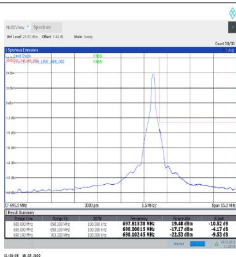
1-N71-15-10-H-2-DFT-PI2BPSK-Edge_1RB_Right-1@51-Ant1-PASS-see graph
