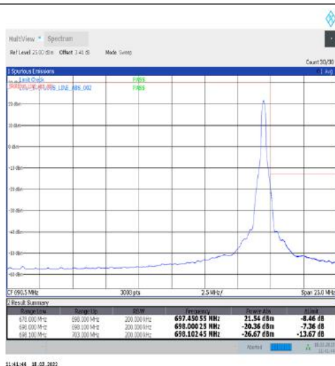
1-N71-15-20-H-2-DFT-PI2BPSK-Edge_1RB_Right-1@105-Ant1-PASS-see graph
