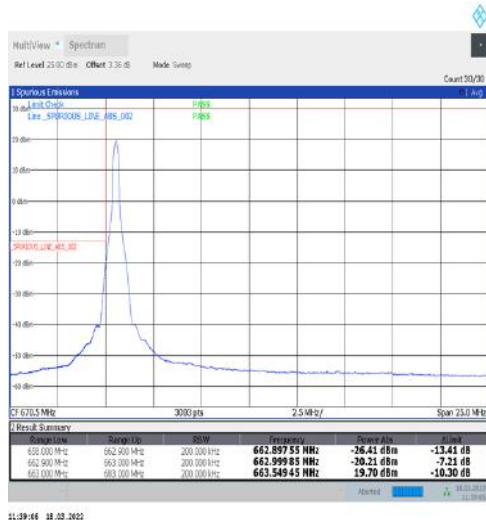
1-N71-15-20-L-4-CP-QPSK-Edge_1RB_Left-1@0-Ant1-PASS-see graph
