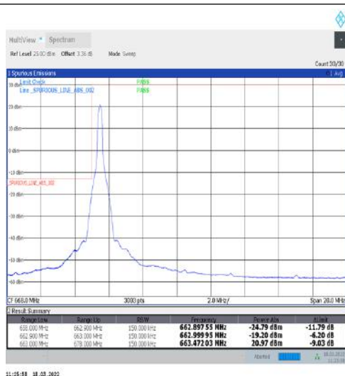
1-N71-15-15-L-1-DFT-PI2BPSK-Edge_1RB_Left-1@0-Ant1-PASS-see graph
