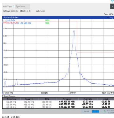
1-N71-15-10-H-5-CP-QPSK-Edge_1RB_Right-1@51-Ant1-PASS-see graph
