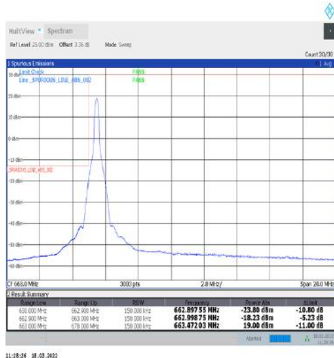
1-N71-15-15-L-4-CP-QPSK-Edge_1RB_Left-1@0-Ant1-PASS-see graph
