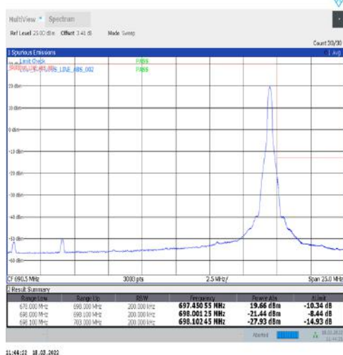
1-N71-15-20-H-5-CP-QPSK-Edge_1RB_Right-1@105-Ant1-PASS-see graph
