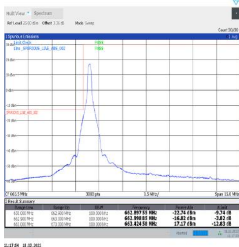
1-N71-15-10-L-4-CP-QPSK-Edge_1RB_Left-1@0-Ant1-PASS-see graph
