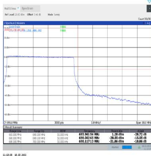
1-N71-15-5-H-6-CP-QPSK-Outer_Full-25@0-Ant1-PASS-see graph
