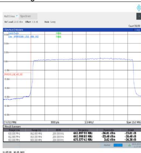
1-N71-15-20-L-3-DFT-PI2BPSK-Outer_Full-100@0-Ant1-PASS-see graph
