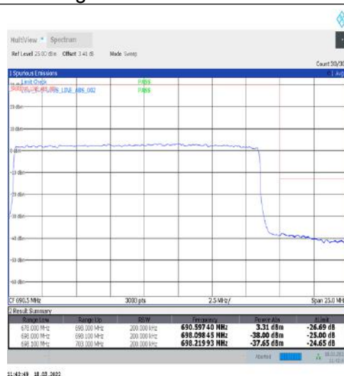
1-N71-15-20-H-3-DFT-PI2BPSK-Outer_Full-100@0-Ant1-PASS-see graph
