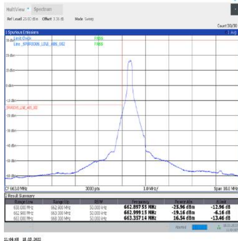
1-N71-15-5-L-1-DFT-PI2BPSK-Edge_1RB_Left-1@0-Ant1-PASS-see graph
