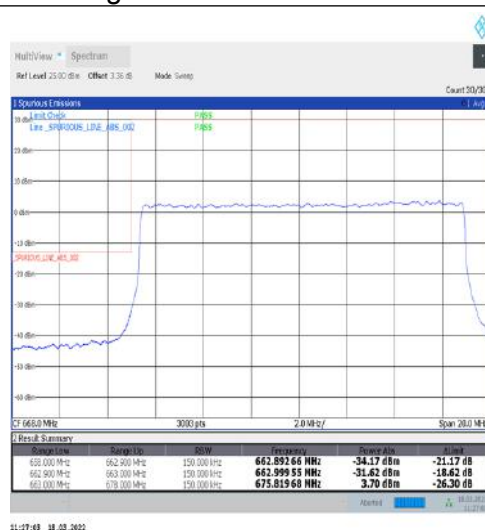
1-N71-15-15-L-3-DFT-PI2BPSK-Outer_Full-75@0-Ant1-PASS-see graph
