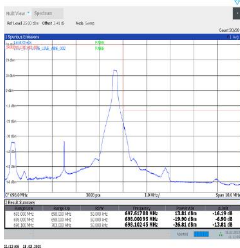
1-N71-15-5-H-5-CP-QPSK-Edge_1RB_Right-1@24-Ant1-PASS-see graph
