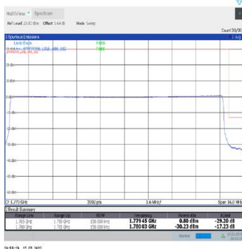
1-N66-15-15-H-6-CP-QPSK-Outer_Full-79@0-Ant1-seegraph-PASS-see graph
