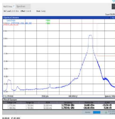
1-N66-15-5-H-5-CP-QPSK-Edge_1RB_Right-1@24-Ant1-seegraph-PASS-see graph
