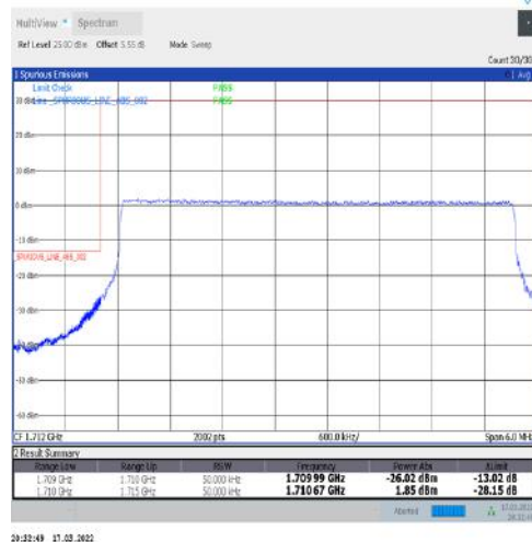
1-N66-15-5-L-6-CP-QPSK-Outer_Full-25@0-Ant1-seegraph-PASS-see graph
