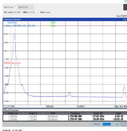
1-N66-15-15-L-4-CP-QPSK-Edge_1RB_Left-1@0-Ant1-seegraph-PASS-see graph
