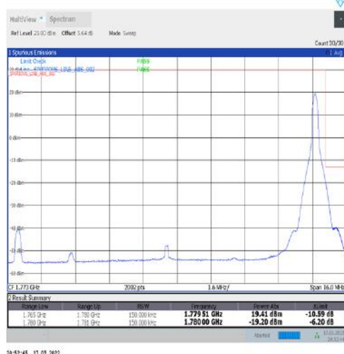
1-N66-15-15-H-5-CP-QPSK-Edge_1RB_Right-1@78-Ant1-seegraph-PASS-see graph
