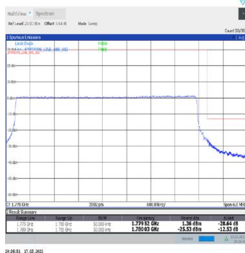
1-N66-15-5-H-6-CP-QPSK-Outer_Full-25@0-Ant1-seegraph-PASS-see graph
