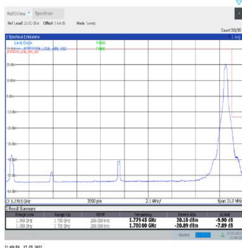
1-N66-15-20-H-5-CP-QPSK-Edge_1RB_Right-1@105-Ant1-seegraph-PASS-see graph
