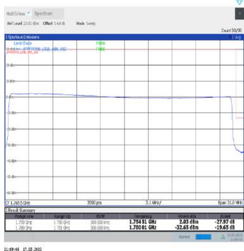
1-N66-15-30-H-6-CP-QPSK-Outer_Full-160@0-Ant1-seegraph-PASS-see graph
