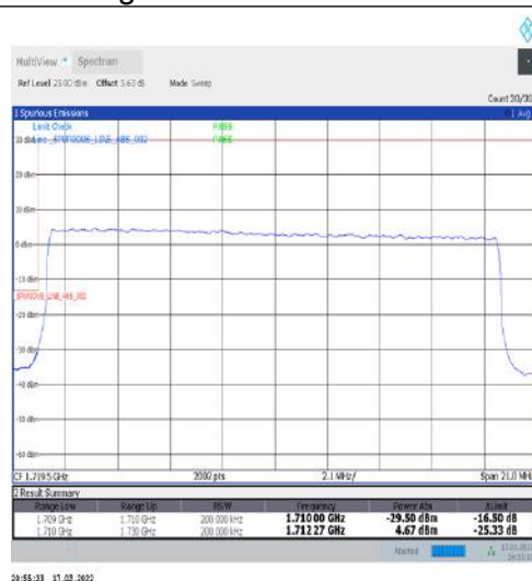
1-N66-15-20-L-3-DFT-PI2BPSK-Outer_Full-100@0-Ant1-seegraph-PASS-see graph
