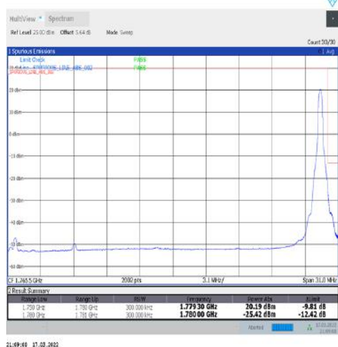
1-N66-15-30-H-5-CP-QPSK-Edge_1RB_Right-1@159-Ant1-seegraph-PASS-see graph
