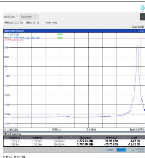
1-N66-15-30-H-2-DFT-PI2BPSK-Edge_1RB_Right-1@159-Ant1-seegraph-PASS-see graph
