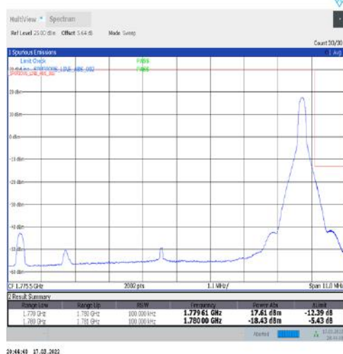
1-N66-15-10-H-5-CP-QPSK-Edge_1RB_Right-1@51-Ant1-seegraph-PASS-see graph
