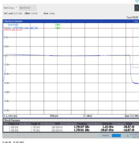
1-N66-15-20-H-6-CP-QPSK-Outer_Full-106@0-Ant1-seegraph-PASS-see graph
