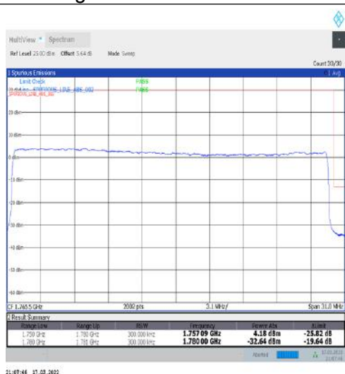
1-N66-15-30-H-3-DFT-PI2BPSK-Outer_Full-160@0-Ant1-seegraph-PASS-see graph
