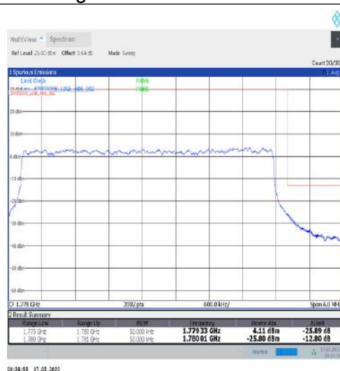
1-N66-15-5-H-3-DFT-PI2BPSK-Outer_Full-25@0-Ant1-seegraph-PASS-see graph
