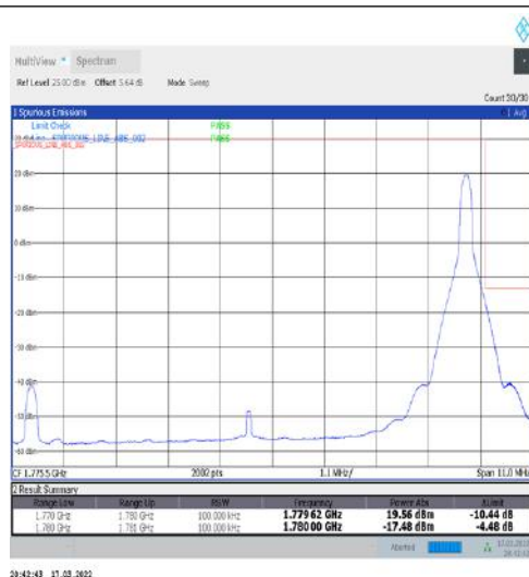
1-N66-15-10-H-2-DFT-PI2BPSK-Edge_1RB_Right-1@51-Ant1-seegraph-PASS-see graph
