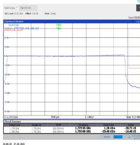
1-N66-15-10-H-6-CP-QPSK-Outer_Full-52@0-Ant1-seegraph-PASS-see graph
