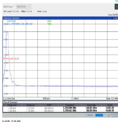
1-N66-15-40-L-4-CP-QPSK-Edge_1RB_Left-1@0-Ant1-seegraph-PASS-see graph
