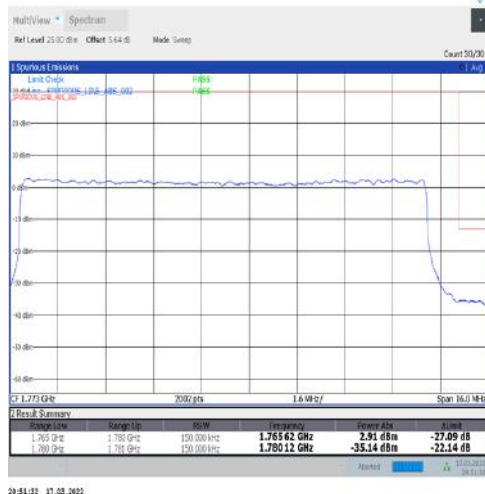
1-N66-15-15-H-3-DFT-PI2BPSK-Outer_Full-75@0-Ant1-seegraph-PASS-see graph
