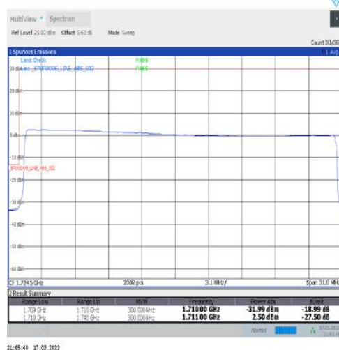
1-N66-15-30-L-6-CP-QPSK-Outer_Full-160@0-Ant1-seegraph-PASS-see graph
