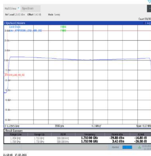
1-N66-15-40-L-6-CP-QPSK-Outer_Full-216@0-Ant1-seegraph-PASS-see graph
