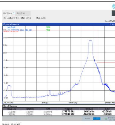
1-N66-15-5-H-2-DFT-PI2BPSK-Edge_1RB_Right-1@24-Ant1-seegraph-PASS-see graph
