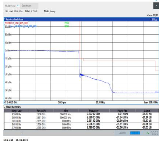
1-N41--30-100-H-6-CP-QPSK-Outer_Full-273@0-Ant1-PASS-see graph
