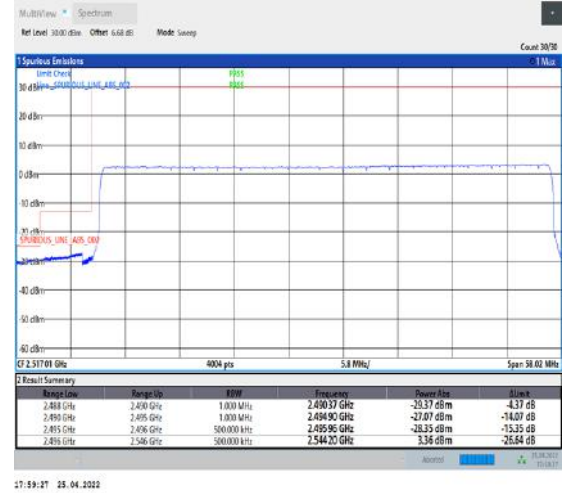
1-N41--30-50-L-6-CP-QPSK-Outer_Full-133@0-Ant2-PASS-see graph
