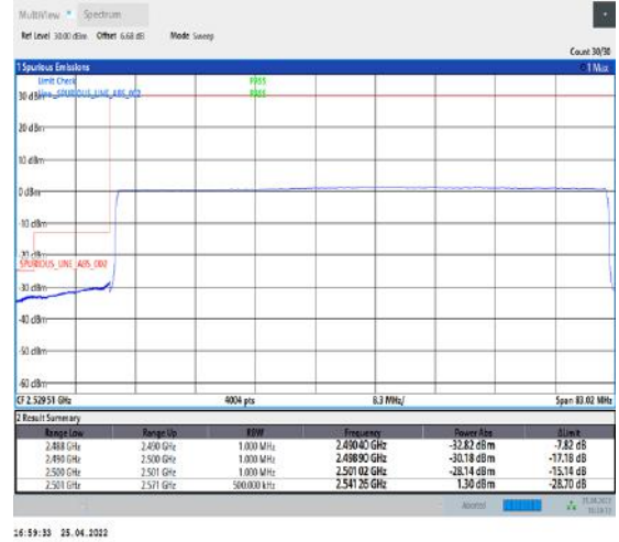
1-N41--30-70-L-6-CP-QPSK-Outer_Full-189@0-Ant1-PASS-see graph
