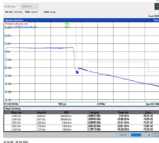
1-N41--30-30-H-6-CP-QPSK-Outer_Full-78@0- Ant1-PASS-see graph
