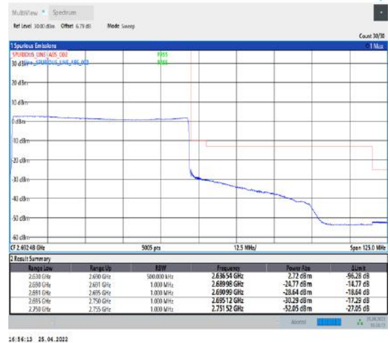
1-N41--30-60-H-6-CP-QPSK-Outer_Full-162@0-Ant1-PASS-see graph
