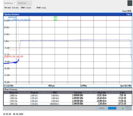
1-N41--30-60-L-6-CP-QPSK-Outer_Full-162@0-Ant1-PASS-see graph
