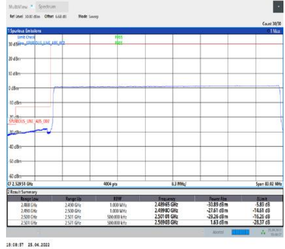
1-N41--30-70-L-6-CP-QPSK-Outer_Full-189@0-Ant2-PASS-see graph
