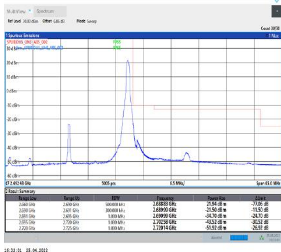
1-N41--30-30-H-5-CP-QPSK-Edge_1RB_Right-1@77- Ant1-PASS-see graph
