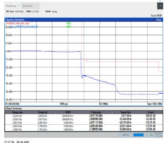
1-N41--30-90-H-6-CP-QPSK-Outer_Full-245@0-Ant1-PASS-see graph
