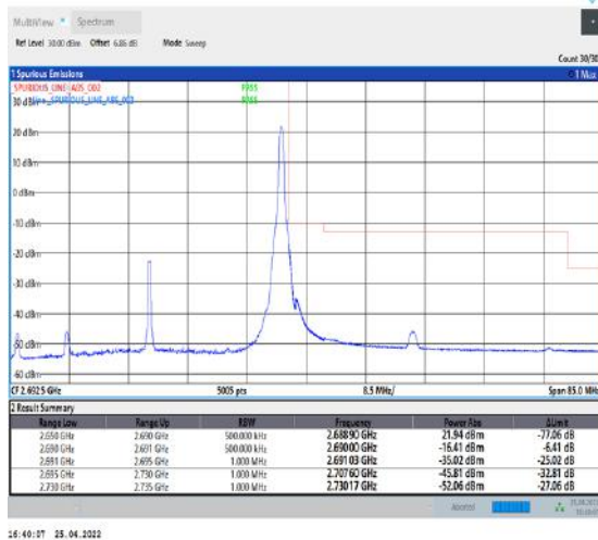
1-N41--30-40-H-5-CP-QPSK-Edge_1RB_Right-1@105-Ant1-PASS-see graph
