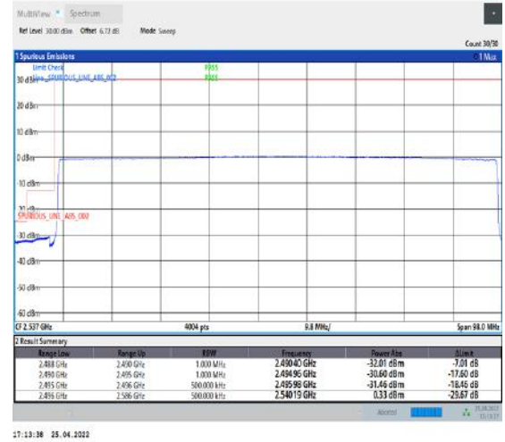
1-N41--30-90-L-6-CP-QPSK-Outer_Full-245@0-Ant1-PASS-see graph
