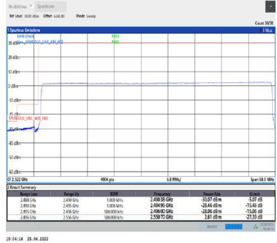
1-N41--30-60-L-6-CP-QPSK-Outer_Full-162@0-Ant2-PASS-see graph
