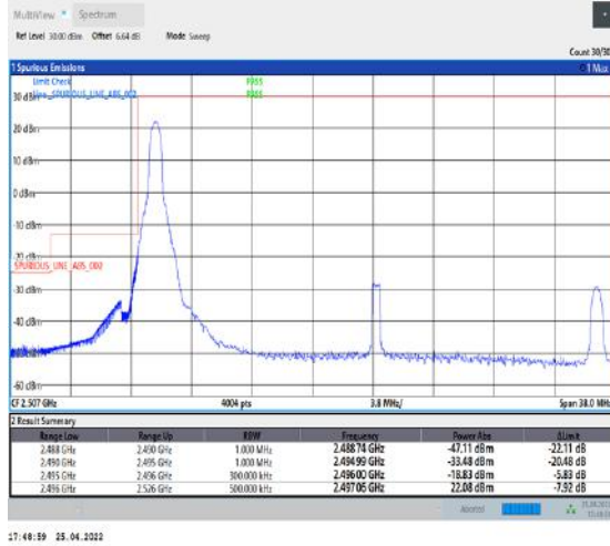
1-N41--30-30-L-4-CP-QPSK-Edge_1RB_Left-1@0-Ant2-PASS-see graph
