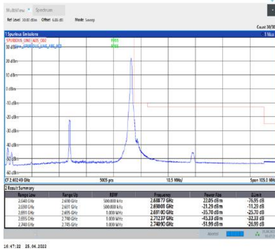
1-N41--30-50-H-5-CP-QPSK-Edge_1RB_Right-1@132-Ant1-PASS-see graph
