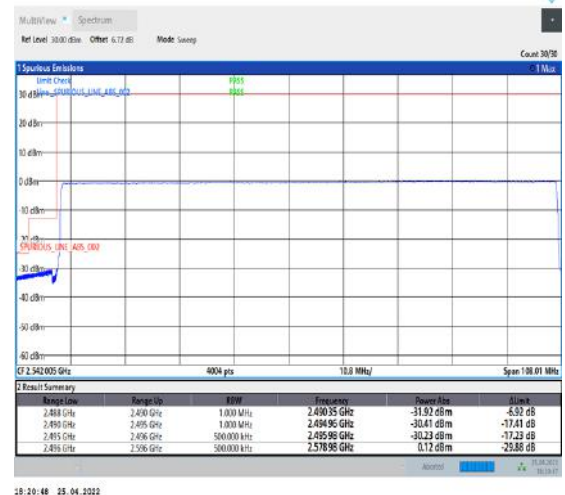
1-N41--30-100-L-6-CP-QPSK-Outer_Full-273@0-Ant2-PASS-see graph
