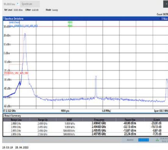
1-N41--30-60-L-4-CP-QPSK-Edge_1RB_Left-1@0-Ant2-PASS-see graph
