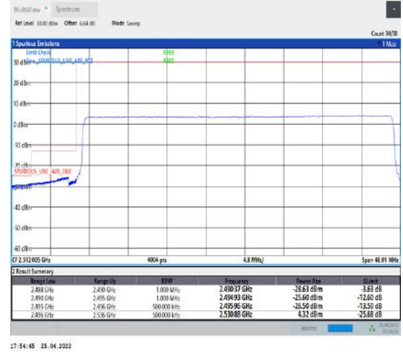
1-N41--30-40-L-6-CP-QPSK-Outer_Full-106@0-Ant2-PASS-see graph
