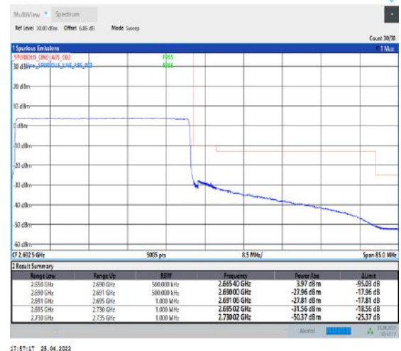
1-N41--30-40-H-6-CP-QPSK-Outer_Full-106@0-Ant2-PASS-see graph
