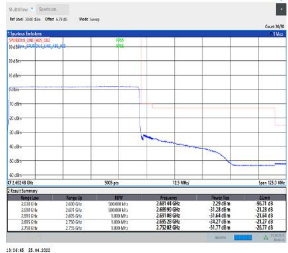
1-N41--30-60-H-6-CP-QPSK-Outer_Full-162@0-Ant2-PASS-see graph
