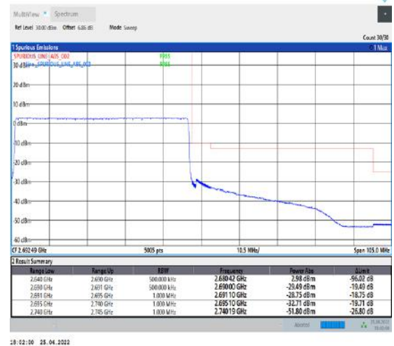
1-N41--30-50-H-6-CP-QPSK-Outer_Full-133@0-Ant2-PASS-see graph
