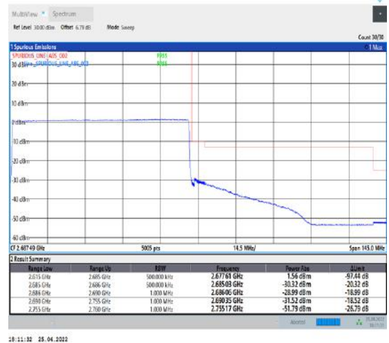
1-N41--30-70-H-6-CP-QPSK-Outer_Full-189@0-Ant2-PASS-see graph
