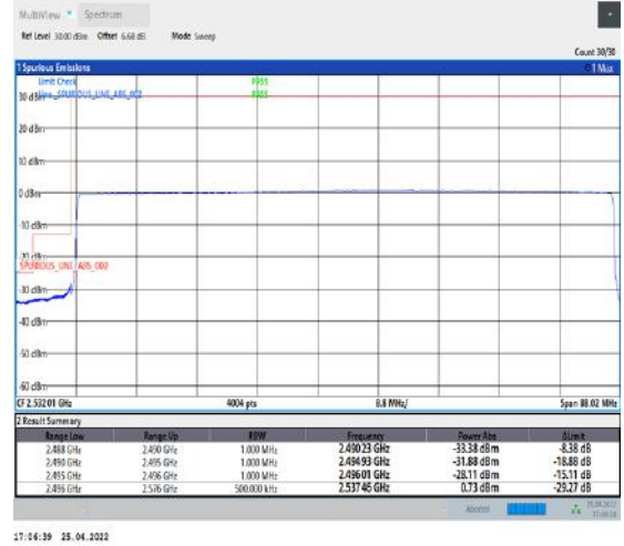
1-N41--30-80-L-6-CP-QPSK-Outer_Full-217@0-Ant1-PASS-see graph
