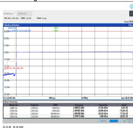
1-N41--30-80-L-6-CP-QPSK-Outer_Full-217@0- Ant2-PASS-see graph
