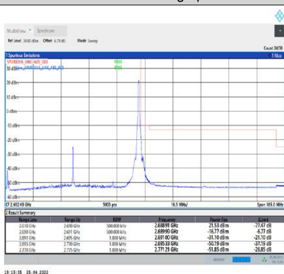
1-N41--30-80-H-5-CP-QPSK-Edge_1RB_Right-1@216- Ant2-PASS-see graph
