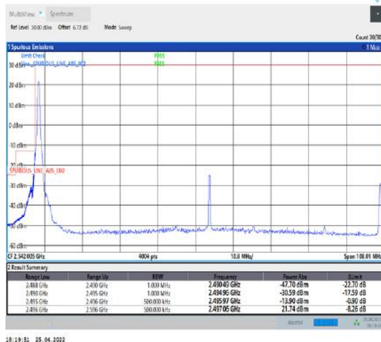
1-N41--30-100-L-4-CP-QPSK-Edge_1RB_Left-1@0-Ant2-PASS-see graph
