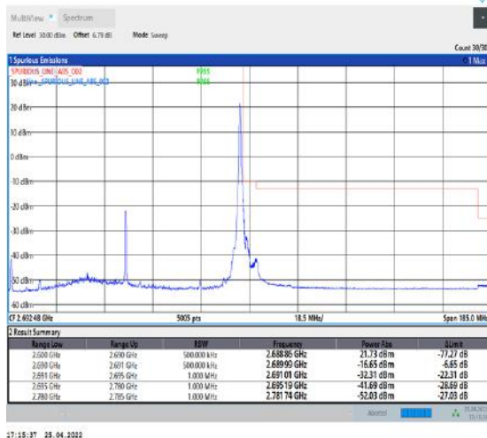
1-N41--30-90-H-5-CP-QPSK-Edge_1RB_Right-1@244-Ant1-PASS-see graph
