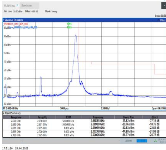
1-N41--30-30-H-5-CP-QPSK-Edge_1RB_Right-1@77-Ant2-PASS-see graph
