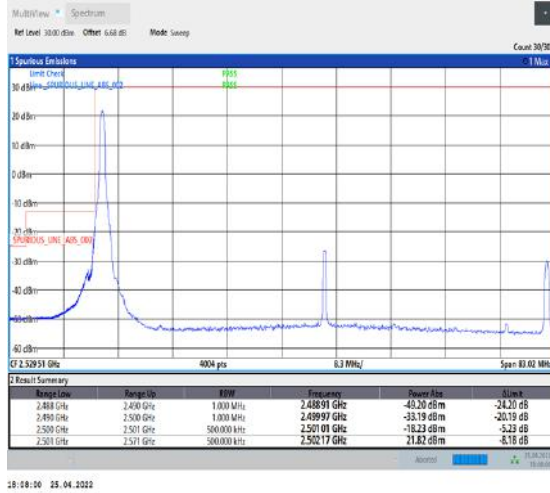
1-N41--30-70-L-4-CP-QPSK-Edge_1RB_Left-1@0-Ant2-PASS-see graph
