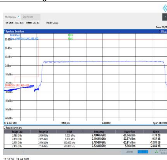
1-N41--30-30-L-6-CP-QPSK-Outer_Full-78@0- Ant1-PASS-see graph
