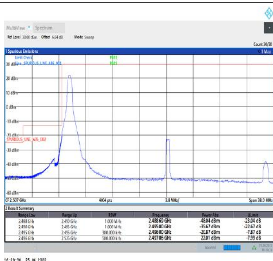
1-N41--30-30-L-4-CP-QPSK-Edge_1RB_Left-1@0- Ant1-PASS-see graph
