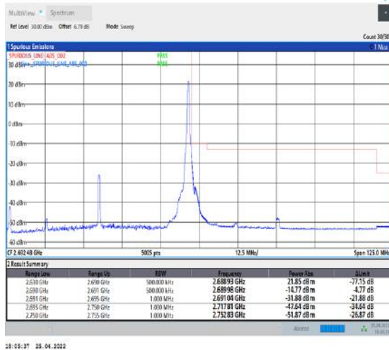
1-N41--30-60-H-5-CP-QPSK-Edge_1RB_Right-1@161-Ant2-PASS-see graph
