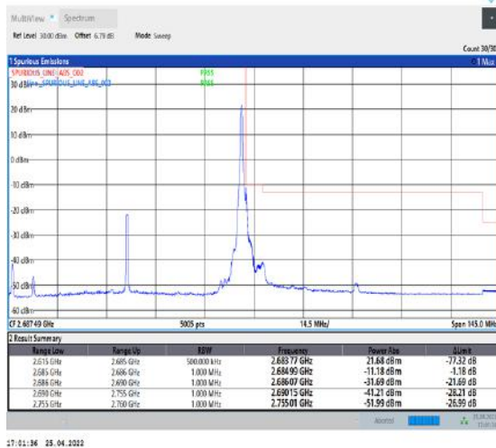
1-N41--30-70-H-5-CP-QPSK-Edge_1RB_Right-1@188-Ant1-PASS-see graph
