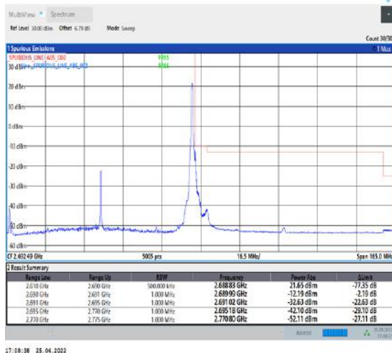
1-N41--30-80-H-5-CP-QPSK-Edge_1RB_Right-1@216-Ant1-PASS-see graph
