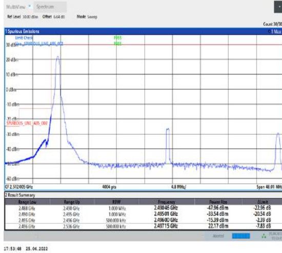
1-N41--30-40-L-4-CP-QPSK-Edge_1RB_Left-1@0-Ant2-PASS-see graph
