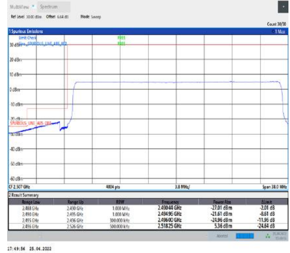
1-N41--30-30-L-6-CP-QPSK-Outer_Full-78@0-Ant2-PASS-see graph
