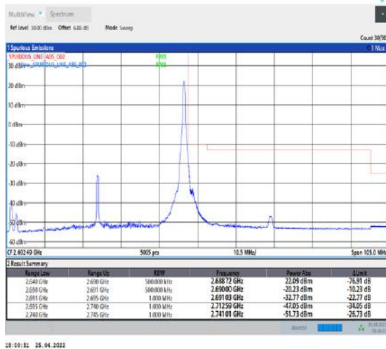
1-N41--30-50-H-5-CP-QPSK-Edge_1RB_Right-1@132-Ant2-PASS-see graph
