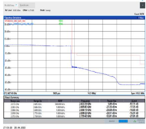
1-N41--30-70-H-6-CP-QPSK-Outer_Full-189@0-Ant1-PASS-see graph
