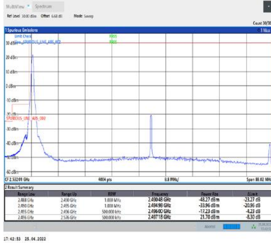
1-N41--30-80-L-4-CP-QPSK-Edge_1RB_Left-1@0-Ant1-PASS-see graph
