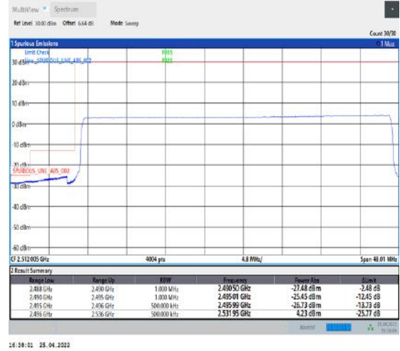
1-N41--30-40-L-6-CP-QPSK-Outer_Full-106@0-Ant1-PASS-see graph
