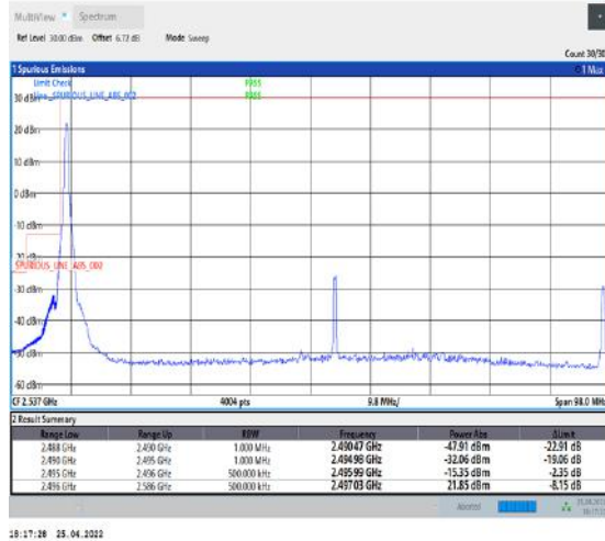
1-N41--30-90-L-4-CP-QPSK-Edge_1RB_Left-1@0-Ant2-PASS-see graph
