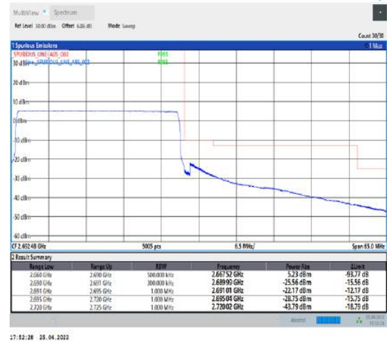
1-N41--30-30-H-6-CP-QPSK-Outer_Full-78@0-Ant2-PASS-see graph
