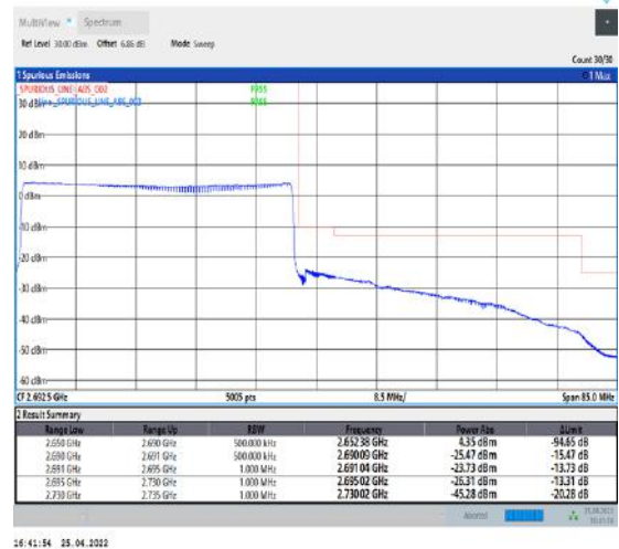
1-N41--30-40-H-6-CP-QPSK-Outer_Full-106@0-Ant1-PASS-see graph
