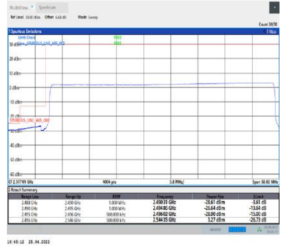
1-N41--30-50-L-6-CP-QPSK-Outer_Full-133@0-Ant1-PASS-see graph
