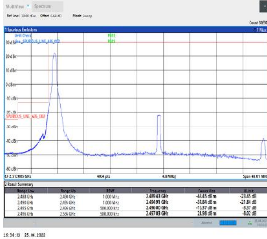
1-N41--30-40-L-4-CP-QPSK-Edge_1RB_Left-1@0-Ant1-PASS-see graph
