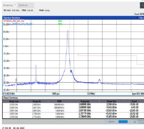
1-N41--30-40-H-5-CP-QPSK-Edge_1RB_Right-1@105-Ant2-PASS-see graph
