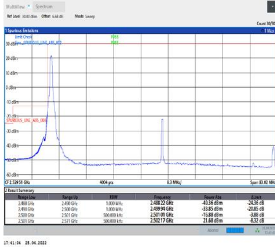
1-N41--30-70-L-4-CP-QPSK-Edge_1RB_Left-1@0-Ant1-PASS-see graph
