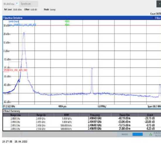
1-N41--30-60-L-4-CP-QPSK-Edge_1RB_Left-1@0-Ant1-PASS-see graph
