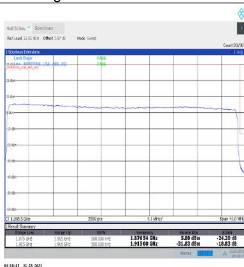
1-N25-15-40-H-3-DFT-PI2BPSK-Outer_Full-216@0-Ant1-seegraph-PASS-see graph
