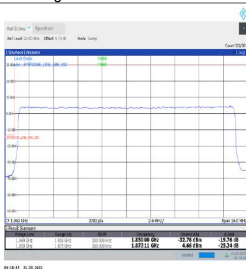
1-N25-15-25-L-3-DFT-PI2BPSK-Outer_Full-128@0-Ant1-seegraph-PASS-see graph
