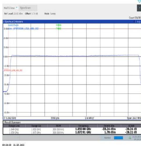
1-N25-15-25-L-6-CP-QPSK-Outer_Full-133@0-Ant1-seegraph-PASS-see graph
