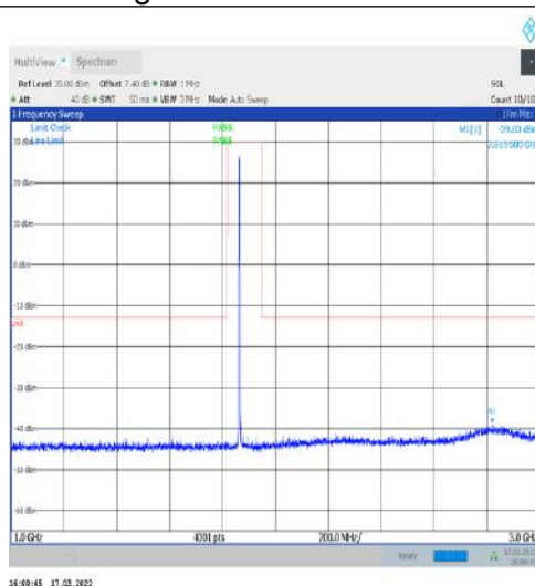
1-N25-15-40-M-1-DFT-PI2BPSK-Inner_1RB_Left- 1@1-1000-3000-Ant1--39.03--13-PASS
