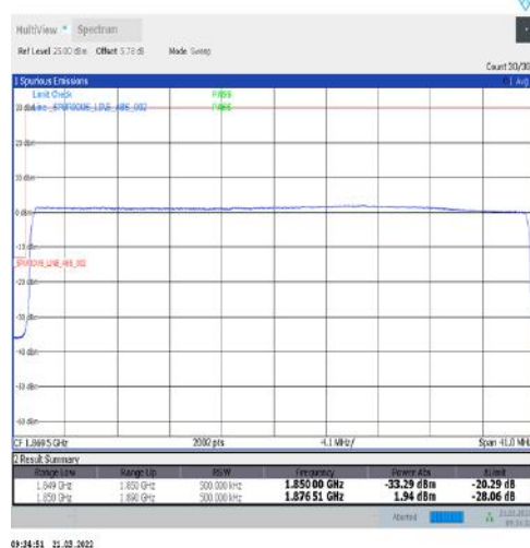
1-N25-15-40-L-6-CP-QPSK-Outer_Full-216@0-Ant1-seegraph-PASS-see graph
