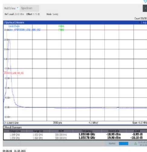
1-N25-15-40-L-4-CP-QPSK-Edge_1RB_Left-1@0-Ant1-seegraph-PASS-see graph
