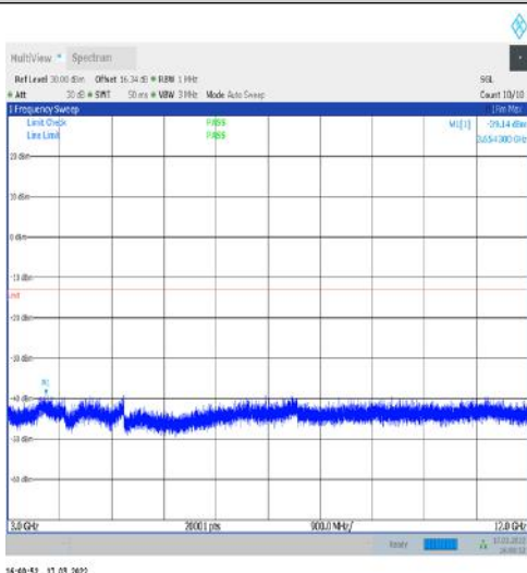
1-N25-15-40-M-1-DFT-PI2BPSK-Inner_1RB_Left- 1@1-3000-12000-Ant1--39.14--13-PASS
