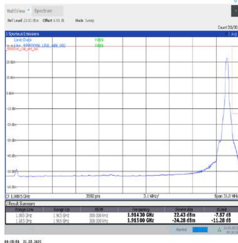
1-N25-15-30-H-2-DFT-PI2BPSK-Edge_1RB_Right-1@159-Ant1-seegraph-PASS-see graph
