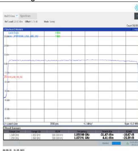
1-N25-15-40-L-3-DFT-PI2BPSK-Outer_Full-216@0-Ant1-seegraph-PASS-see graph
