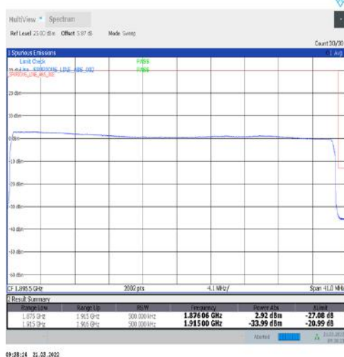
1-N25-15-40-H-6-CP-QPSK-Outer_Full-216@0-Ant1-seegraph-PASS-see graph
