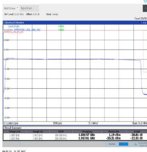
1-N25-15-30-H-6-CP-QPSK-Outer_Full-160@0-Ant1-seegraph-PASS-see graph
