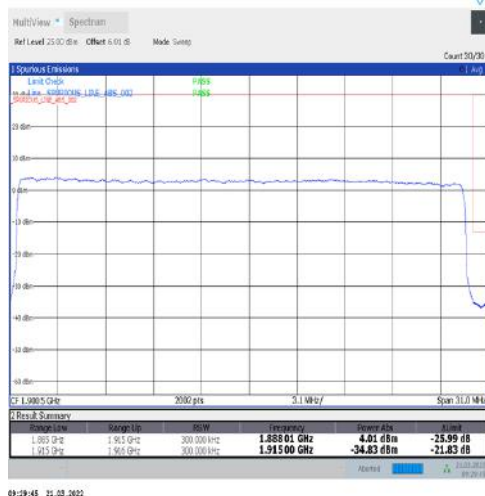
1-N25-15-30-H-3-DFT-PI2BPSK-Outer_Full-160@0-Ant1-seegraph-PASS-see graph
