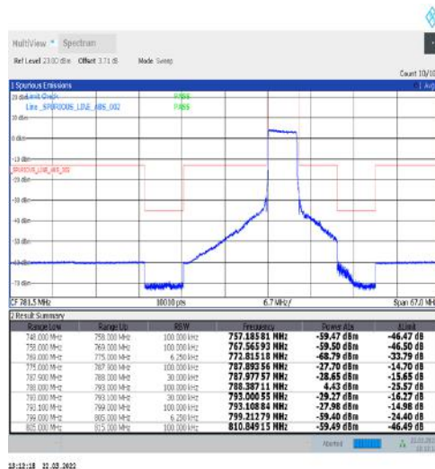
1-N14-15-5-L-6-CP-QPSK-Outer_Full-25@0-Ant1-PASS-see graph
