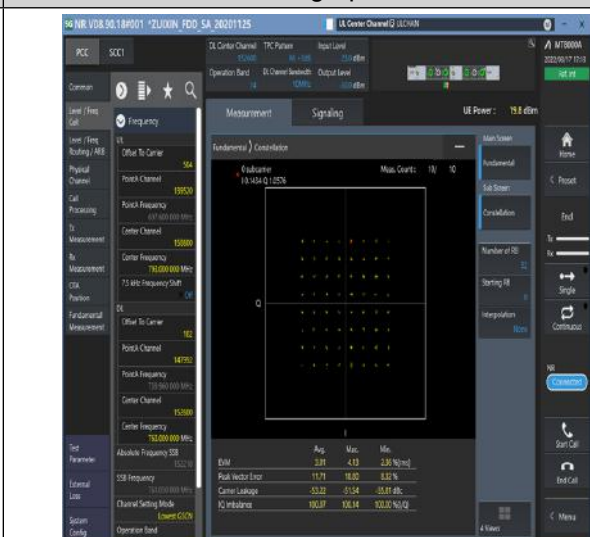
1-N14-15-10-M-8-CP-64QAM-Outer_Full-52@0-Ant1-see graph-PASS
