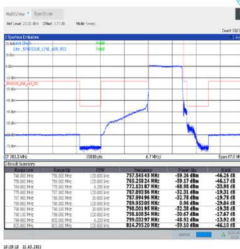
1-N14-15-10-M-4-CP-QPSK-Outer_Full-52@0-Ant1-PASS-see graph
