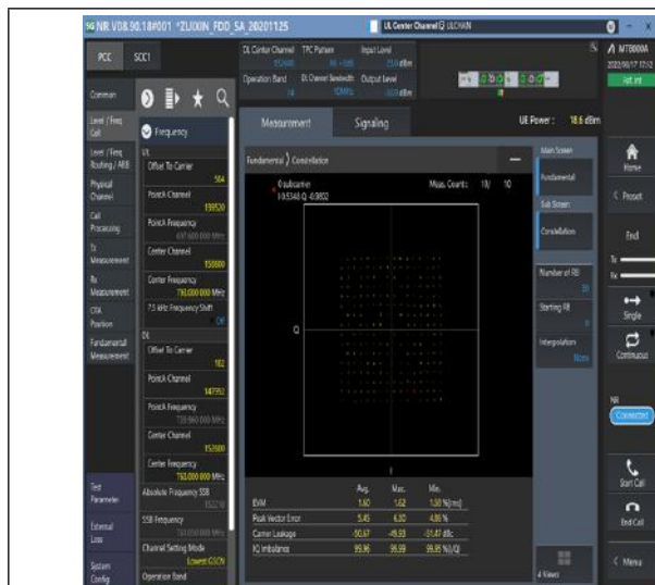
1-N14-15-10-M-5-DFT-256QAM-Outer_Full-50@0-Ant1-see graph-PASS
