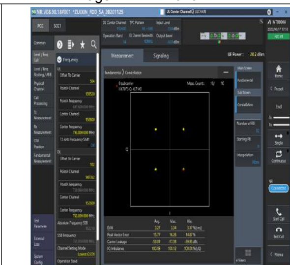
1-N14-15-10-M-6-CP-QPSK-Outer_Full-52@0-Ant1-see graph-PASS
