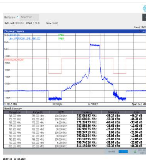
1-N14-15-5-L-3-DFT-PI2BPSK-Outer_Full-25@0-Ant1-PASS-see graph
