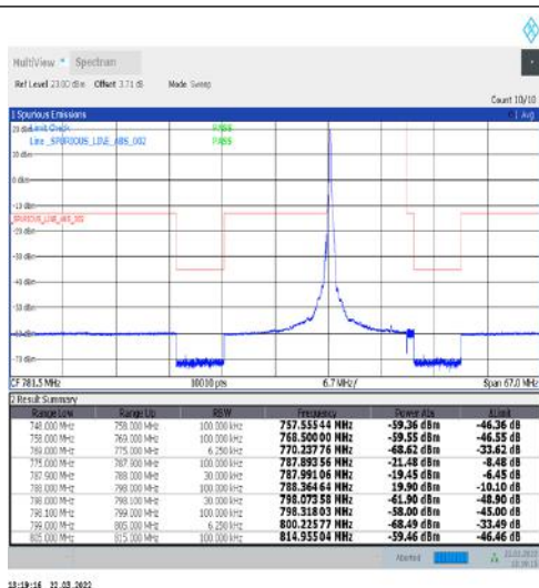
1-N14-15-10-M-1-DFT-PI2BPSK-Edge_1RB_Left-1@0-Ant1-PASS-see graph
