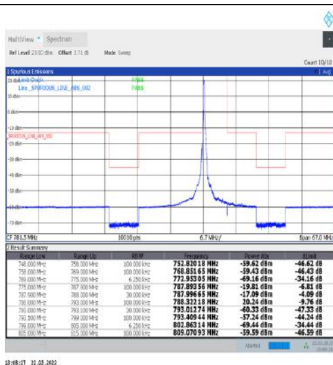
1-N14-15-5-L-1-DFT-PI2BPSK-Edge_1RB_Left-1@0-Ant1-PASS-see graph
