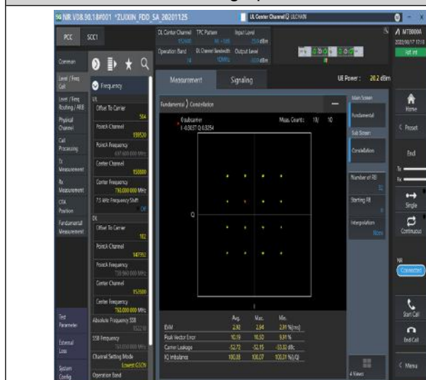
1-N14-15-10-M-7-CP-16QAM-Outer_Full-52@0-Ant1-see graph-PASS
