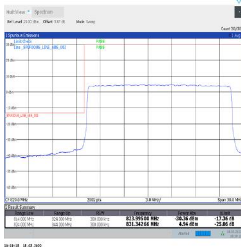
1-N5-15-20-L-3-DFT-PI2BPSK-Outer_Full-100@0-Ant1-seegraph-PASS-see graph
