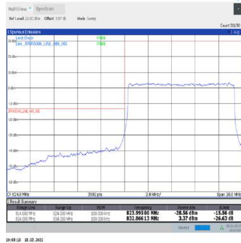
1-N5-15-10-L-3-DFT-PI2BPSK-Outer_Full-50@0-Ant1-seegraph-PASS-see graph
