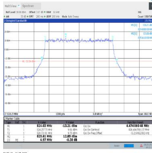
1-N5-15-5-L-2-DFT-PI2BPSK-Outer_Full-25@0-Ant1- 4.474-4.970-≤5-PASS
