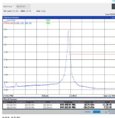
1-N5-15-15-H-5-CP-QPSK-Edge_1RB_Right-1@78-Ant1-seegraph-PASS-see graph
