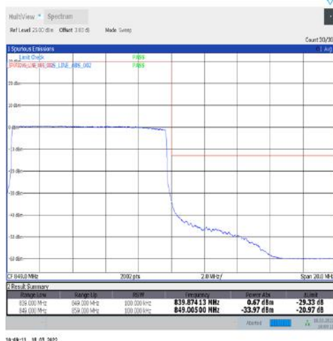
1-N5-15-10-H-6-CP-QPSK-Outer_Full-52@0-Ant1-seegraph-PASS-see graph
