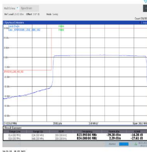
1-N5-15-20-L-6-CP-QPSK-Outer_Full-106@0-Ant1-seegraph-PASS-see graph
