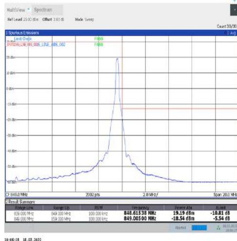
1-N5-15-10-H-2-DFT-PI2BPSK-Edge_1RB_Right-1@51-Ant1-seegraph-PASS-see graph
