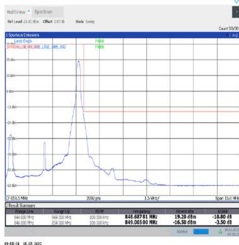
1-N5-15-5-H-2-DFT-PI2BPSK-Edge_1RB_Right-1@24-Ant1-seegraph-PASS-see graph
