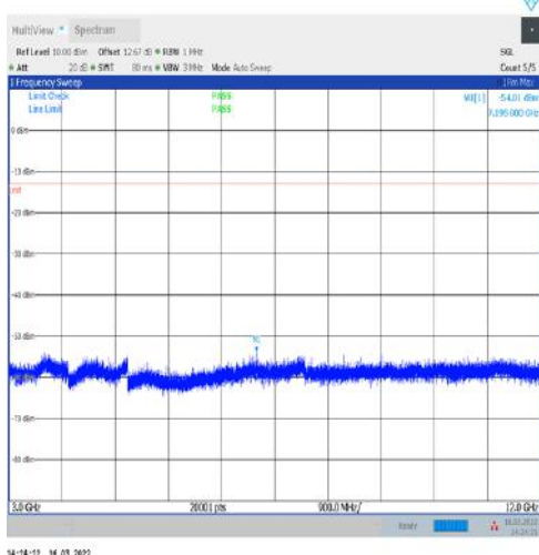
1-N5-15-20-H-1-DFT-PI2BPSK-Inner_1RB_Left- 1@1-3000-12000-Ant1--54.01--13-PASS
