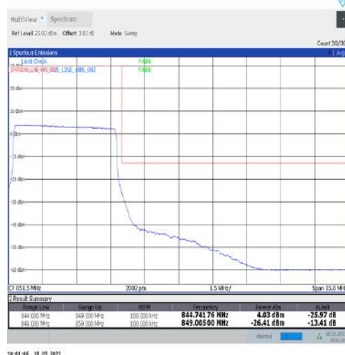
1-N5-15-5-H-6-CP-QPSK-Outer_Full-25@0-Ant1-seegraph-PASS-see graph
