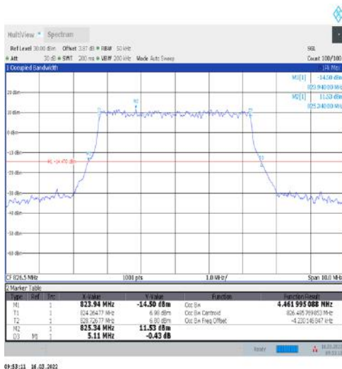
1-N5-15-5-L-3-DFT-16QAM-Outer_Full-25@0-Ant1- 4.462-5.110-≤5-PASS
