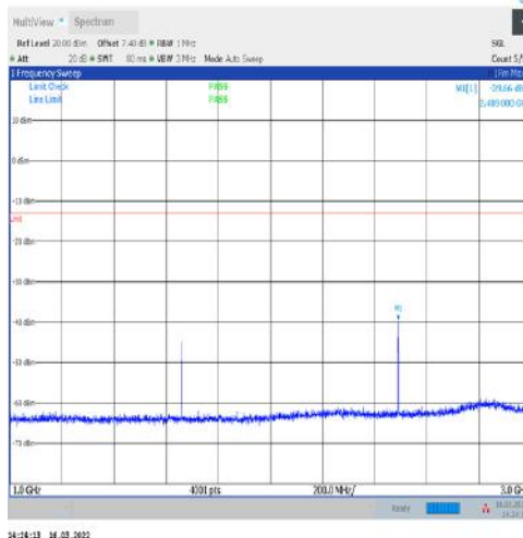
1-N5-15-20-H-1-DFT-PI2BPSK-Inner_1RB_Left- 1@1-1000-3000-Ant1--39.66--13-PASS
