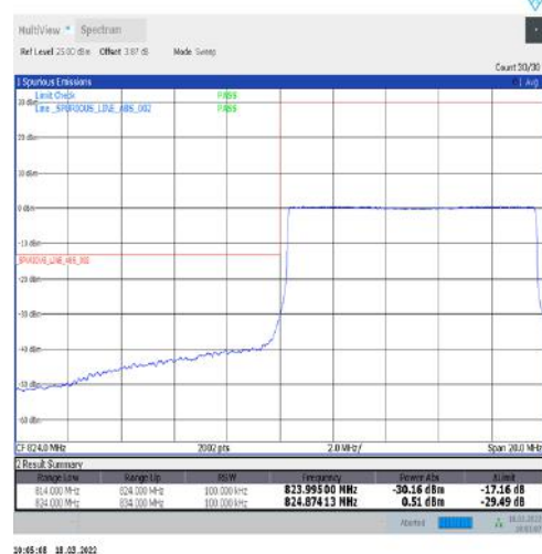
1-N5-15-10-L-6-CP-QPSK-Outer_Full-52@0-Ant1-seegraph-PASS-see graph
