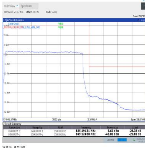
1-N5-15-15-H-3-DFT-PI2BPSK-Outer_Full-75@0-Ant1-seegraph-PASS-see graph
