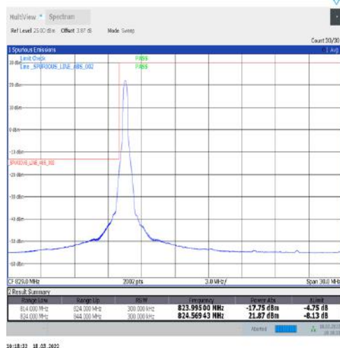
1-N5-15-20-L-1-DFT-PI2BPSK-Edge_1RB_Left-1@0-Ant1-seegraph-PASS-see graph
