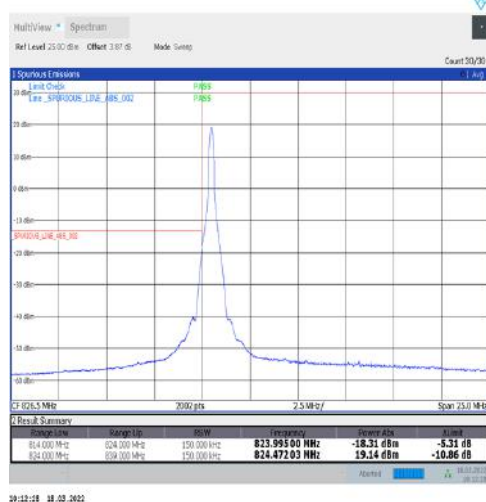
1-N5-15-15-L-4-CP-QPSK-Edge_1RB_Left-1@0-Ant1-seegraph-PASS-see graph
