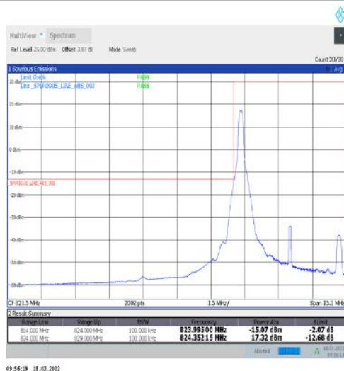
1-N5-15-5-L-4-CP-QPSK-Edge_1RB_Left-1@0-Ant1-seegraph-PASS-see graph
