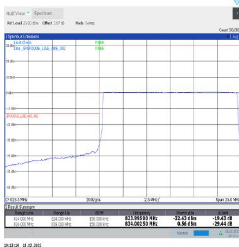
1-N5-15-15-L-6-CP-QPSK-Outer_Full-79@0-Ant1-seegraph-PASS-see graph
