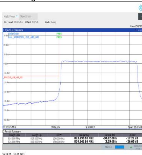
1-N5-15-15-L-3-DFT-PI2BPSK-Outer_Full-75@0-Ant1-seegraph-PASS-see graph
