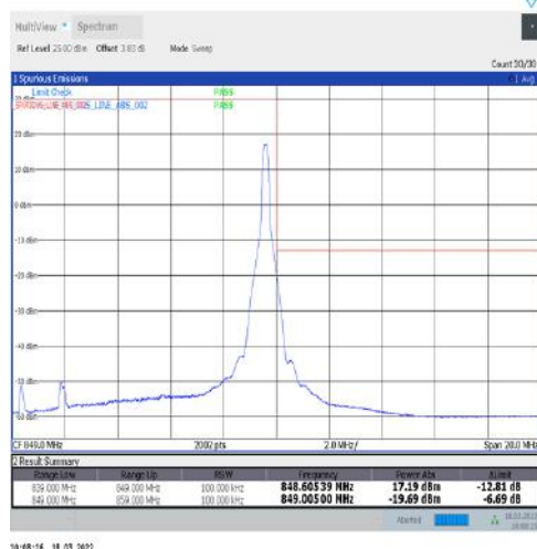
1-N5-15-10-H-5-CP-QPSK-Edge_1RB_Right-1@51-Ant1-seegraph-PASS-see graph
