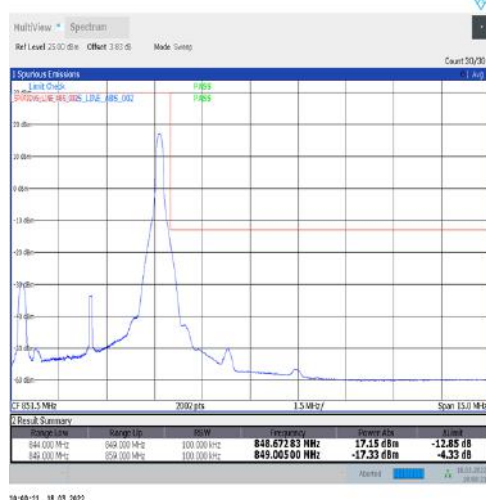
1-N5-15-5-H-5-CP-QPSK-Edge_1RB_Right-1@24-Ant1-seegraph-PASS-see graph
