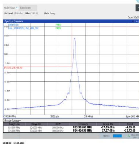
1-N5-15-10-L-4-CP-QPSK-Edge_1RB_Left-1@0-Ant1-seegraph-PASS-see graph
