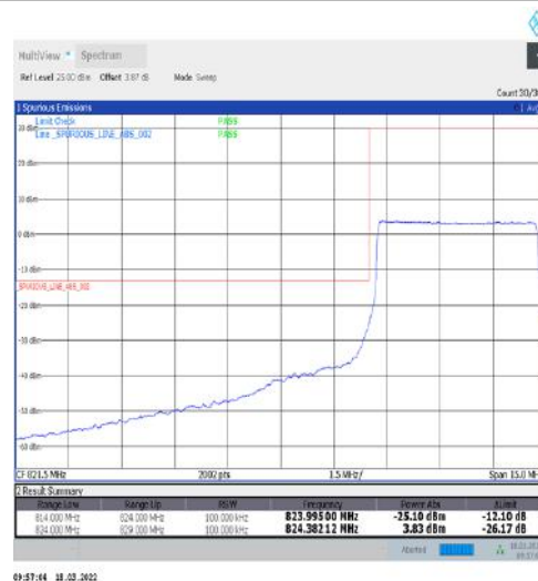
1-N5-15-5-L-6-CP-QPSK-Outer_Full-25@0-Ant1-seegraph-PASS-see graph
