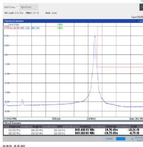
1-N5-15-20-H-5-CP-QPSK-Edge_1RB_Right-1@105-Ant1-seegraph-PASS-see graph
