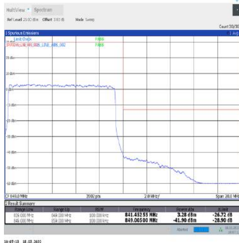
1-N5-15-10-H-3-DFT-PI2BPSK-Outer_Full-50@0-Ant1-seegraph-PASS-see graph
