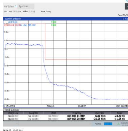
1-N5-15-5-H-3-DFT-PI2BPSK-Outer_Full-25@0-Ant1-seegraph-PASS-see graph
