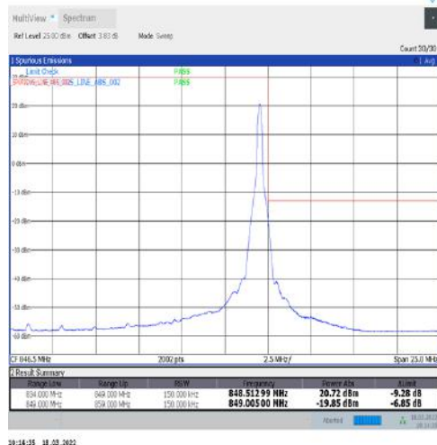
1-N5-15-15-H-2-DFT-PI2BPSK-Edge_1RB_Right-1@78-Ant1-seegraph-PASS-see graph
