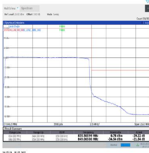
1-N5-15-15-H-6-CP-QPSK-Outer_Full-79@0-Ant1-seegraph-PASS-see graph
