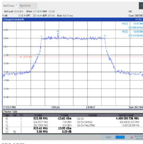
1-N5-15-5-L-1-DFT-QPSK-Outer_Full-25@0-Ant1- 4.486-5.060-≤5-PASS
