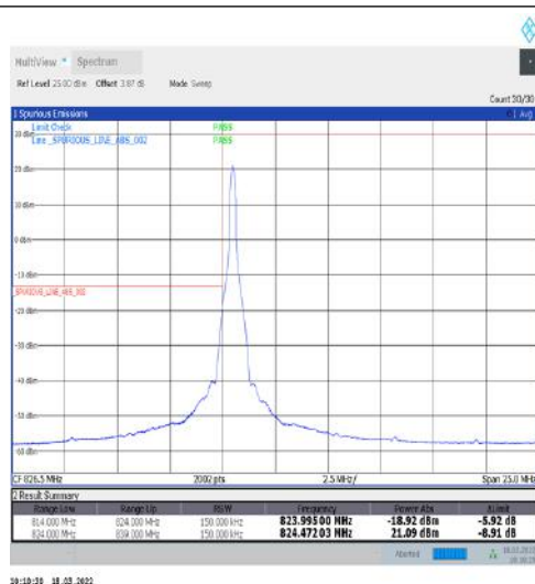
1-N5-15-15-L-1-DFT-PI2BPSK-Edge_1RB_Left-1@0-Ant1-seegraph-PASS-see graph
