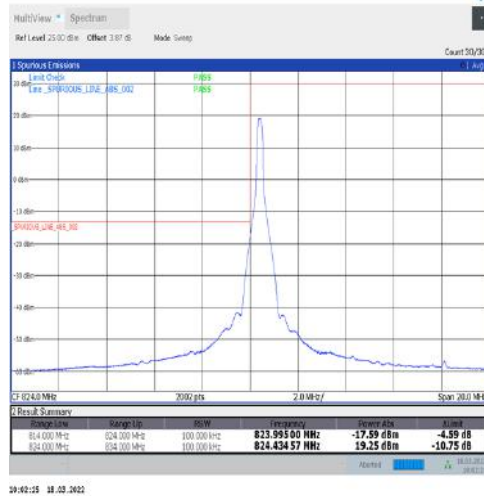
1-N5-15-10-L-1-DFT-PI2BPSK-Edge_1RB_Left-1@0-Ant1-seegraph-PASS-see graph
