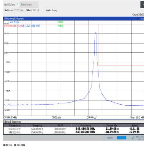
1-N5-15-20-H-2-DFT-PI2BPSK-Edge_1RB_Right-1@105-Ant1-seegraph-PASS-see graph
