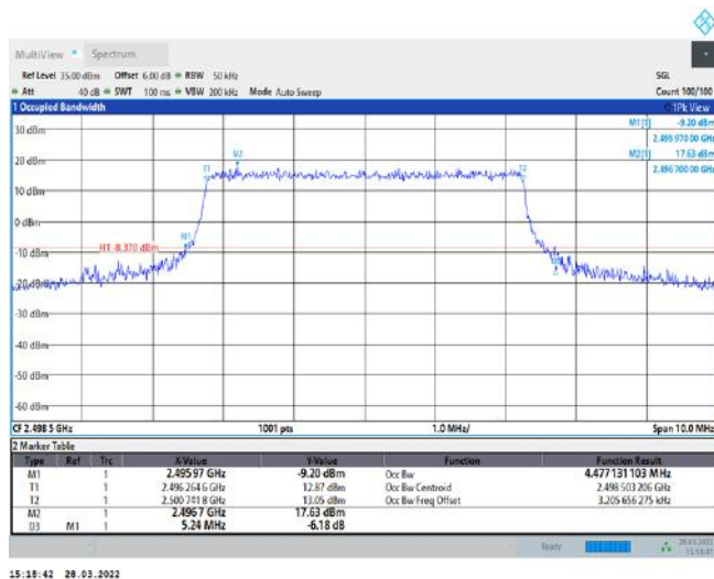
Band41-5MHz-QPSK-40620-25RB#0
