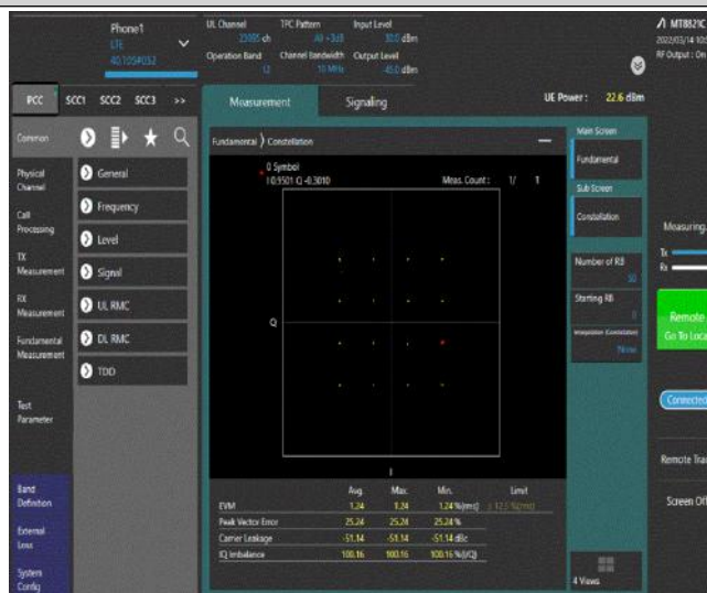
Band12-10MHz-16QAM-23095-50RB#0
